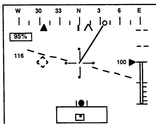
Figure 2-6. The Transition mode used to fly a straight path in a cross-wind.
