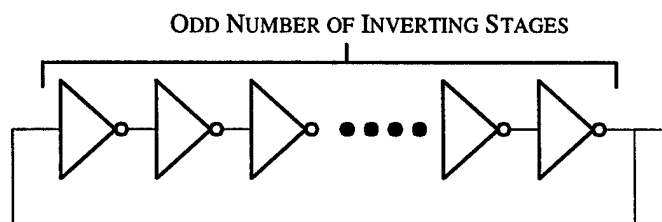
Figure 2.22 Basic ring oscillator block diagram.
