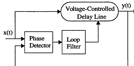
Figure 2.9 Basic DLL topology.
