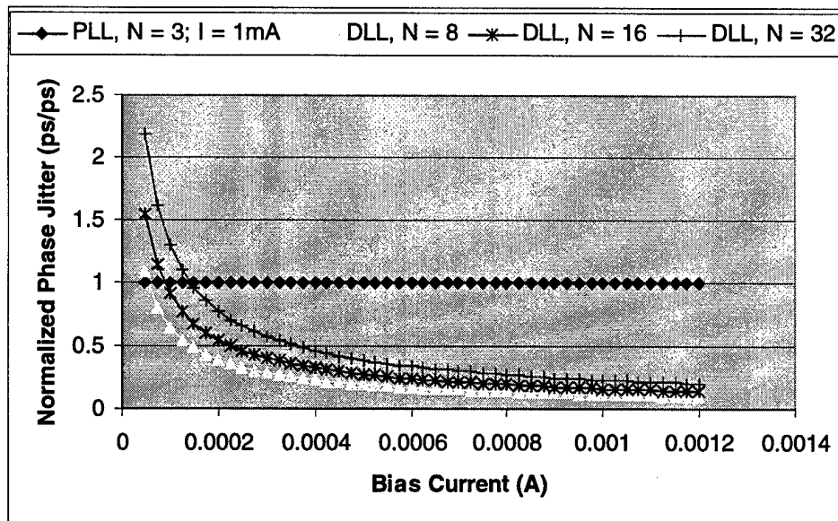
Figure 6.8 Normalized phase jitter of the DLL in comparison to the PLL.
