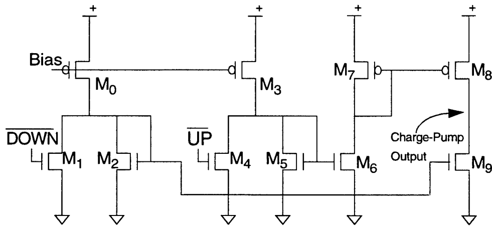
Figure 5.9 CSA charge pump schematic.
