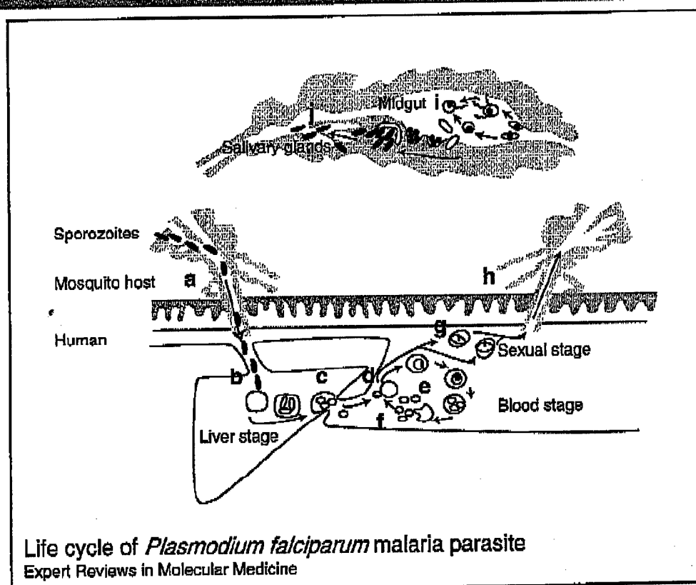
Figure 1. The life cycle of Plasmodium falciparum malaria parasite. Malaria is caused by infection with an obligate, intracellular protozoan parasite of the genus Plasmodium . Of the four species that infect humans ( Plasmodium falciparum , Plasmodium vivax , Plasmodium ovale and Plasmodium malariae ), it is P. falciparum that is responsible for virtually all deaths. The life cycle of Plasmodium spp. is complex and somewhat specific to the parasite species. (a) P. falciparum infection in humans begins when an infected Anopheles sp. mosquito takes a blood meal and injects infective sporozoites into the peripheral circulation. (b) Within minutes, these sporozoites invade hepatocytes in the liver and, over approximately one week, undergo asexual multiplication, producing tens of thousands of merozoite forms of the parasite. (c) When the infected hepatocyte ruptures, merozoites are released into the peripheral circulation. (d) The merozoites invade red blood cells (rbc) and (e) complete another round of multiplication within 48–72 h, with the production of 16–20 additional merozoites per rbc, which devour the rbc haemoglobin in the process. (f) The released merozoites invade hepatocytes and carry on the cycle. It is the synchronous release of merozoites that is thought to be responsible for the periodic fevers associated with malaria. (g) Some invading merozoites do not divide, but differentiate into male (microgametocyte) and female (macrogametocyte) sexual forms. (h) These sexual forms are taken from the bloodstream by a feeding Anopheles sp. mosquito and (i) fertilise in the mosquito midgut to form zygotes. These zygotes further differentiate into motile forms, called ookinets, migrate through the mosquito gut wall and divide within oocysts on the external gut wall to form thousands of sporozoites. (j) The infective sporozoites are released into the mosquito haemocoel and move to the salivary gland, where they await injection into another human host, thus completing the life cycle (fig001dcn).
