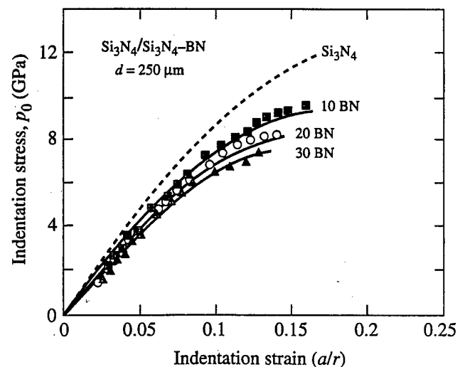
Fig. 5. Indentation stress–strain curves for \text{Si}_3\text{N}_4/\text{Si}_3\text{N}_4 -BN bilayer composites, \text{Si}_3\text{N}_4 coating thickness d = 250 \mu\text{m} , showing effect of BN content in substrate. Solid curves are FEM predictions, using material parameters calibrated from Fig. 3. Upper dashed curve is bound for \text{Si}_3\text{N}_4 from Fig. 3.
