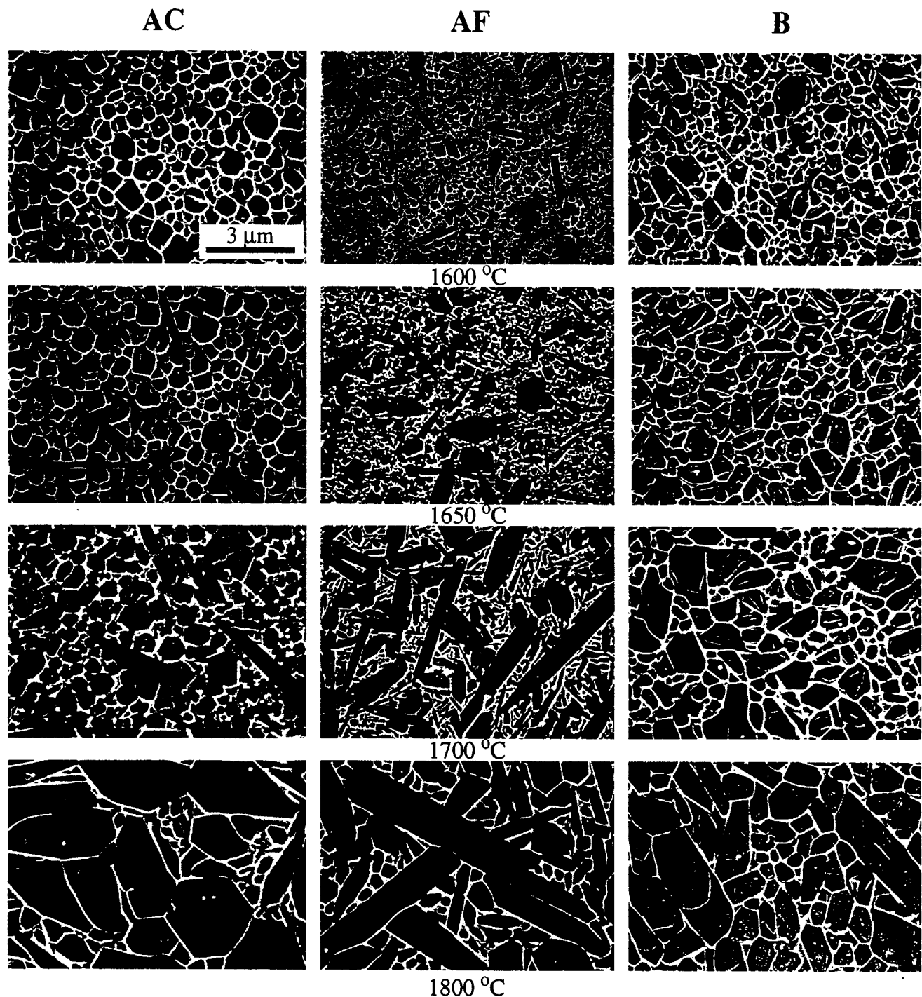
Fig. 1. SEM micrographs of Si 3 N 4 polished surfaces, fired at 1600°, 1650°, 1700°, and 1800°C for 1 h. Specimen designation as follows: AC (E3 powder, \alpha phase, coarse); AF (E10 powder, \alpha phase, fine); B (KSN-80SP powder, \beta phase). Specimens plasma etched in CF 4 and O 2 gas for 10 min to reveal grain structures.
