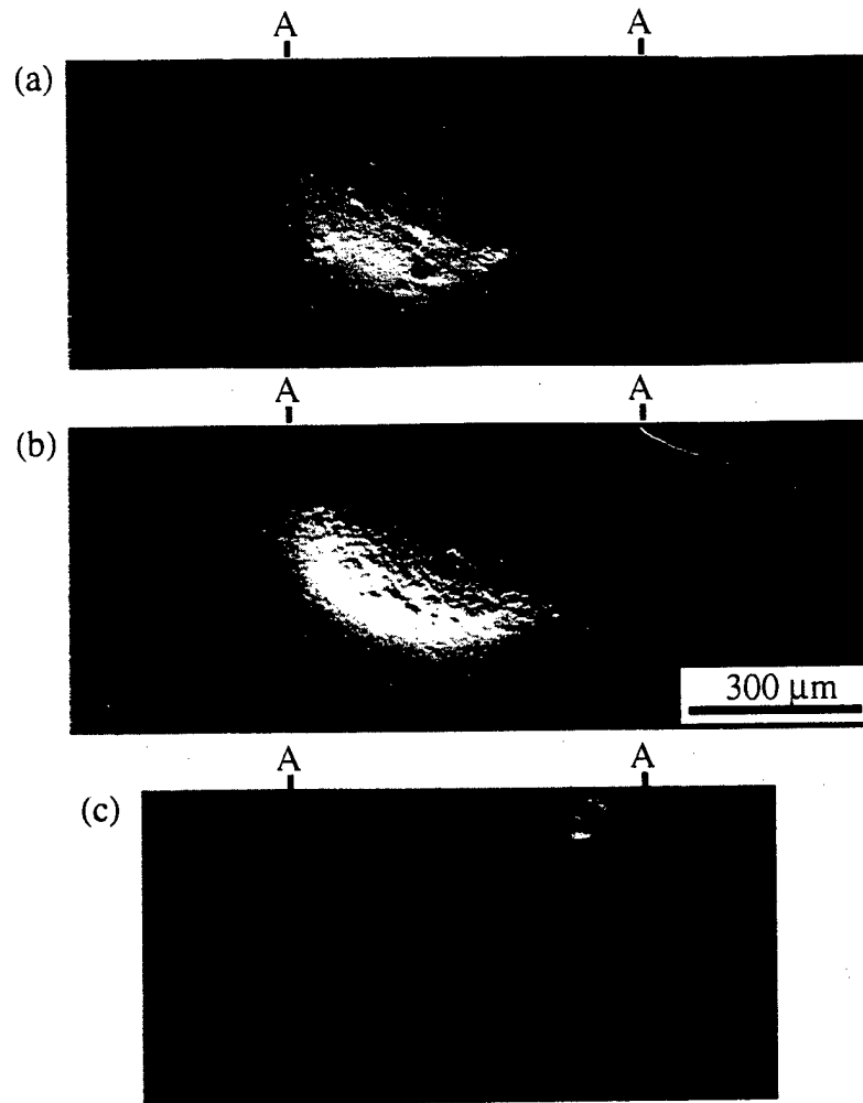
Fig. 8. Side views of Hertzian contact damage in B \text{Si}_3\text{N}_4 , fired at (a) 1650^\circ\text{C} , (b) 1700^\circ\text{C} , and (c) 1800^\circ\text{C} . Indentations made using WC sphere radius r = 1.98 mm at load P = 4000 N. AA denotes contact diameter. Nomarski optical micrographs of bonded-interface specimens.
