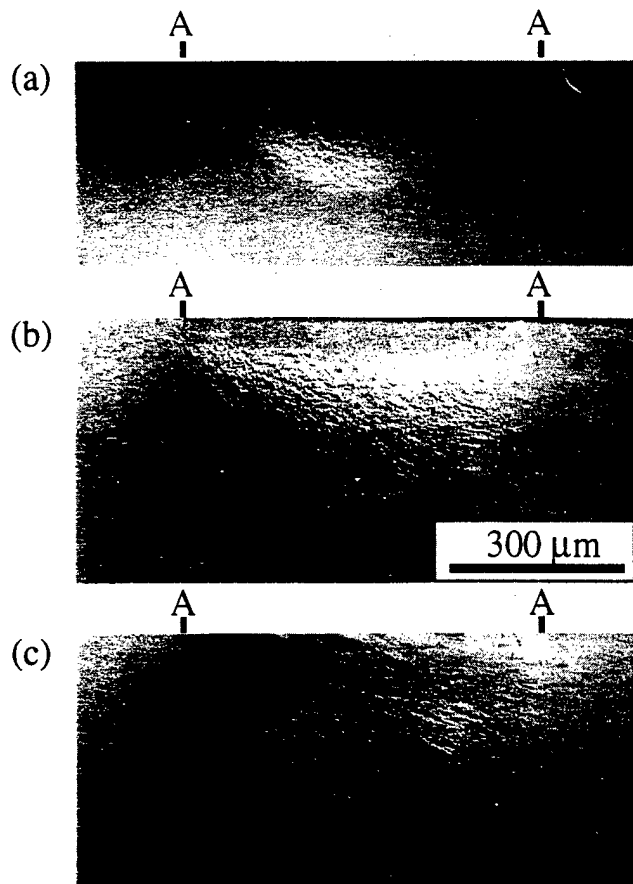
Fig. 7. Side views of Hertzian contact damage in AF \text{Si}_3\text{N}_4 , fired at (a) 1650°, (b) 1700°, and (c) 1800°C. Indentations made using WC sphere radius r = 1.98 mm at load P = 4000 N. AA denotes contact diameter. Nomarski optical micrographs of bonded-interface specimens.
