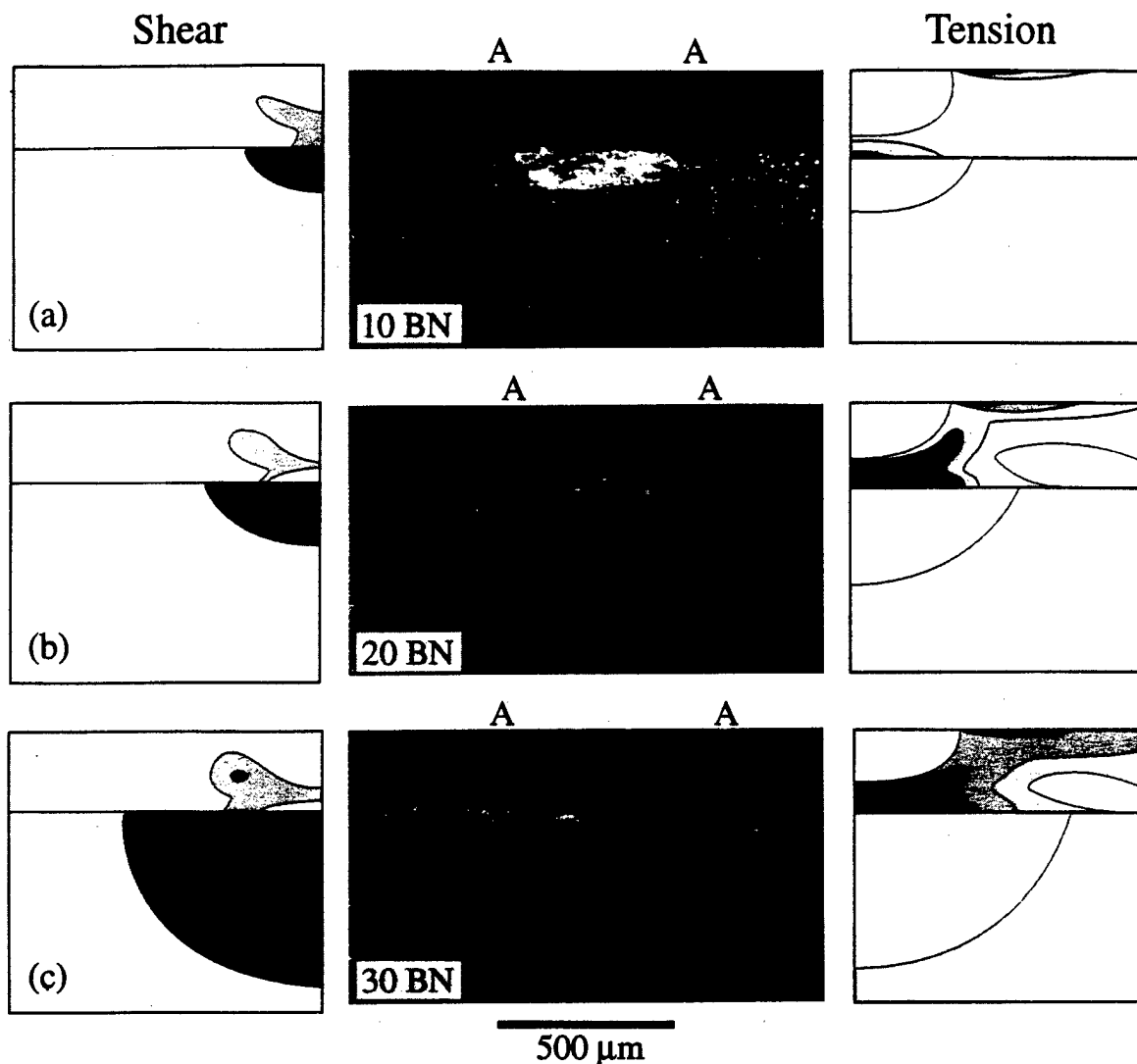
Fig. 8. Contact fracture in \text{Si}_3\text{N}_4/\text{Si}_3\text{N}_4 -BN bilayer composites, \text{Si}_3\text{N}_4 coating thickness d = 250 \mu\text{m} , using WC sphere r = 1.98 \text{ mm} at P = 2000 \text{ N} , illustrating effect of substrate composition: (a) 10 wt% BN, (b) 20 wt% BN, (c) 30 wt% BN. Note increased damage at higher BN contents.
