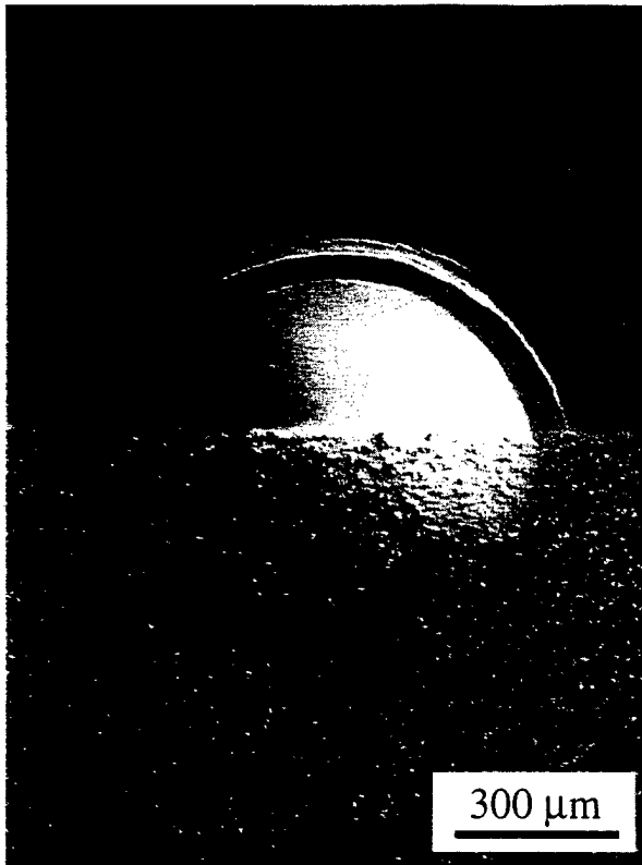
Fig. 2. Hertzian indentations in \text{Si}_3\text{N}_4/\text{Si}_3\text{N}_4 -10 wt% BN bilayer, made symmetrically across interface trace, with WC sphere r = 1.98 mm at P = 2000 N. Note crack penetration from \text{Si}_3\text{N}_4 side to \text{Si}_3\text{N}_4 -BN side, without delamination.
