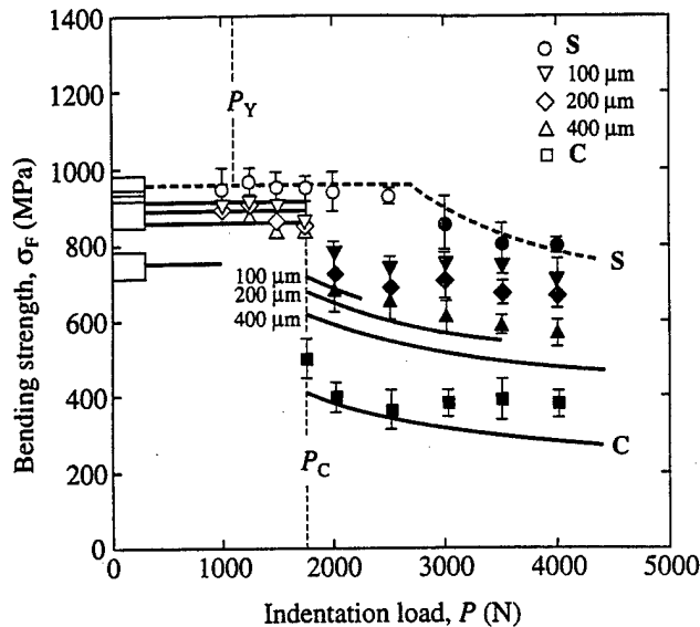
Fig. 13. Strength degradation of C/S \text{Si}_3\text{N}_4 bilayers, plus C and S monoliths, for contacts with WC sphere radius r = 1.98 mm. Data plotted as a function of indentation load P , for coating thicknesses indicated. Open symbols indicate breaks away from indentation sites, gray symbols failures from quasi-plastic zones, black symbols failures from cone cracks. Boxes at left axis denote strengths of unindented specimens. Vertical dashed lines indicate values of P_Y for S, P_C for C. Solid curves are theoretical predictions assuming failure from cone cracks at P > P_C and from microstructural flaws at P < P_C , for C monoliths (lowest curve) and C/S bilayers at 400, 200, and 100 \mu\text{m} (upper three curves, truncated at loads and coating thicknesses where cones penetrate into substrate). Dashed curve is empirical fit to S data. 18
