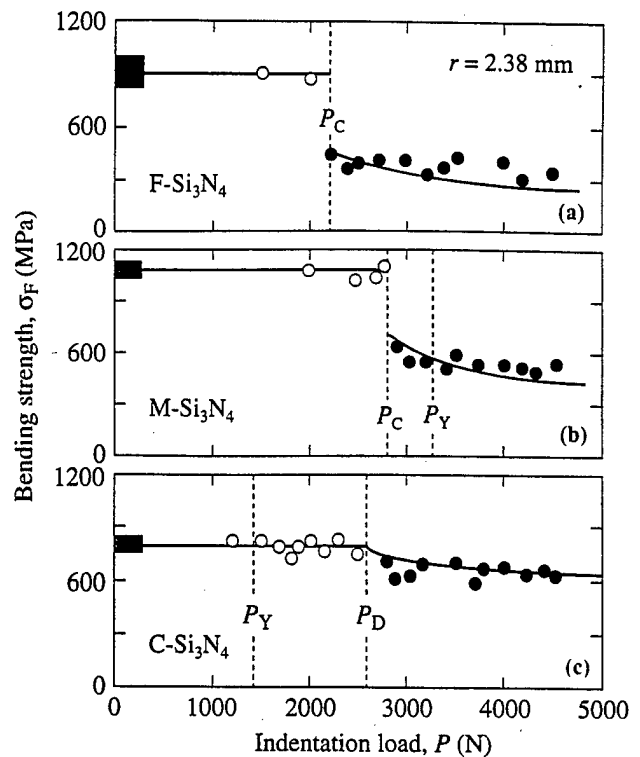
Fig. 2. Inert strength of Hertzian-indented \text{Si}_3\text{N}_4 specimens indented with WC sphere, r = 2.38 mm, as function of indentation load, illustrating effect of microstructure: (a) F\text{-Si}_3\text{N}_4 , (b) M\text{-Si}_3\text{N}_4 , (c) C\text{-Si}_3\text{N}_4 . Data points are experimental measurements, indentation tests in air: closed symbols represent failures from indentation origins, open symbols from other origins. Shaded box at left axis represents strengths of polished, unindented specimens. Vertical dashed lines indicate critical loads P_C , P_Y , and P_D .
