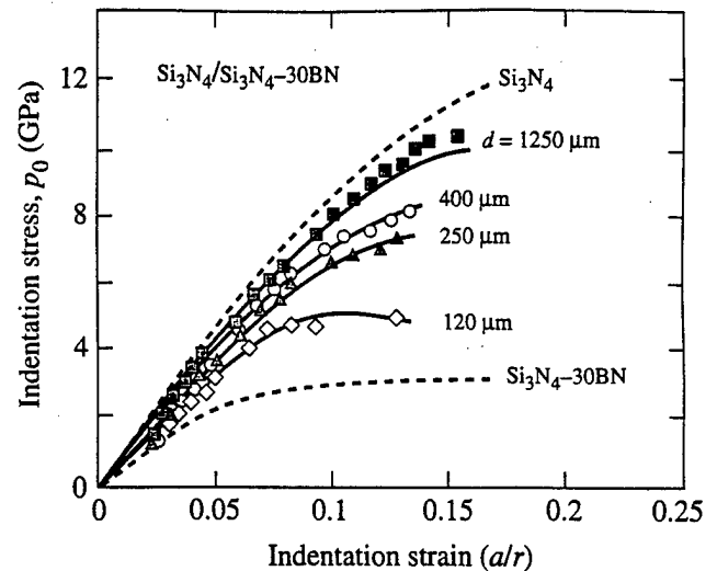
Fig. 4. Indentation stress–strain curves for \text{Si}_3\text{N}_4/\text{Si}_3\text{N}_4 -30 wt% BN bilayer composites, for \text{Si}_3\text{N}_4 coating thicknesses d indicated. Solid curves are FEM predictions, using material parameters calibrated from Fig. 3. Upper and lower dashed curves are bounds for \text{Si}_3\text{N}_4 and \text{Si}_3\text{N}_4 -30 wt% BN component materials, respectively, from Fig. 3.
