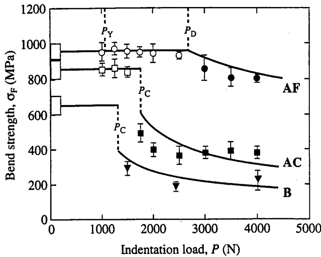
Fig. 11. Strength degradation for AC, AF, and B \text{Si}_3\text{N}_4 materials fired at 1700^\circ\text{C} , for contacts with WC sphere, r = 1.98 mm. Open symbols indicate failures away from indentation sites, gray symbols failures from quasi-plastic zones, black symbols failures from ring cracks. Points with error bars represent means and standard deviations of a minimum of five specimens; points without error bars are individual breaks. Boxes at left axis denote natural strengths (unindented specimens). Vertical dashed lines indicate critical loads for strength-degrading damage (see Fig. 9).
