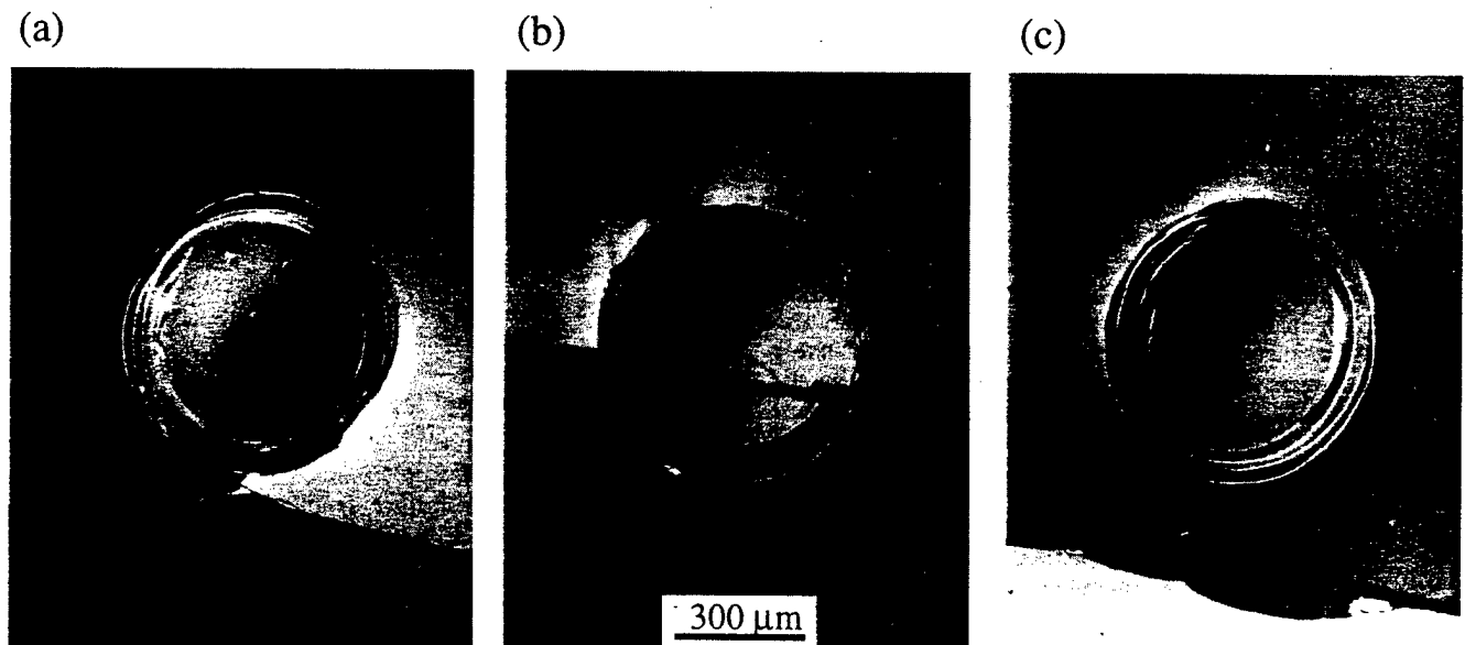
Fig. 10. Micrographs showing failure of (a) AC, (b) AF, and (c) B Si 3 N 4 materials fired at 1700°C, from strength specimens containing indentations made with WC sphere, r = 1.98 mm, P = 4000 N. Nomarski illumination, surface gold coated. Tensile direction vertical in plane of diagram.
