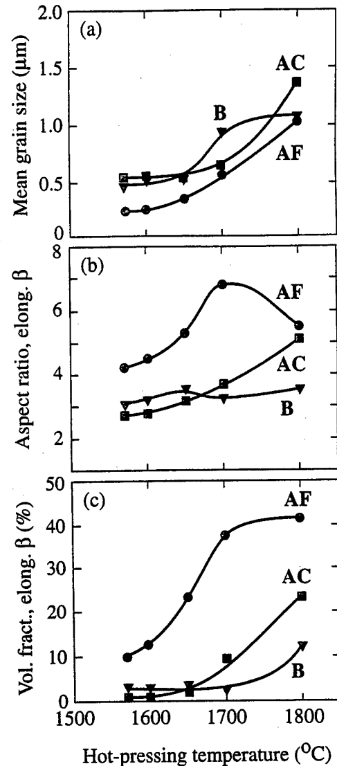
Fig. 3. Microstructural characterization of AC, AF, and B \text{Si}_3\text{N}_4 materials as function of hot-pressing temperature: (a) mean grain size, (b) aspect ratio of largest 10% elongate \beta grains, (c) volume fraction of elongate \beta grains with aspect ratio > 3 .
