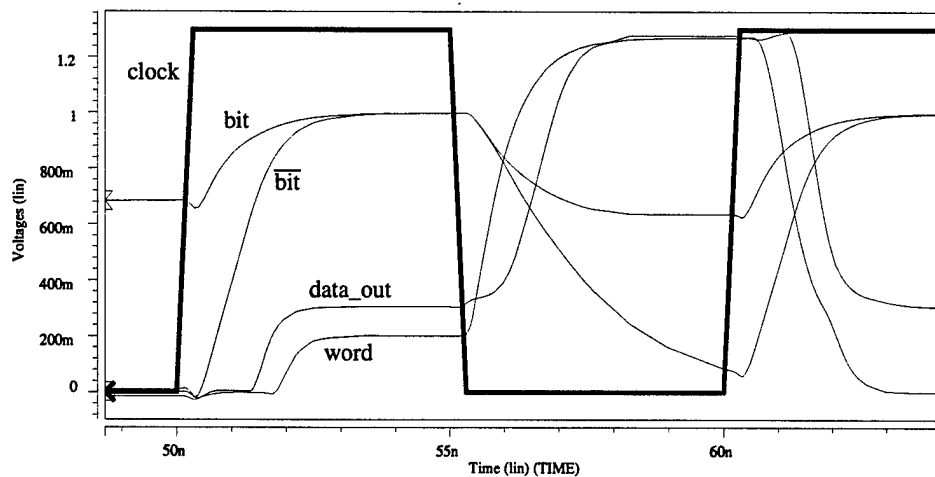
Fig. 3.11 CGaAs synchronous RAM cycle SPICE simulation.
