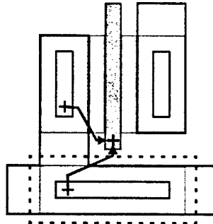
Fig. A.2. A pair of geometry constraints.
