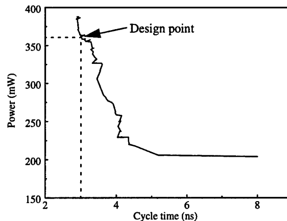
Fig. 3.40 2 k-byte RAM near-optimal power delay curve.
