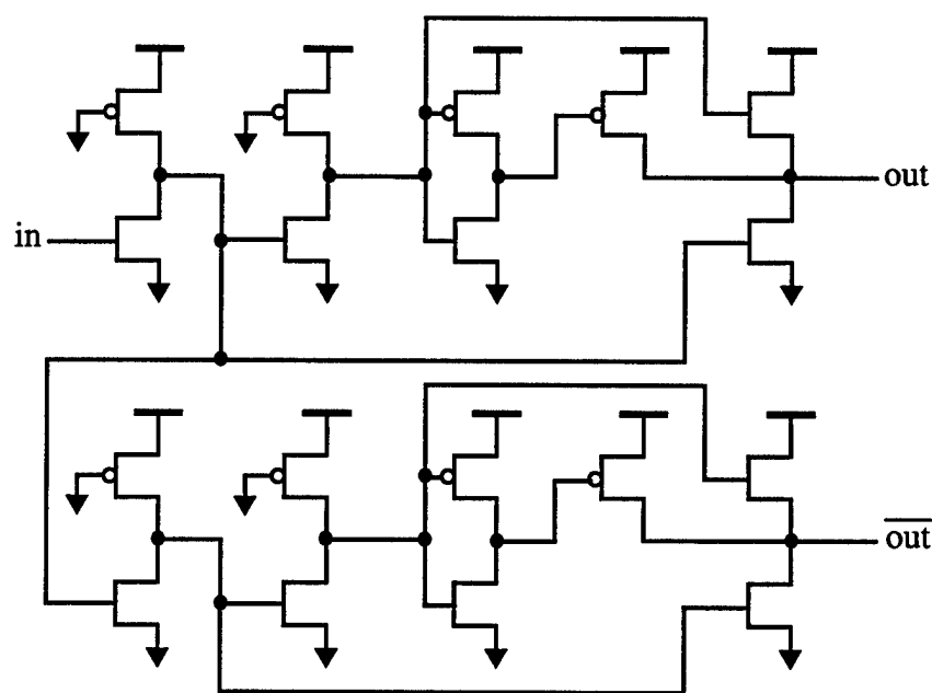
Fig. 3.10 Address and write enable superbuffer circuitry.
