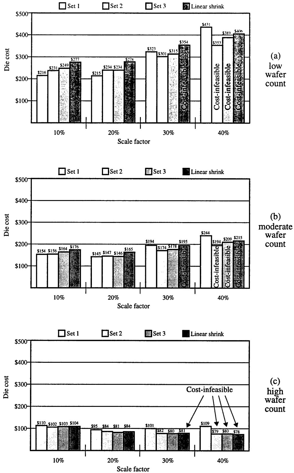
Fig. 4.7 CGaAs die cost estimates.
