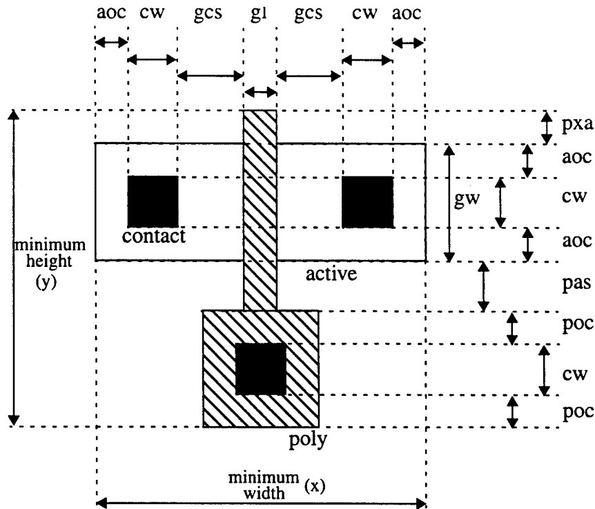
Fig. 2.5 Area-critical design rules for a single transistor.
