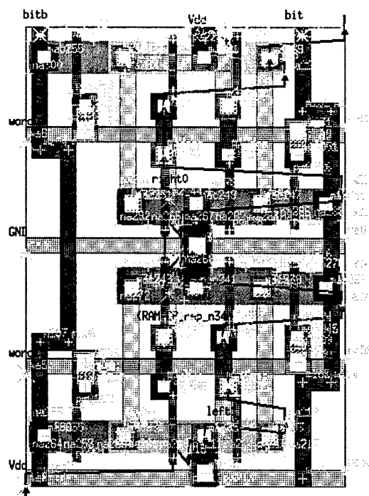
Fig. 4.2 MasterPort's area-critical path analysis of a 6T cell pair.
