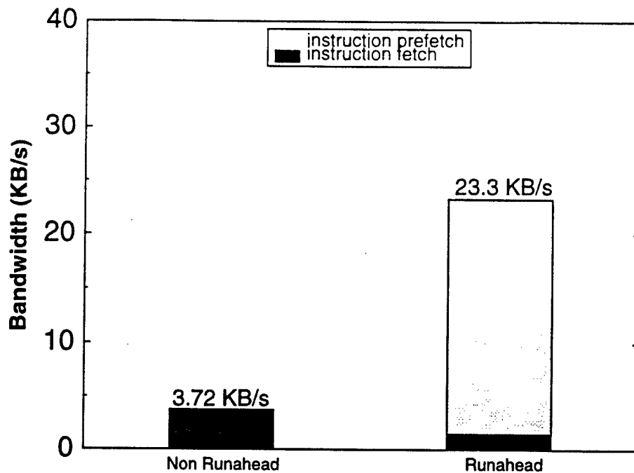
Average L2 Instruction Cache Bandwidth for STREAM
