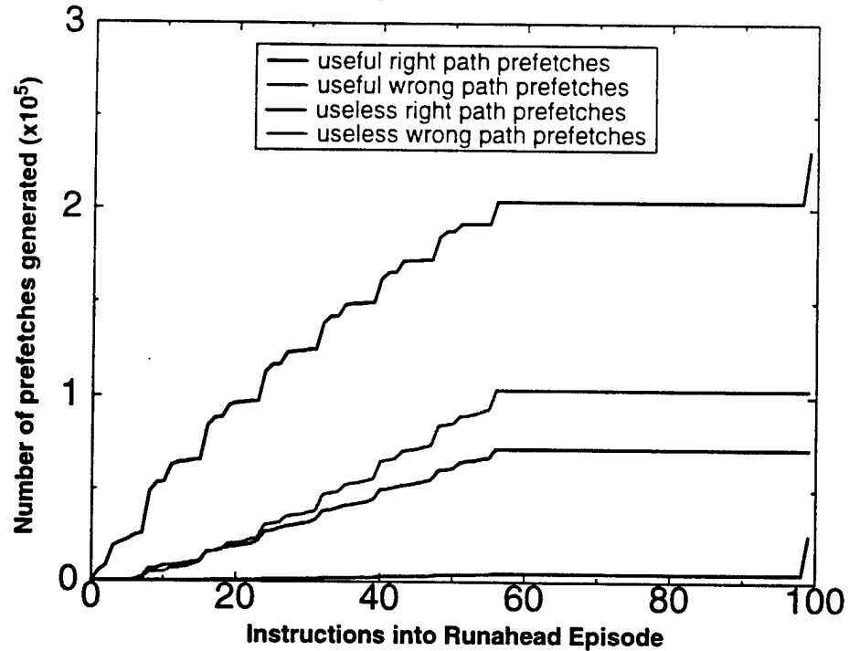
Instruction Stream Prefetch Utility for IJpeg INSTRUCTION prefetches during INSTRUCTION miss initiated runahead
