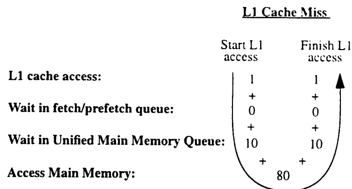
Figure 3.6 Minimum L1 data cache miss timing for processors without L2 data cache
