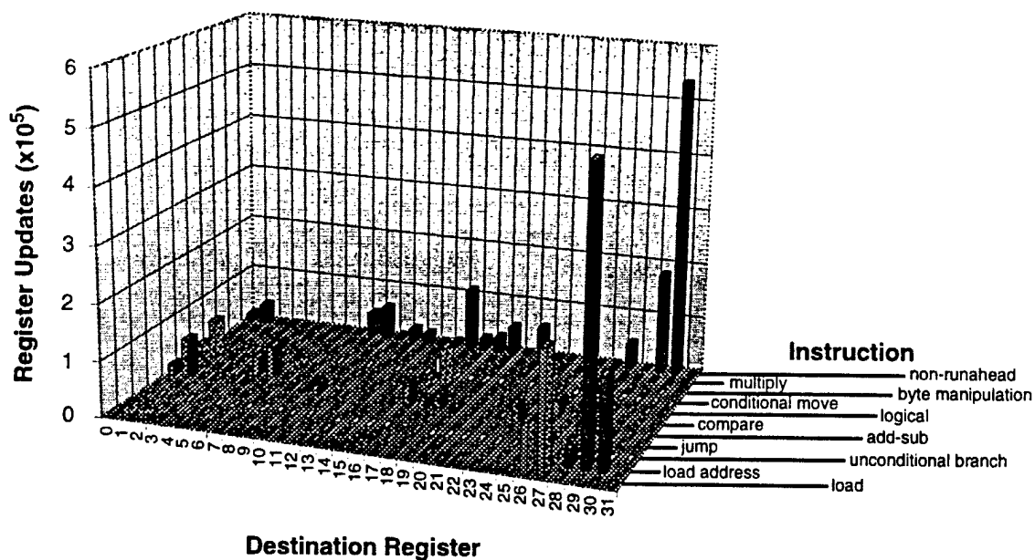
Figure 5.17 Source of Prefetch Addresses for PERL
