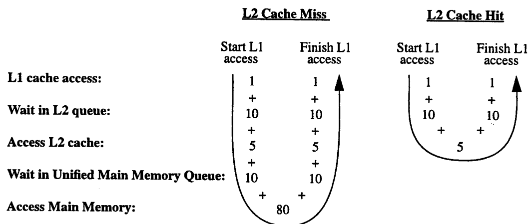
Figure 3.5 Minimum L2 cache access timing
