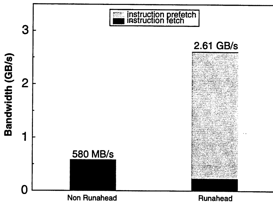
Average L2 Instruction Cache Bandwidth for PERL
