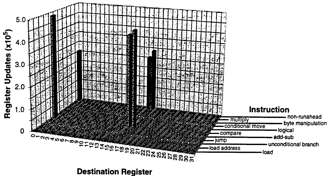
Figure 5.19 Source of Data Stream Prefetch Addresses for STREAM
