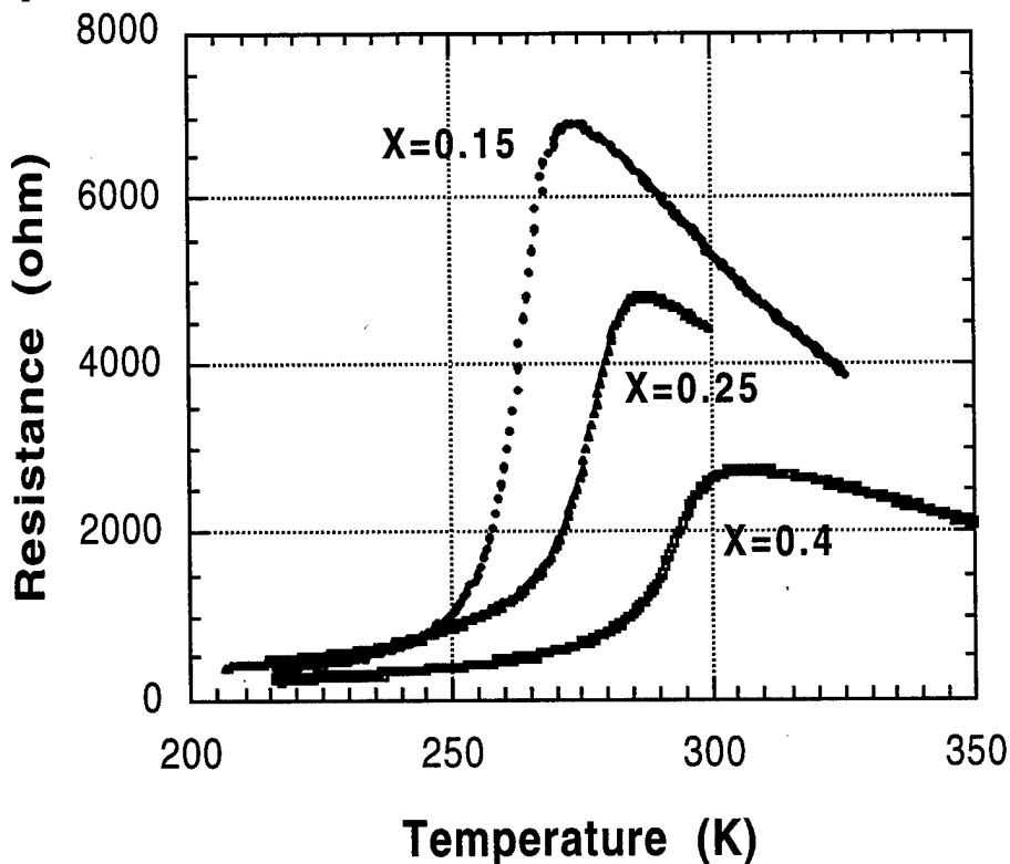
Figure 3: Variation of transition, TCR, and resistance with stoichiometry of La_xCa_{1-x}MnO_3 film
