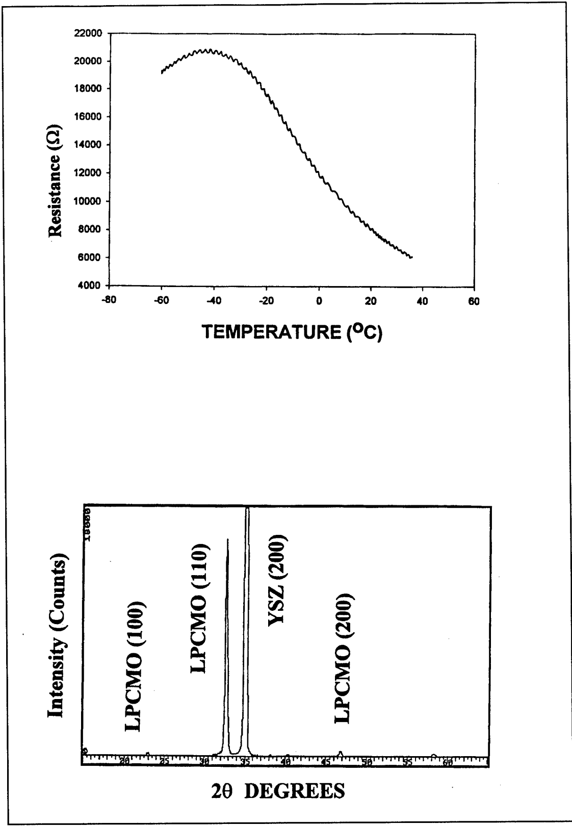
Figure 7: The \Theta - 2\Theta diffraction pattern and R vs T curves measured for LPCMO deposited directly on (100) YSZ single crystal.
