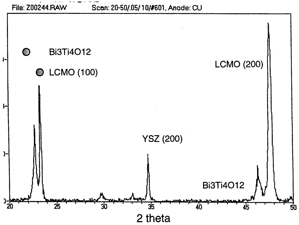
Figure 17: Growth of \text{LCMO}/\text{Bi}_3\text{Ti}_4\text{O}_{12}/\text{YSZ} on \text{Si}_3\text{N}_4 coated Si.
