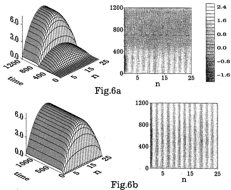
Fig.6. Transient control. Linear array of 25 slab lasers ( a / \sigma = 4 ) in a Talbot cavity. Gain-variation ( t=1..700: g=0.05 , t=700...1200: g=0.4 ) -fig. 6a. Invariable gain ( t=1..1200: g=0.4 ) -fig. 6b.
