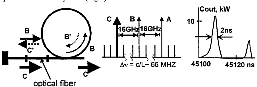
Fig.4. Stage III. Second Stokes SBS generation in the cavity fiber.
