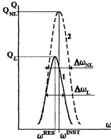
Fig. 5. Laser-induced variation of Q -factor spectrum of passive microresonator which can accompany developing of field instability. 1 - spectrum of Q -factor for linear resonant case; 2 - that for nonlinear case. There are shown variation of resonant frequency and broadening of Q -factor spectral line for linear (L) and nonlinear (NL) optical response. \omega^{RES} is resonant frequency for linear passive resonator, \omega^{INST} is generation frequency at which field instability develops.
