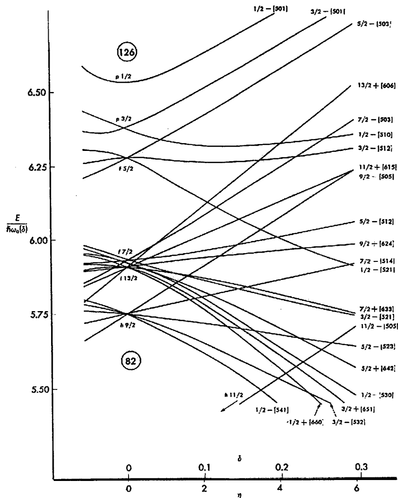
Figure 2: State levels for protons in region between 82 and 126 magic numbers. After Mottelson and Nielson.
