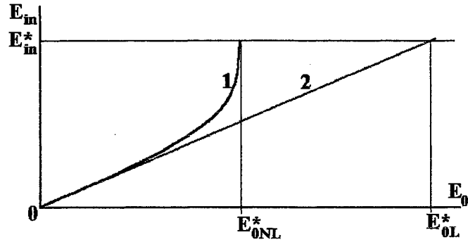
Figure 3. Typical dependence of field amplitude inside microcavity E_{in} on pump field E_0 for nonlinear (curve 1) and linear (curve 2) cases.
