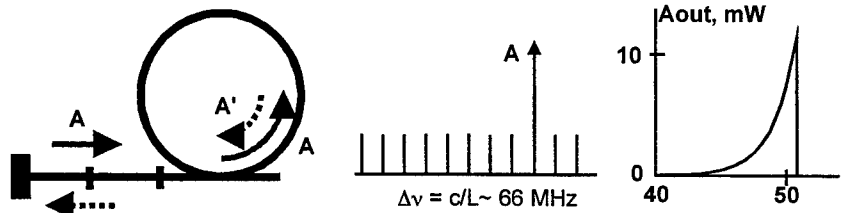
Fig.2. Stage I. Initial lasing caused by Rayleigh backscattering in the ring.
