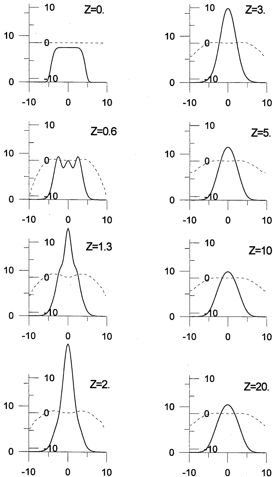
Fig.1 Formation of stable state of symmetric laser bullet. Consequent profiles of light intensity (1) and phase (2) for laser bullet in process of its formation. Initial spot of light with radial symmetry is narrowing and approaching to stationary distribution.
