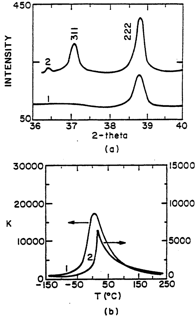
FIGURE 2 As-Fired [1] and Annealed [2] \text{Pb}(\text{Sc}_{1/2}\text{Ta}_{1/2})\text{O}_3 ceramics. (a) The 311/222 x-ray diffraction pair and (b) the dielectric constant as a function of temperature at 1 KHz.
