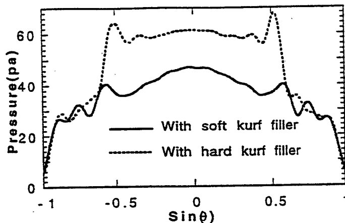
Fig.13 The directivity pattern (acceptance angle) of an array element with soft and hard kerf filler
