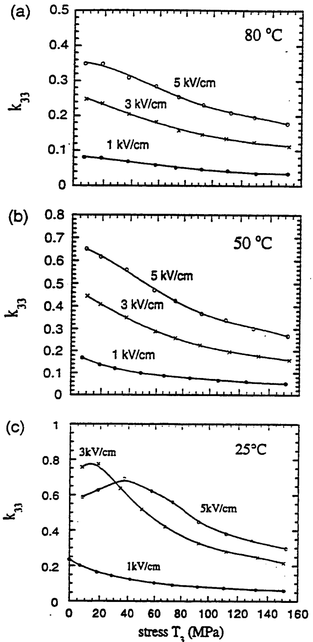
FIG. 12. The electromechanical coupling factor k_{33} (calculated at 10 Hz) as a function of the compressive T_3 at different temperatures: (a) 80 °C, (b) 50 °C, and (c) 25 °C; and dc electric bias fields: 1 kV/cm ( \bullet ), 3 kV/cm ( \times ), and 5 kV/cm ( \circ ).
