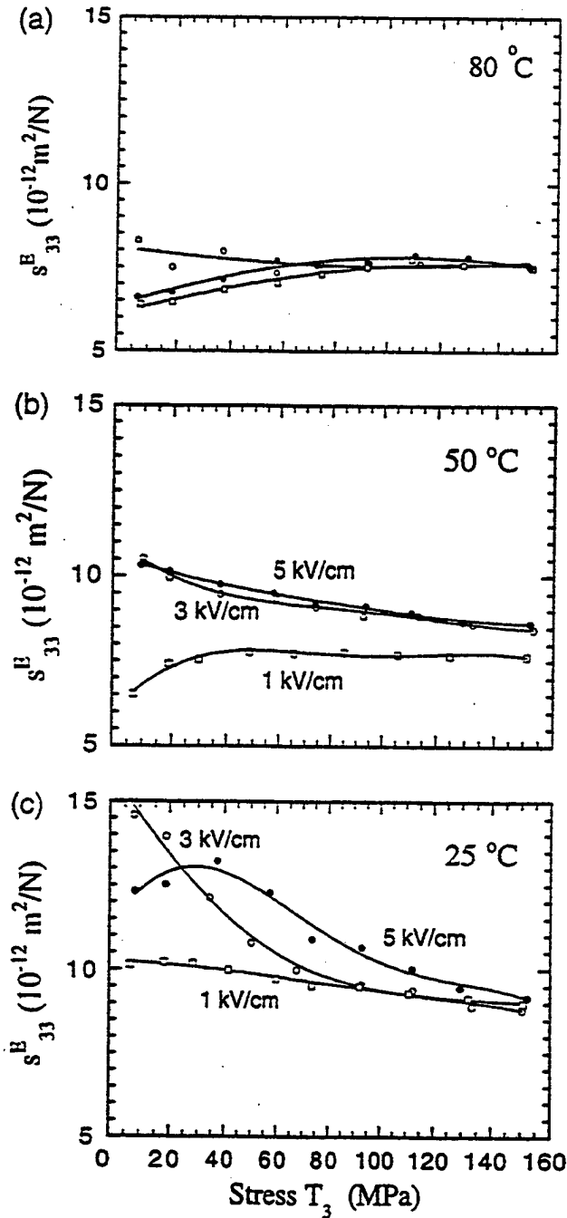
FIG. 6. The elastic compliance s_{33}^E as a function of the compressive T_3 at different temperatures: (a) 80 °C, (b) 50 °C, and (c) 25 °C; and dc electric bias fields: 1 kV/cm ( \square ), 3 kV/cm ( \circ ), and 5 kV/cm ( \bullet ).
