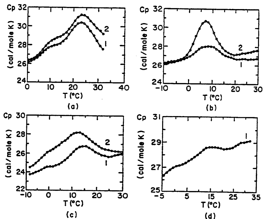
FIGURE 8 The specific heat, C_p(T) , of As-Fired [1] and Annealed [2] (1-x)\text{Pb}(\text{Sc}_{1/2}\text{Ta}_{1/2})\text{O}_3-x\text{PbTiO}_3 ceramics: (a) x=0.0 , (b) x=0.05 , (c) x=0.075 , (d) x=0.1 .
