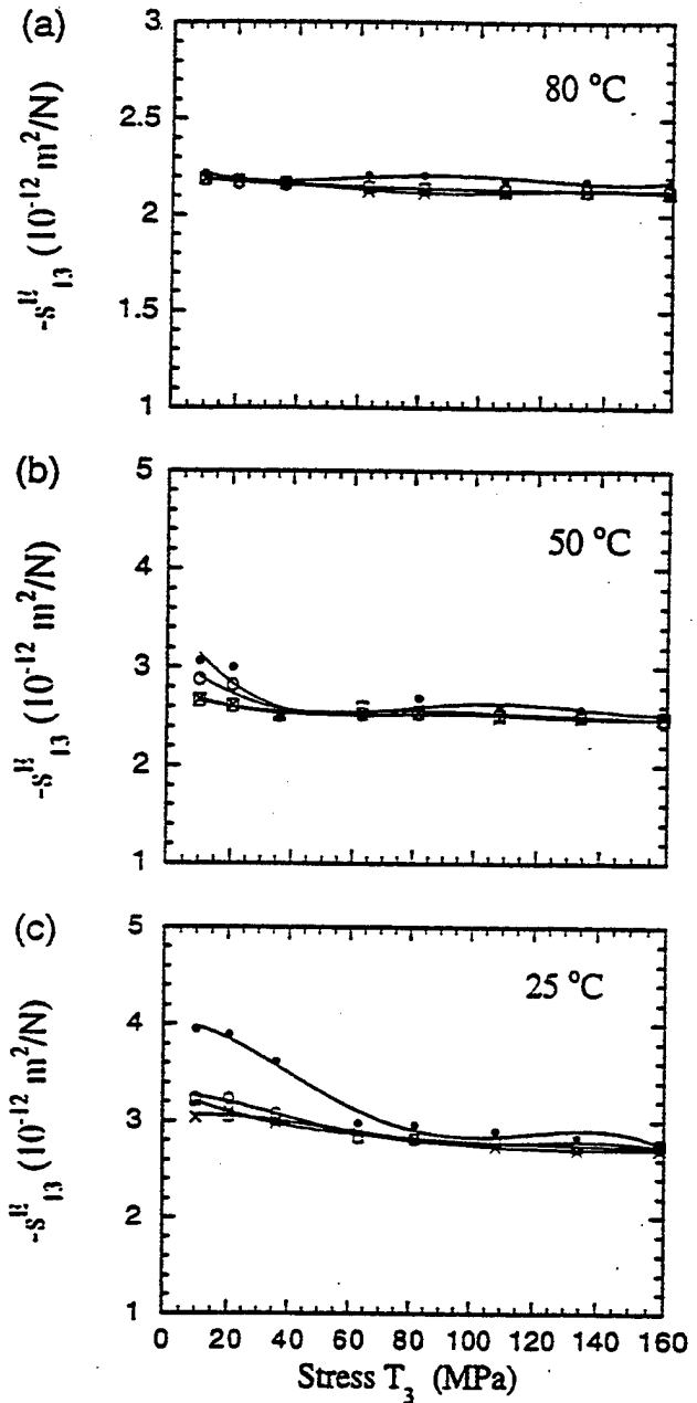
FIG. 7. The elastic compliance s_{13}^E as a function of the compressive T_3 at different temperatures: (a) 80 °C, (b) 50 °C, and (c) 25 °C, and dc electric bias fields: zero bias ( \times ), 1 kV/cm ( \square ), 3 kV/cm ( \circ ), and 5 kV/cm ( \bullet ).
