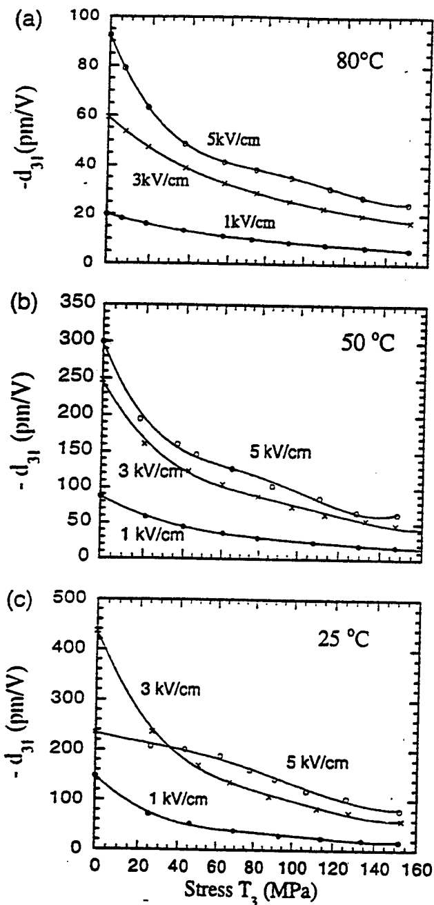
FIG. 9. The effective piezoelectric coefficient d_{31} at the dc field-biased states as a function of the compressive T_3 at different temperatures: (a) 80 °C, (b) 50 °C, and (c) 25 °C; and dc electric bias fields: 1 kV/cm ( \bullet ), 3 kV/cm ( \times ), and 5 kV/cm ( \circ ).
