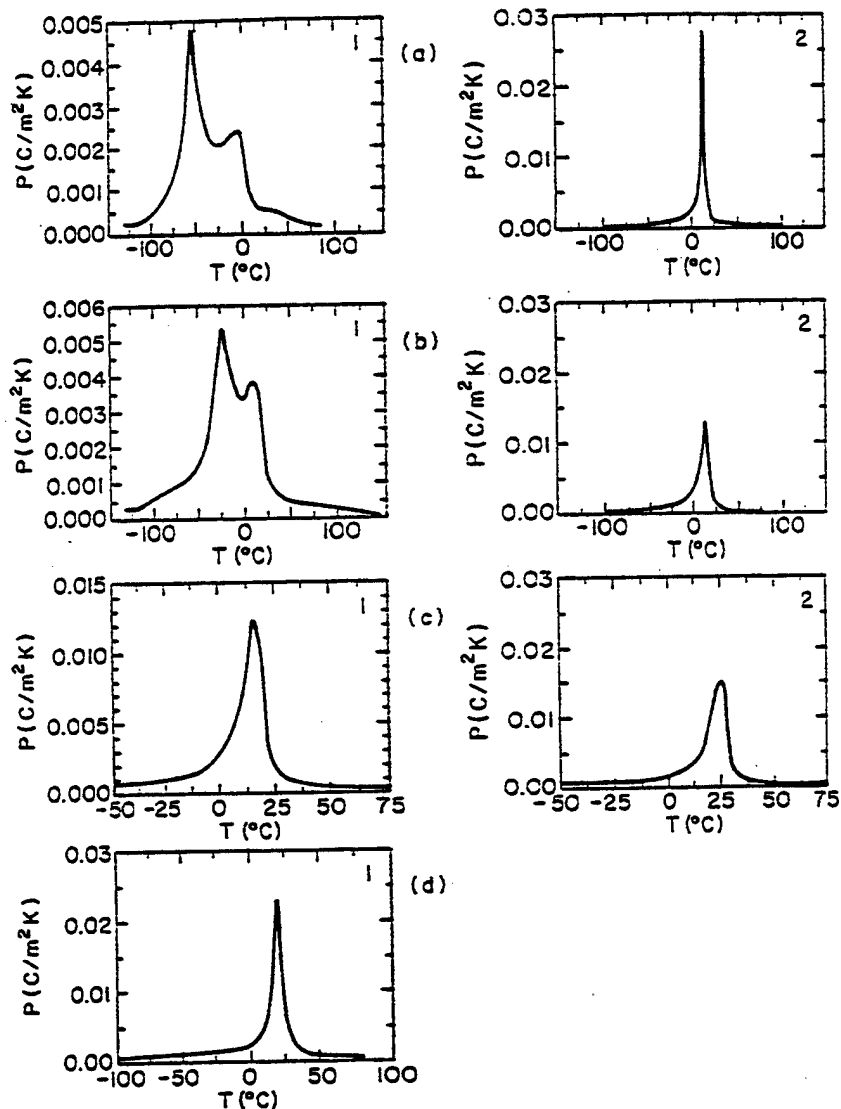
FIGURE 7 The pyroelectric coefficient for As-Fired [1] and Annealed [2] (1-x)\text{Pb}(\text{Sc}_{1/2}\text{Ta}_{1/2})\text{O}_3-(x)\text{PbTiO}_3 ceramics: (a) x=0.025 , (b) x=0.05 , (c) x=0.075 , (d) x=0.1 .
