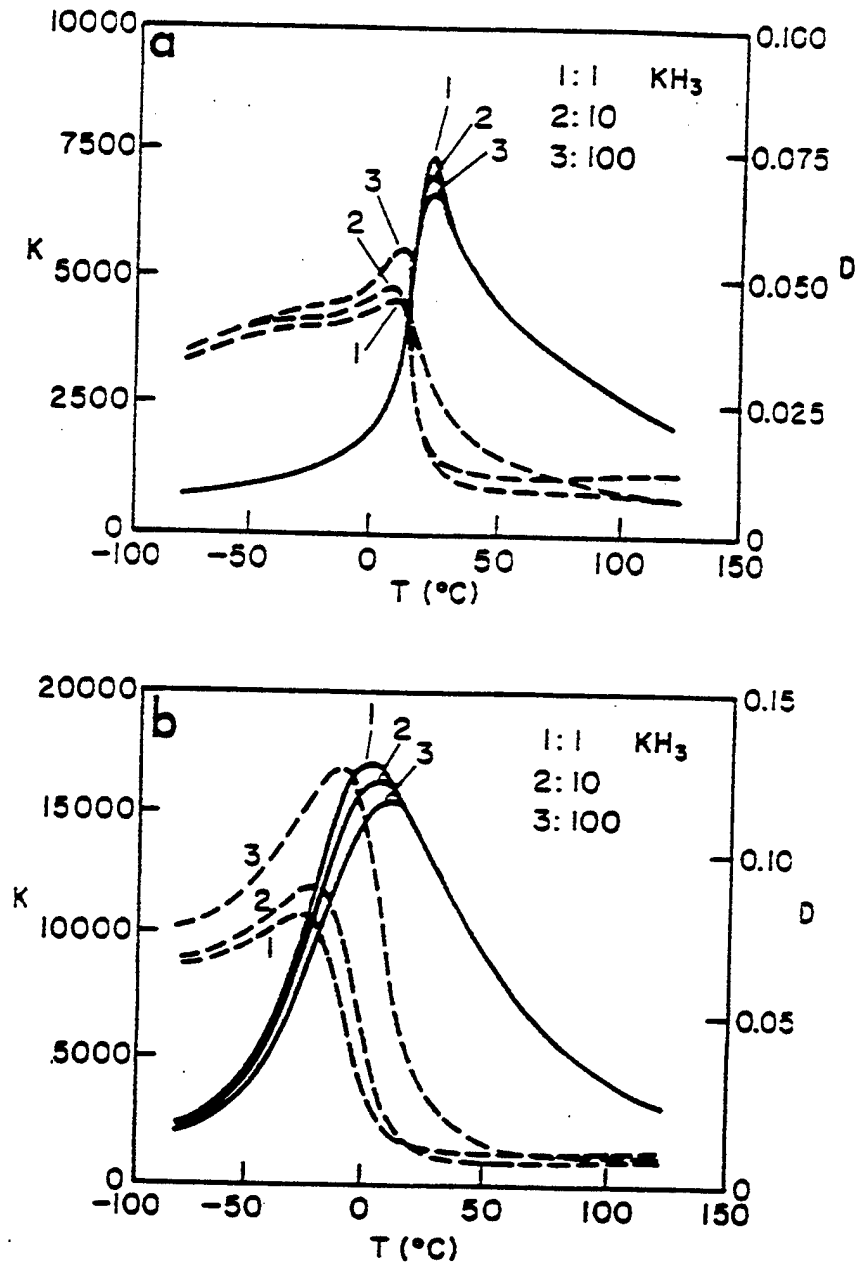
FIGURE 3 The dielectric constant and loss of Pb(Sc_{1/2}Ta_{1/2})O_3 as a function of temperature and frequency [7] . (a) S=0.87 and (b) S=0.4 . (see Section III for definition of S )
