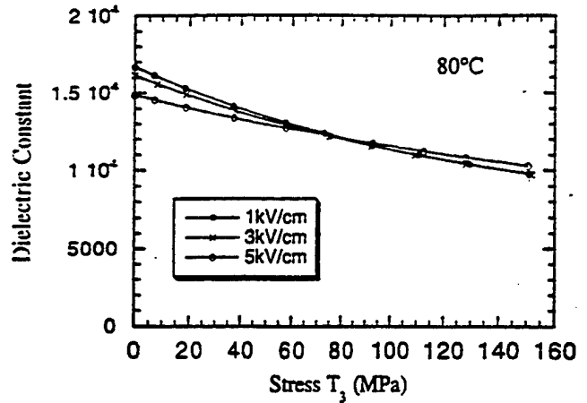
FIG. 5. The dielectric constant as a function of the compressive T_3 at 80 °C, 1 kHz, and under different dc bias fields. The dielectric constant at this temperature exhibits very little dispersion.
