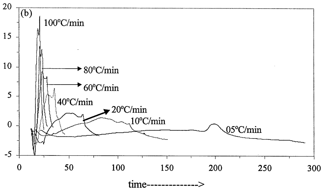
Figure 1. DTA traces for the shock-densified Ti-Si powder compact at different heating rates, showing: (a) \Delta T vs Temperature and (b) \Delta T vs time.
