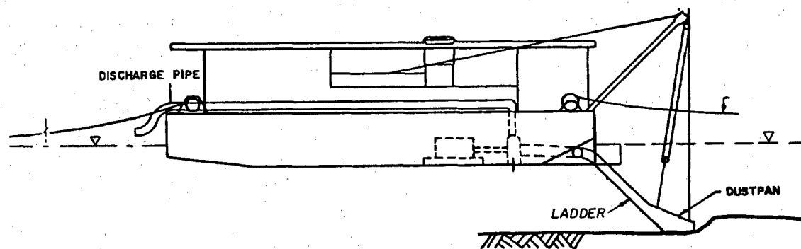
Figure 3-7. Dustpan dredge.
