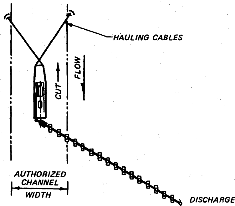
Figure 3-8. Operation of dustpan dredge (viewed from above).
