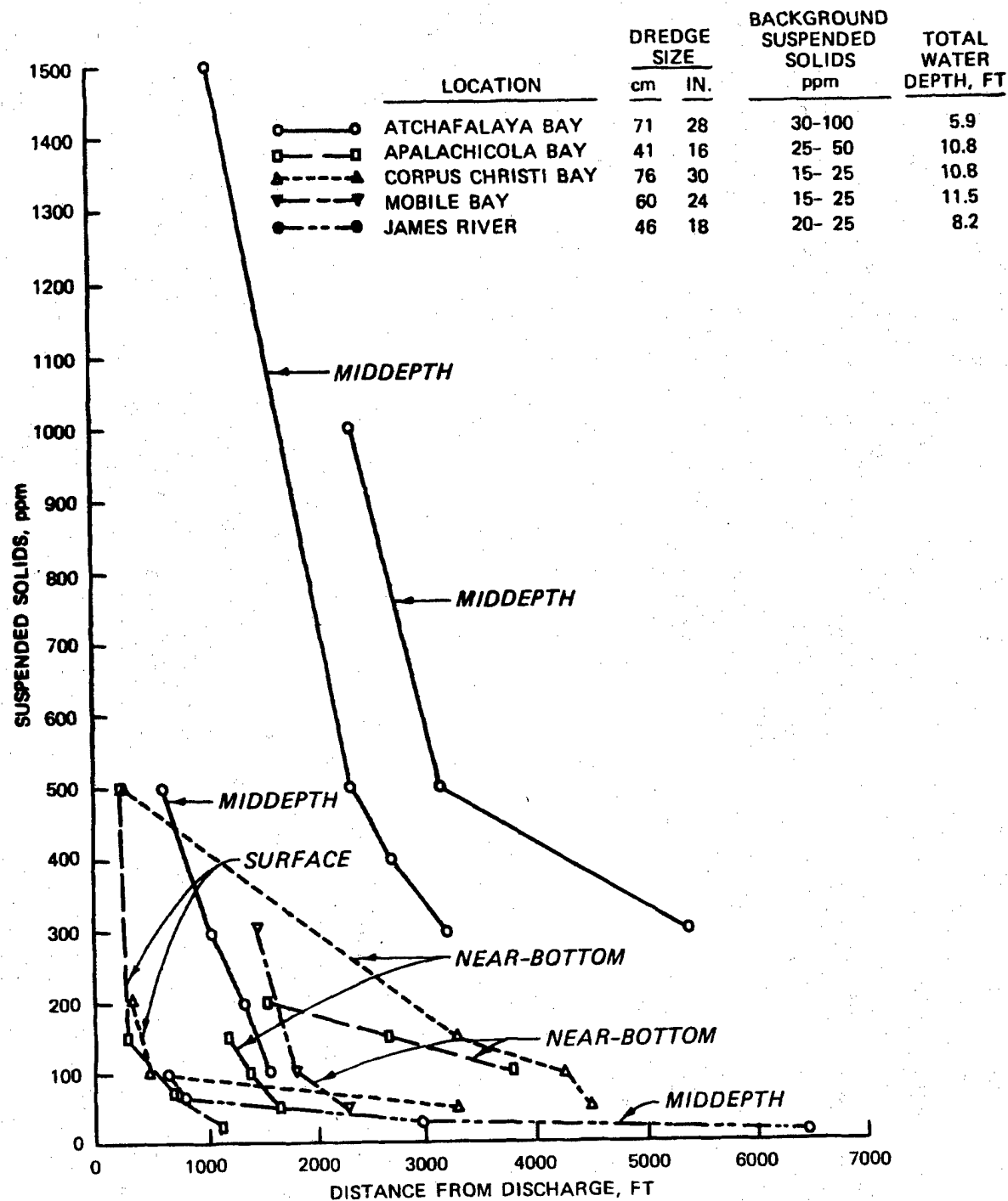
Figure 4-4. Relationship between suspended solids concentration along the plume center line and distance downcurrent from several open-water pipeline disposal operations measured at the indicated water depths,
