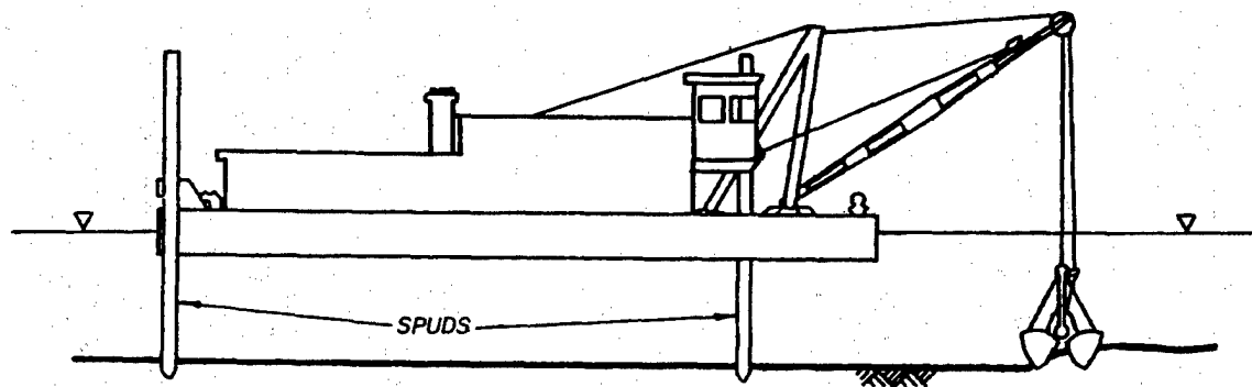
Figure 3-11. Bucket dredge.
