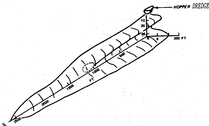
Figure 4-1. Hypothetical suspended solids plume downstream of a hopper dredge operation with overflow in San Francisco Bay (all distances in feet)*
