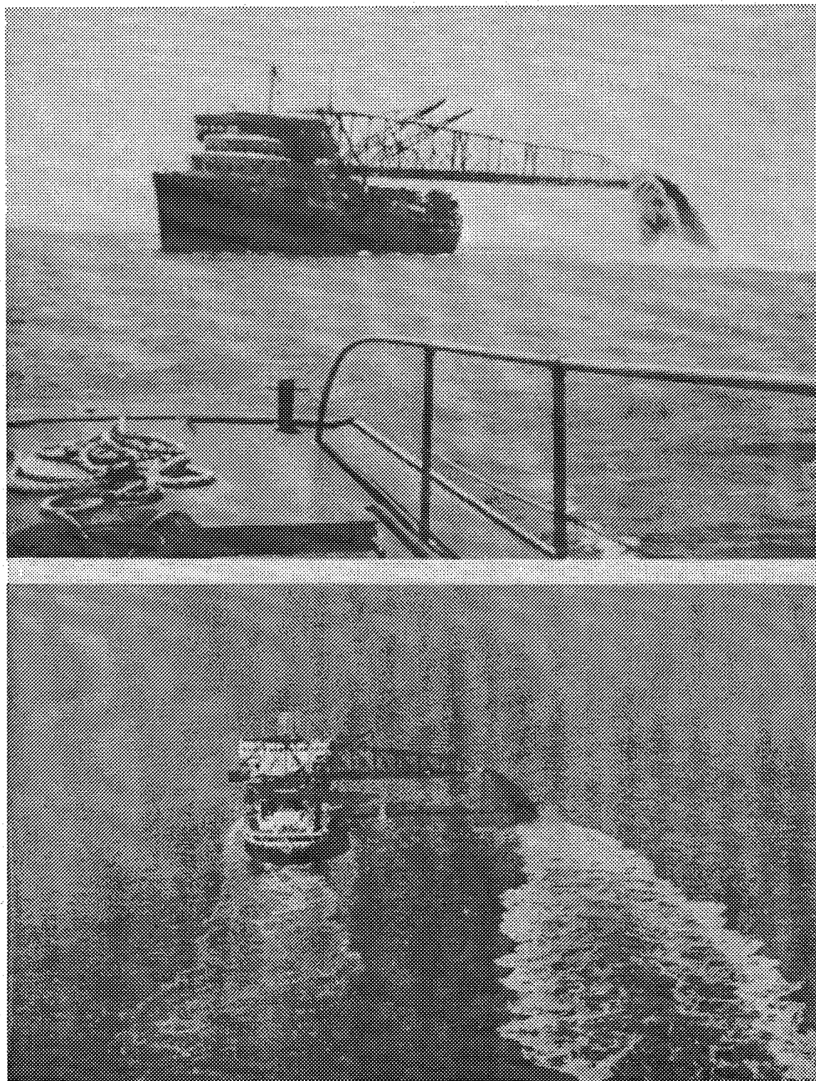
Figure 3-9. Sidecasting dredge.
