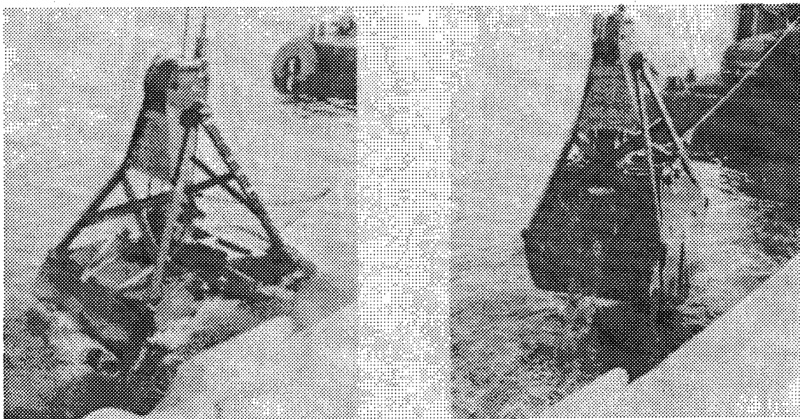
Figure 3-12. Open and closed positions of the watertight bucket.
