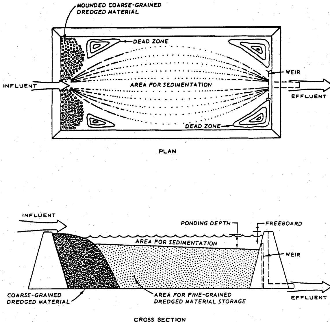
Figure 4-5. Schematic diagram of a dredged material containment area,
