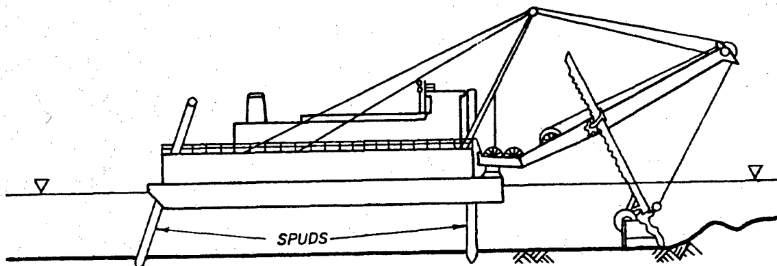
Figure 3-10. Dipper dredge.
