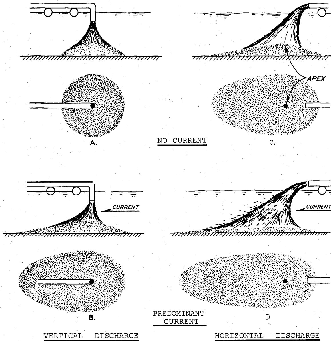
Figure 4-3. Effect of discharge angle and predominant current direction on the shape of a fluid mud mound.
