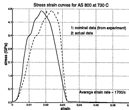
Figure 9: Stress-strain data for in situ reinforced silicon nitride, tested to failure at a strain rate of 1,700/s at 730°C - note that there is a decrease in modulus prior to failure (test data has been corrected using the DSM technique)
