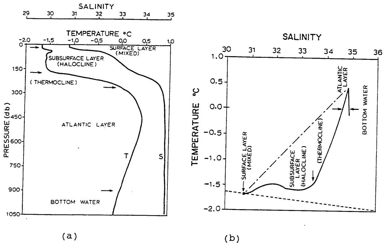
Figure 2.3. Principal water masses in the Canadian Basin, depicted by (a) typical T/S profiles; and (b) correlation in T-S space. (Following Melling and Lewis, 1982).
