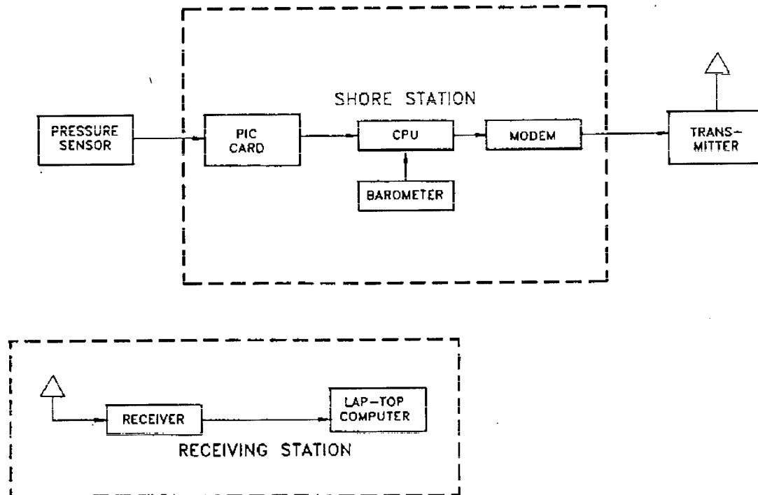
Figure 1. Automated Real-Time Tidal Elevation System
