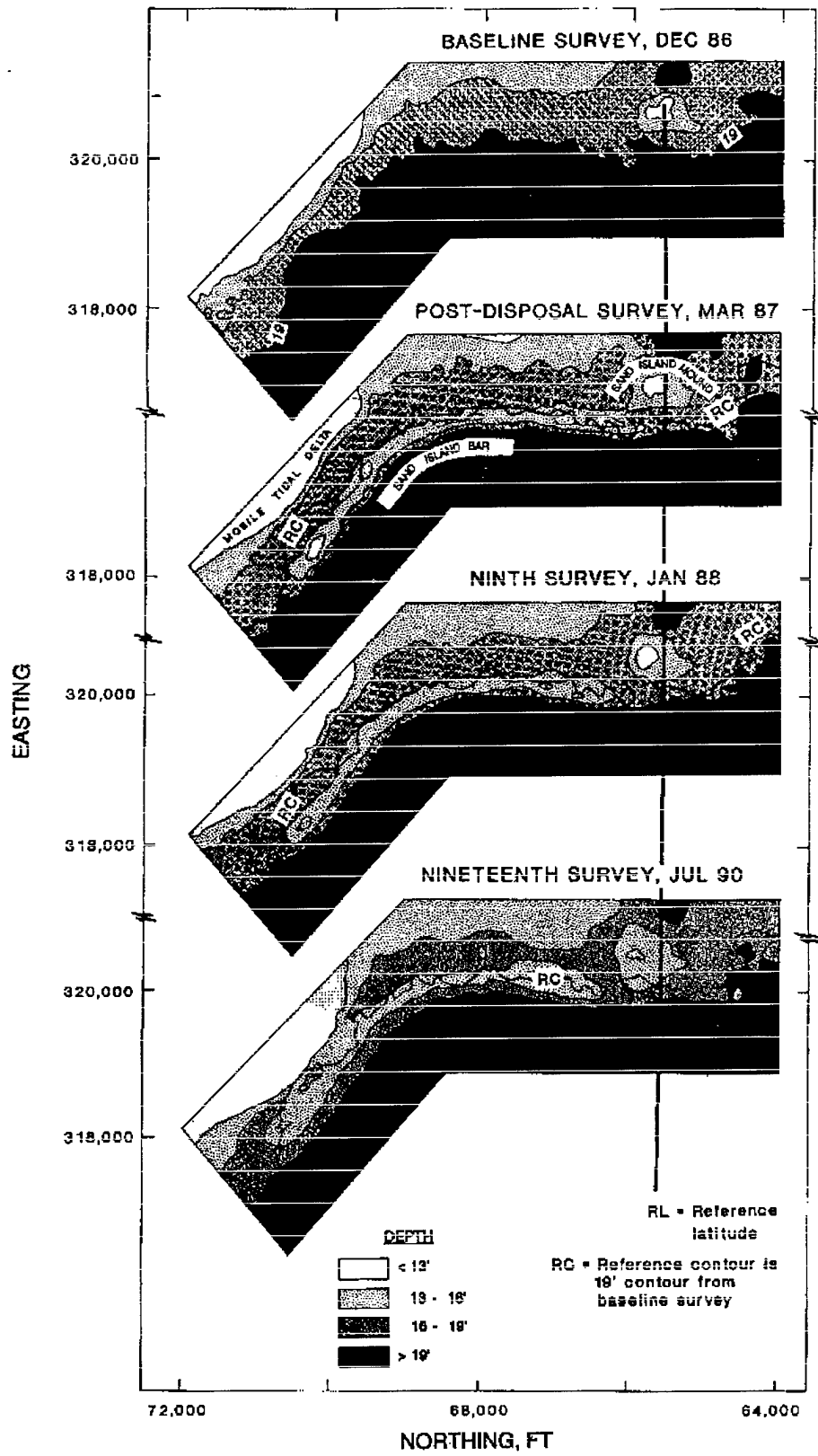
Figure 5. Long-term bathymetric changes in the Sand Island survey area
