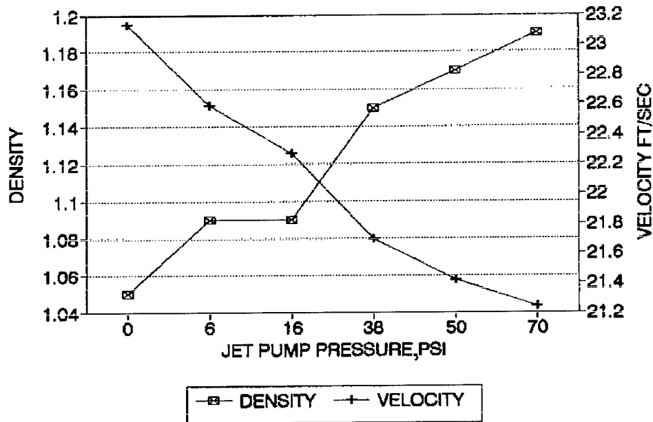
Figure 5. Jet pump pressure versus slurry density and velocity
