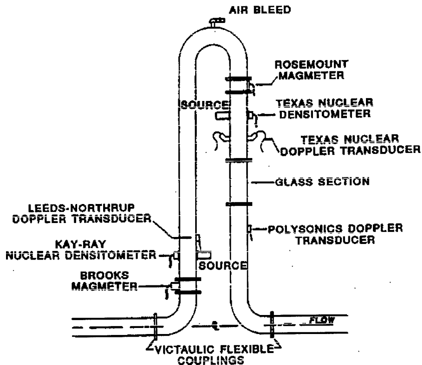
Figure 1. Layout of instrumentation loop
