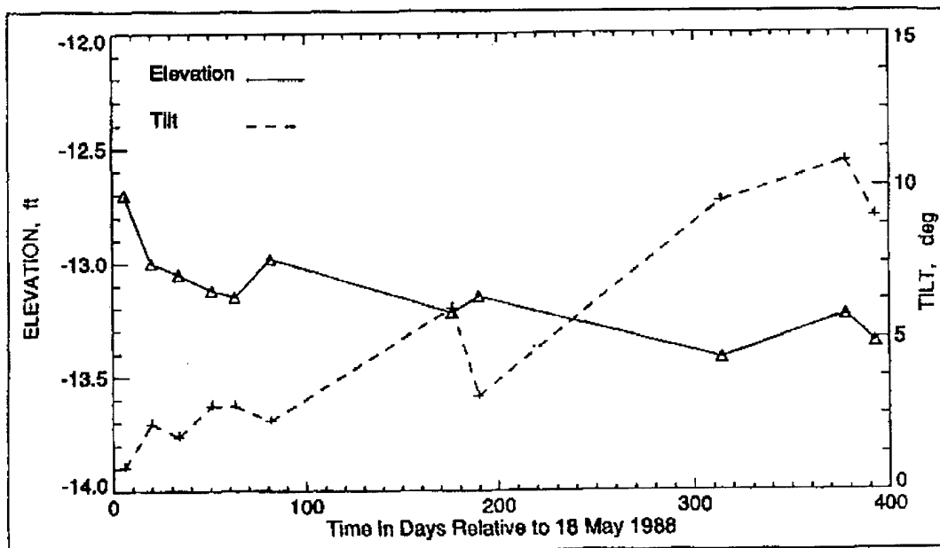
Figure 2. Octapod elevation and tilt
