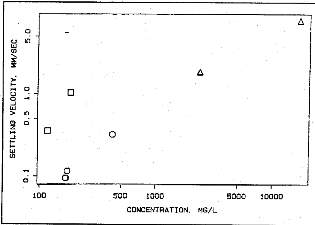
Figure 2. Median settling velocities for the composite sediment observed in the sediment water tunnel (○) and in high-concentration laboratory tests (△), and for resuspended bed material tested in a field settling tube (□)
