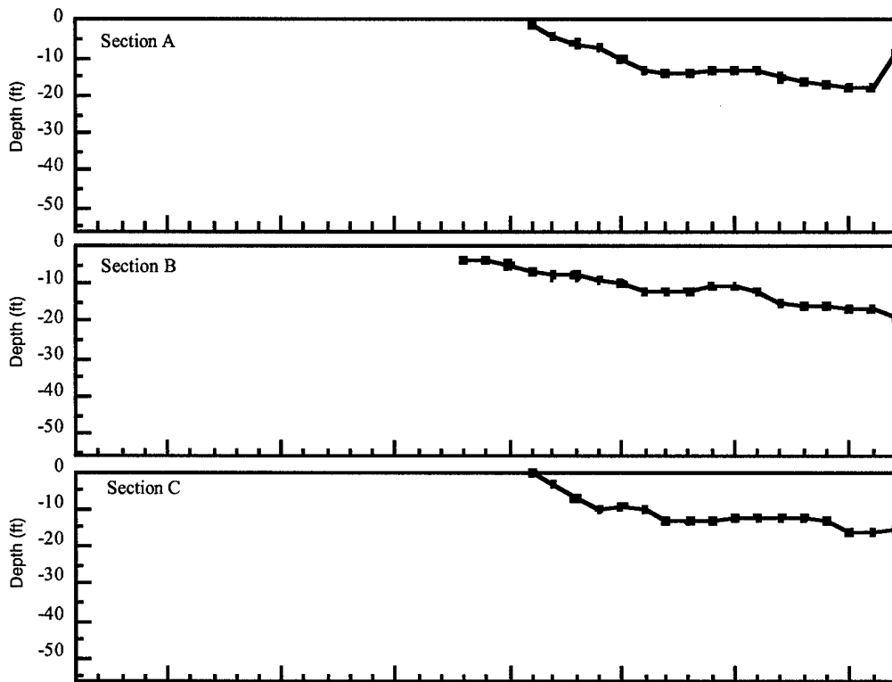
Bathymetry for Missouri (A, B, C sections, 1994 survey)
