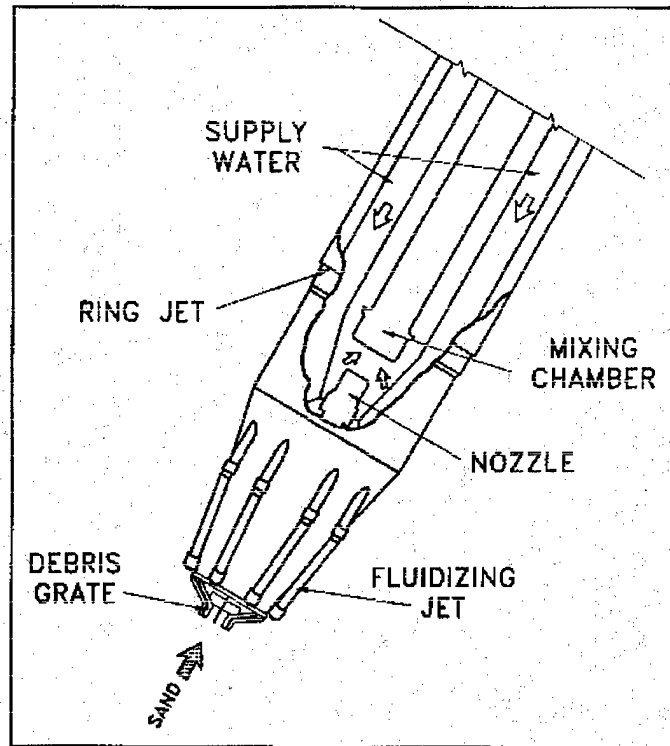
Figure 1. Schematic of DRP eductor
