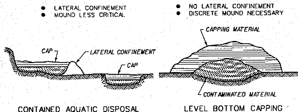
Figure 1. Schematic illustrating level bottom capping and contained aquatic disposal
