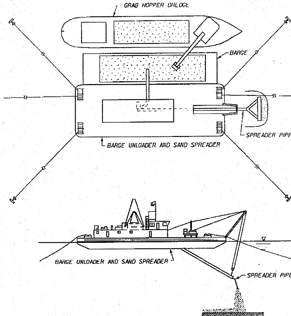
Figure 7. Hydraulic barge unloader and sand spreader barge (from Kikegawa 1981)
