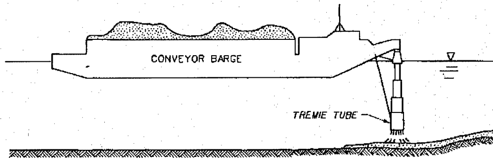
Figure 8. Conveyor unloading barge with tremie (from Togashi 1981)
