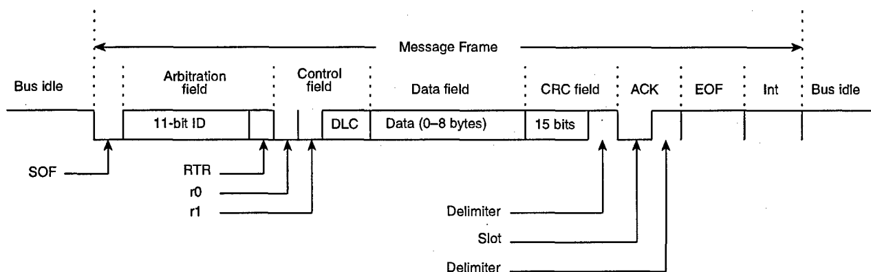
Figure 2. Controller area network standard message frame. (SOF = start of frame, RTR = remote transmission request bit, DLC = data length code, CRC = cyclic redundancy code, ACK = acknowledge bit, EOF = end of frame, Int = interval, and r0, r1 = reserved bits for future use.)
