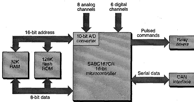
Figure 3. Polymer Battery Experiment telemetry and command interface.
