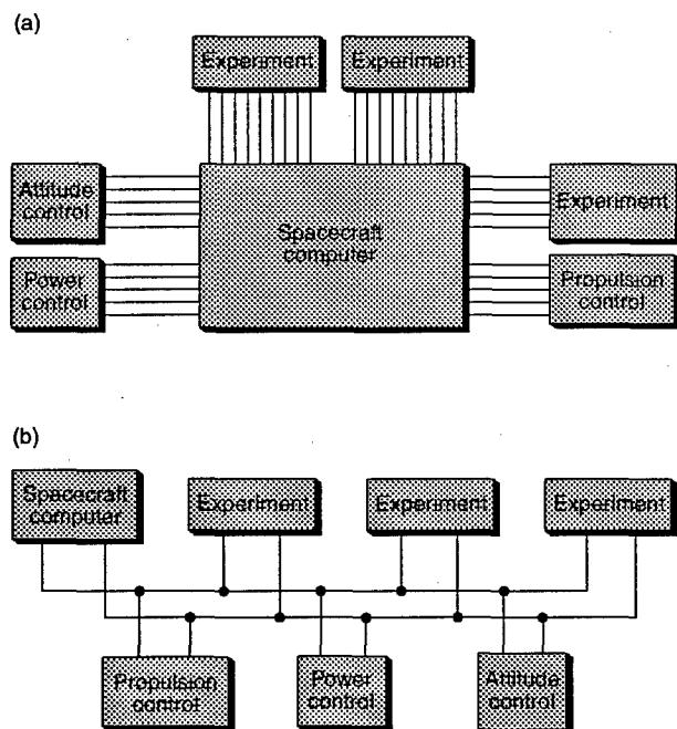
Figure 1. Spacecraft telemetry and command system architectures: (a) centralized, (b) distributed.
