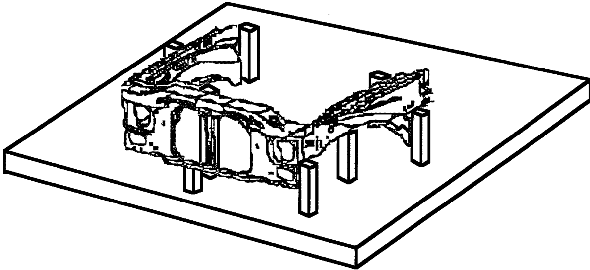
Figure 9-12. Schematic of a Blue Buck holding parts of the frame.
