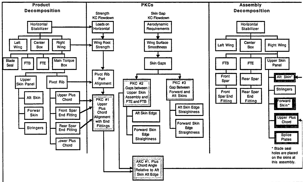
Figure 11-7. Product and Assembly Decompositions and resulting PKCs and AKCs.
