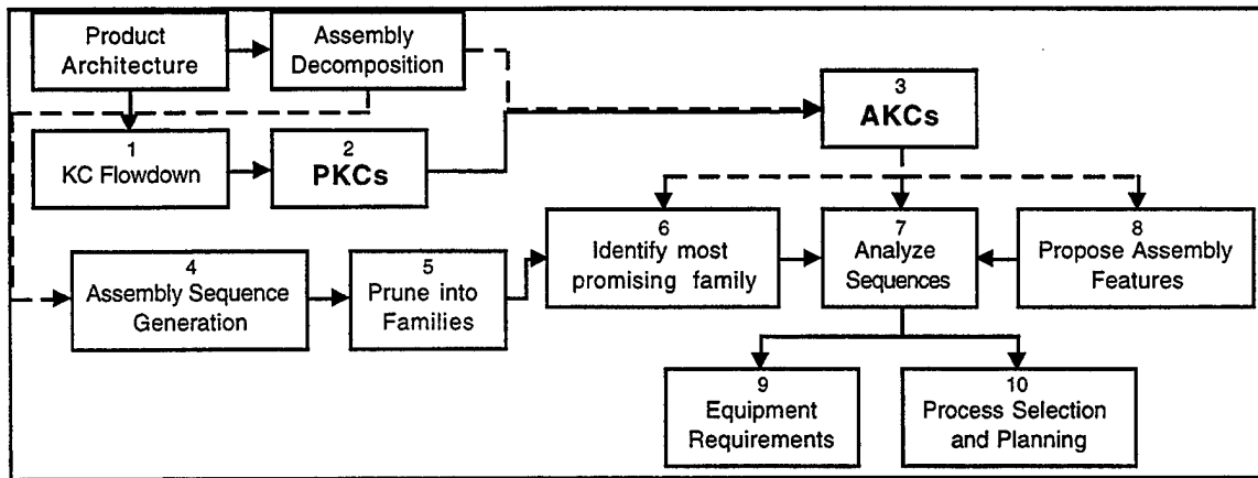
Figure 11-1. Approach to selecting the most promising flexible assembly process.
