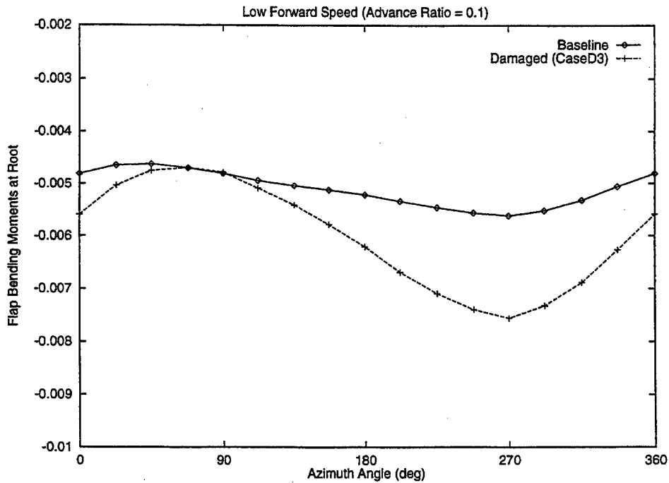
Figure 17. Flap Bending Moments of Undamaged and Damaged Blades in Forward Flight ( \mu = 0.1 ).
