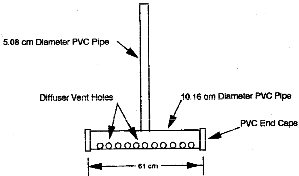
Figure 5. Horizontal diffuser design
