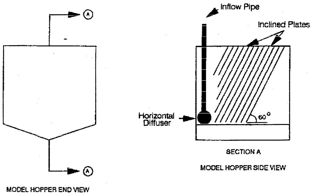
Figure 4. Approximate plate configuration in the hopper, section view
