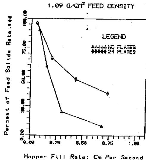
Figure 8. Percent of feed solids retained for a 200-sec overflow duration
