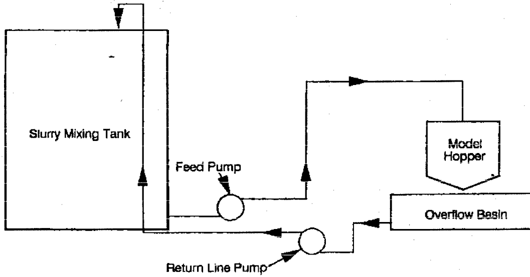
Figure 2. Model hopper overflow test loop
