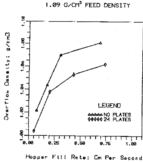
Figure 7. Overflow density at equilibrium for a 200-sec overflow duration
