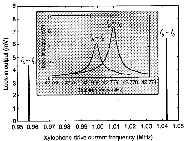
Figure 6. The amplitude of the xylophone response to a high-frequency sinusoidal (1-MHz) magnetic field as a function of drive current. The insert shows the two resonances overlaid side-by-side for comparison purposes.
