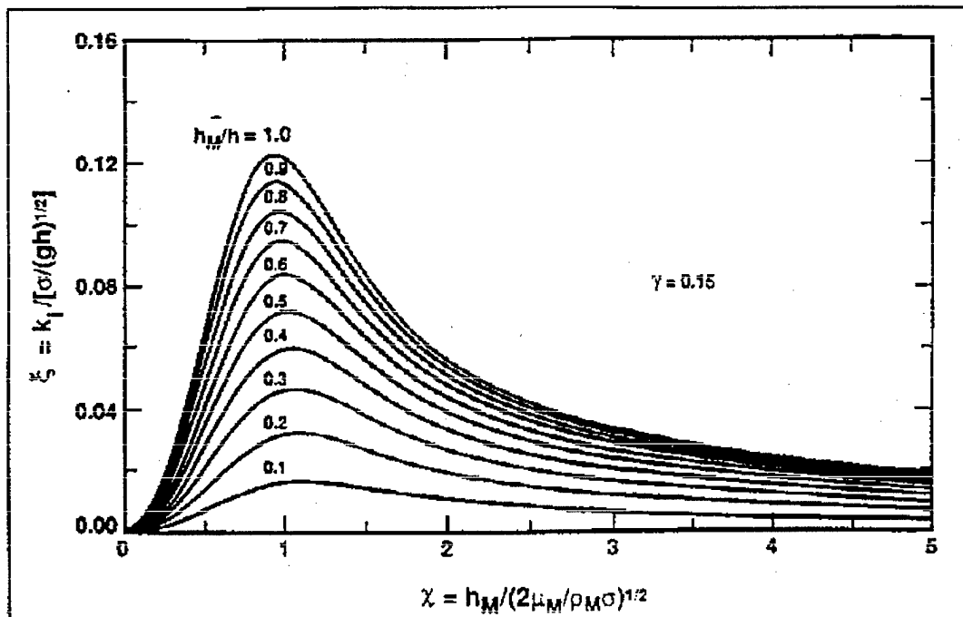
Figure 8. Relationship between \xi and \chi representing the effects of wave energy dissipation in mud on wave attenuation in shallow water. (Corresponding wave number presented in Figure 9)
