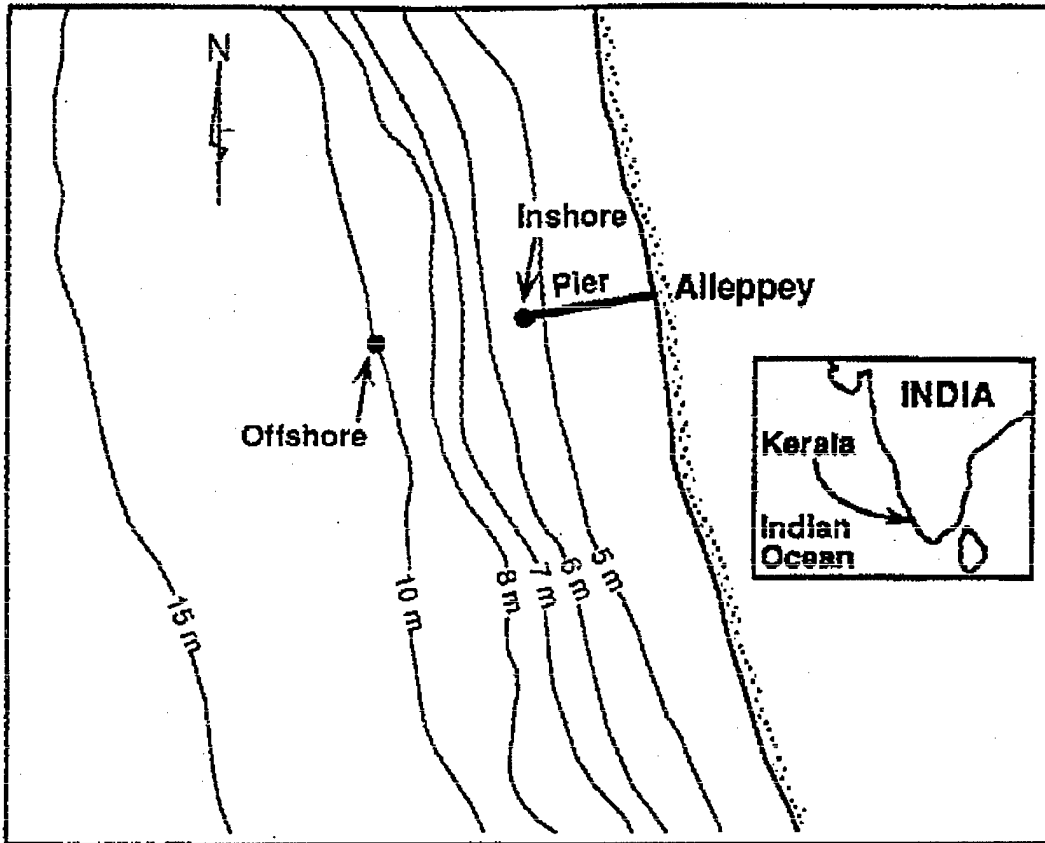
Figure 3. Coastal site at Alleppey in Kerala, India, where monsoonal, shore-parallel mudbanks occur. The pier is 300 m long (after Mathew 1992)
