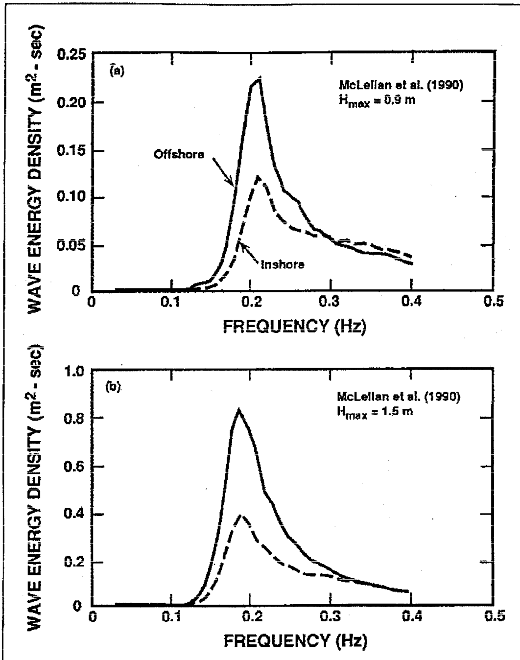
Figure 7. Offshore and inshore wave spectra at the Mobile berm site for two different wave conditions at the offshore site characterized by the maximum wave height, H_{max} : (a) H_{max} = 0.9 m, and (b) H_{max} = 1.5 m (after McLellan, Pope, and Burke 1990)
