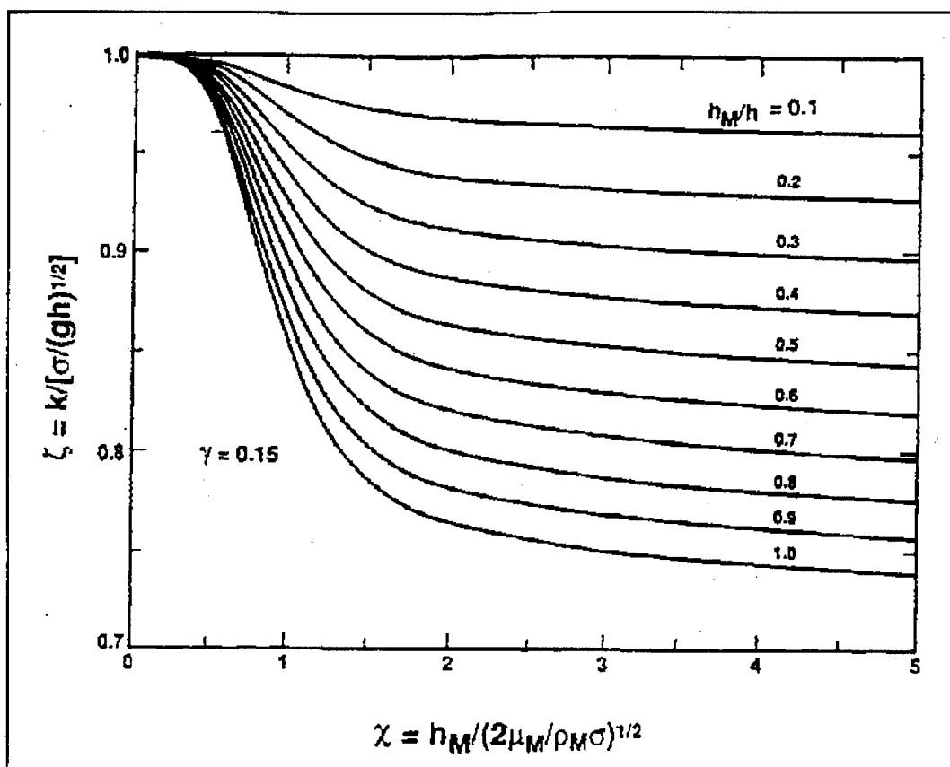
Figure 9. Relationship between \zeta and \chi , for determining the wave number corresponding to Figure 8
