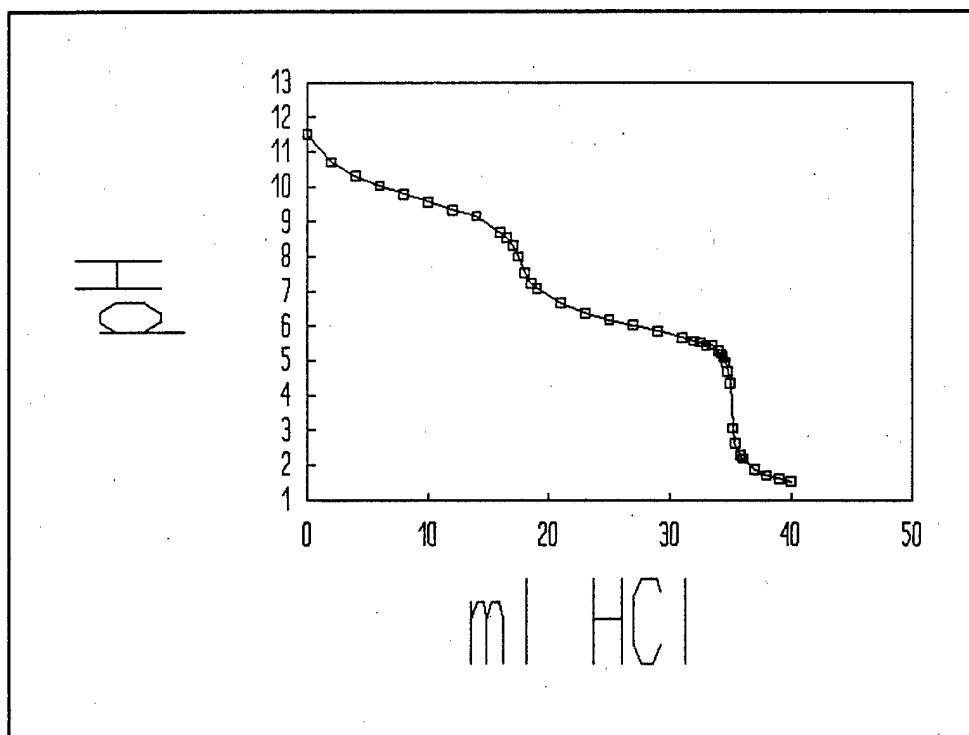
Figure C-226. Curve For The Second Titration Of Spent <45 Micron Sodium Bicarbonate Media With 0.981 M HCl.
