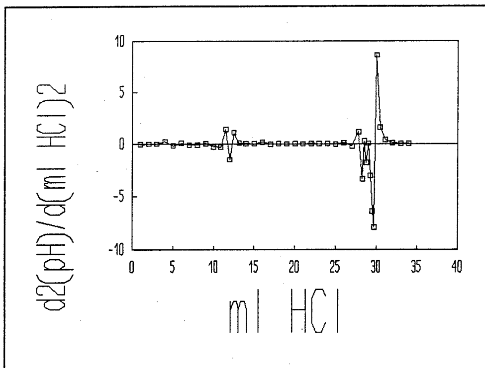
Figure C-174. Second Derivative Of The Fourth Titration Curve For Titration Of Spent 250 Micron Sodium Bicarbonate Media With 0.984 M HCl.
