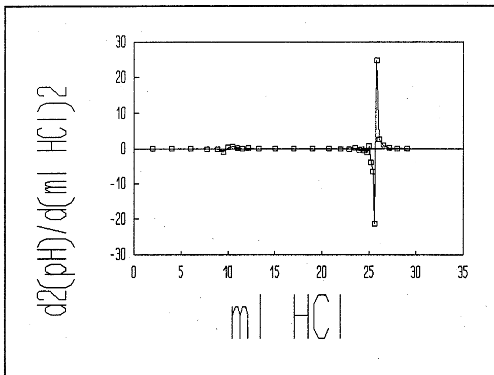
Figure C-57. Second Derivative Of The Third Titration Curve For Titration Of Fresh 150 Micron Sodium Bicarbonate Media With 0.961 M HCl.
