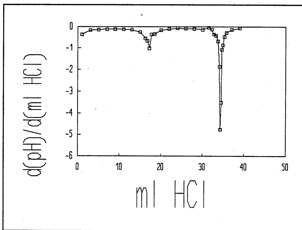
Figure C-107. First Derivative Of The Fourth Titration Curve For Titration Of Fresh <45 Micron Sodium Bicarbonate Media With 0.961 M HCl.
