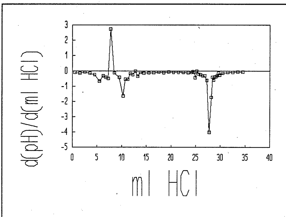
Figure C-122. First Derivative Of The Third Titration Curve For Titration Of Total Spent Sodium Bicarbonate Media With 0.984 M HCl.
