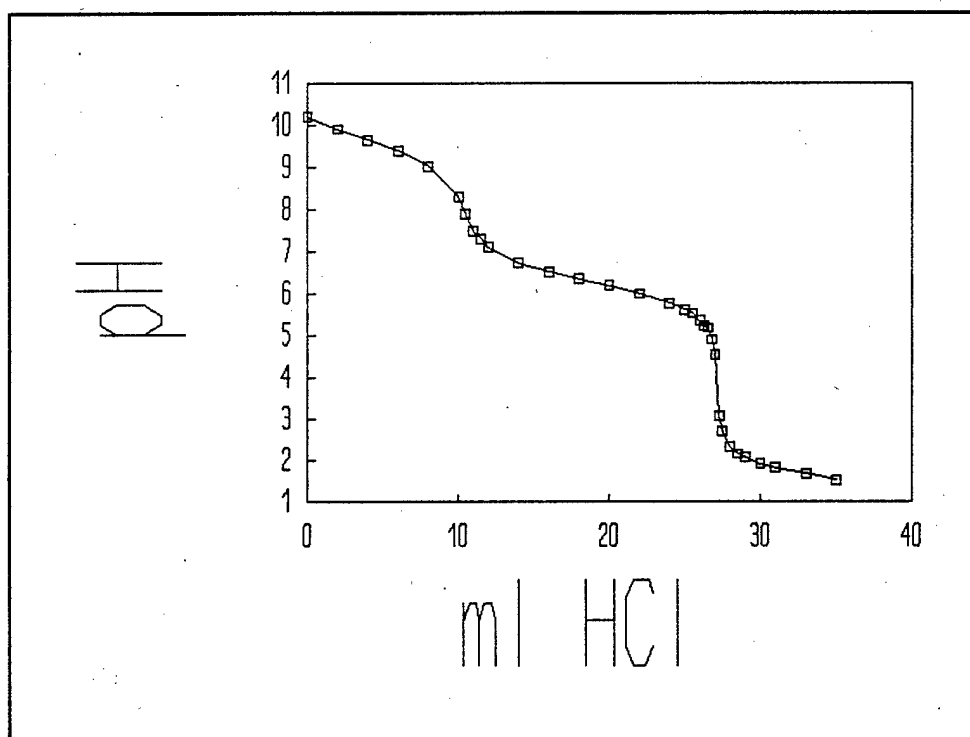
Figure C-34. Curve For The Third Titration Of Fresh 425 Micron Sodium Bicarbonate Media With 0.981 M HCl.
