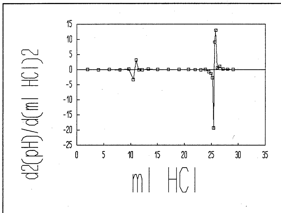
Figure C-51. Second Derivative Of The First Titration Curve For Titration Of Fresh 150 Micron Sodium Bicarbonate Media With 0.961 M HCl.
