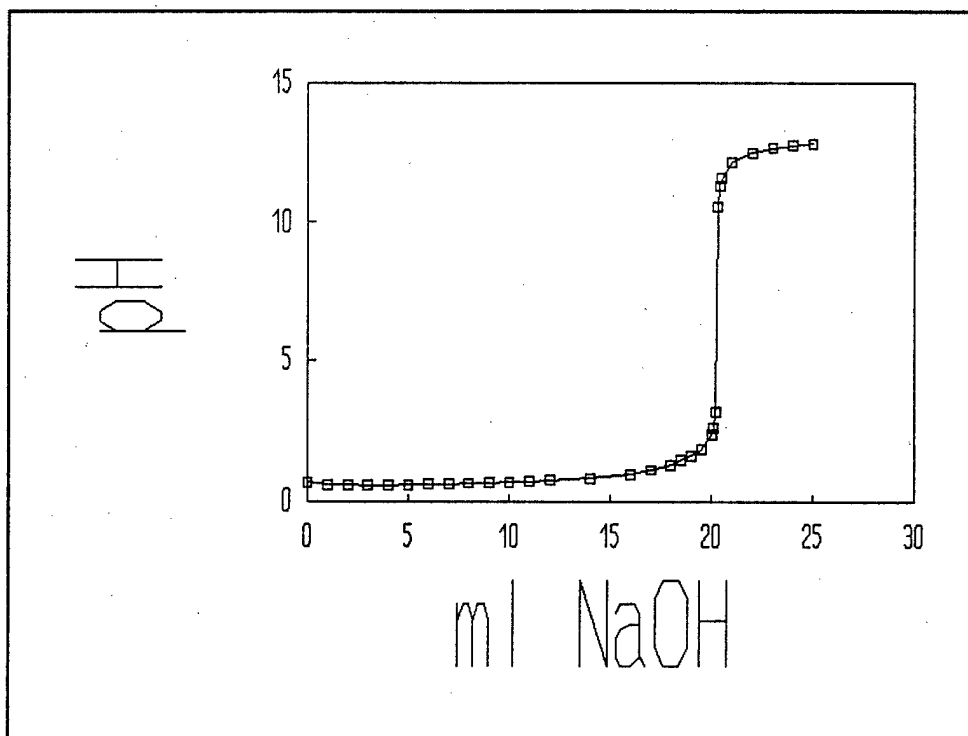
Figure C-7. Titration Curve For The Standardization Of The Second Batch Of HCl With 0.969 M NaOH.
