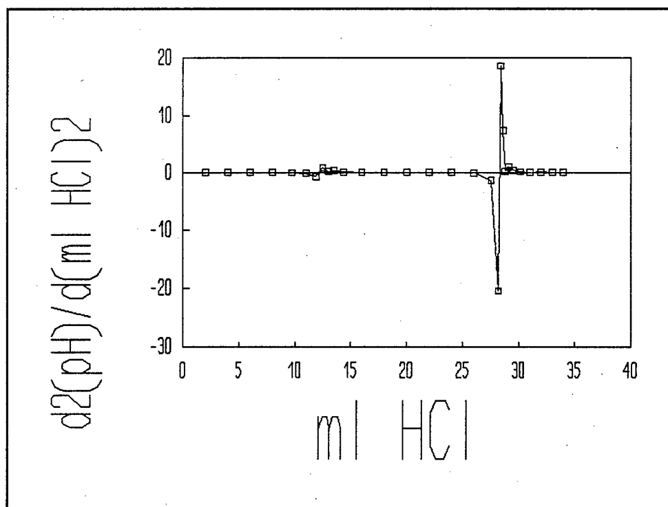
Figure C-33. Second Derivative Of The Second Titration Curve For Titration Of Fresh 425 Micron Sodium Bicarbonate Media With 0.981 M HCl.
