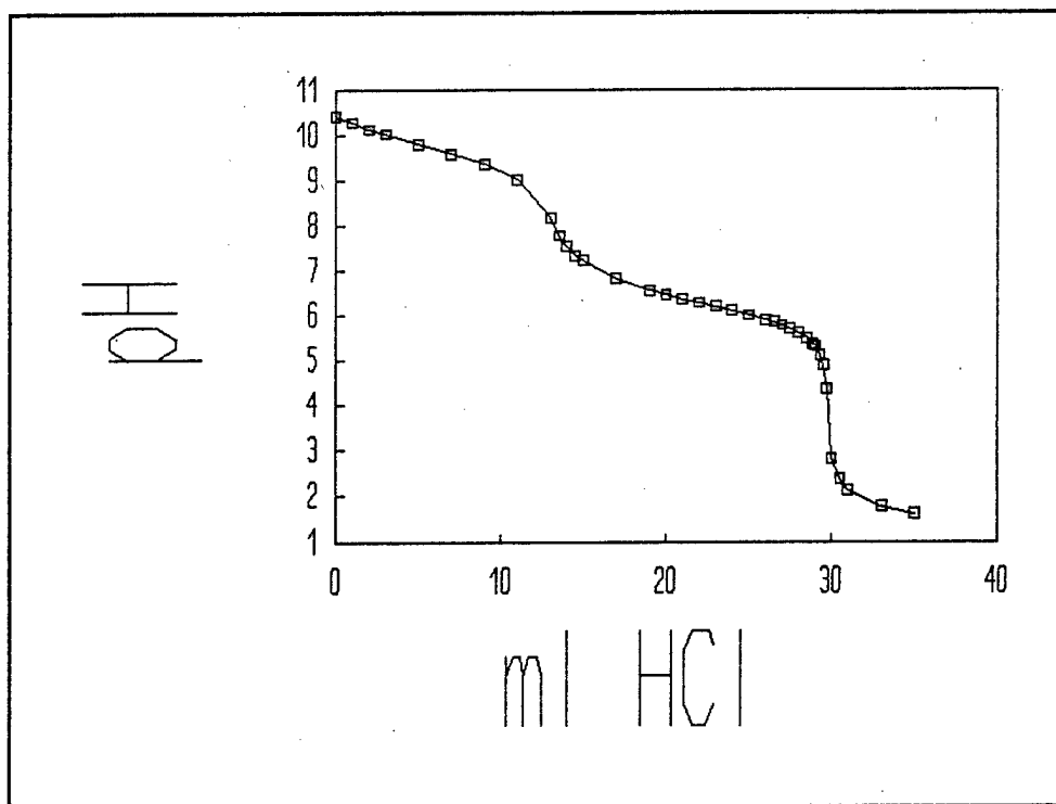
Figure C-199. Curve For The First Titration Of Spent 75 Micron Sodium Bicarbonate Media With 0.981 M HCl.
