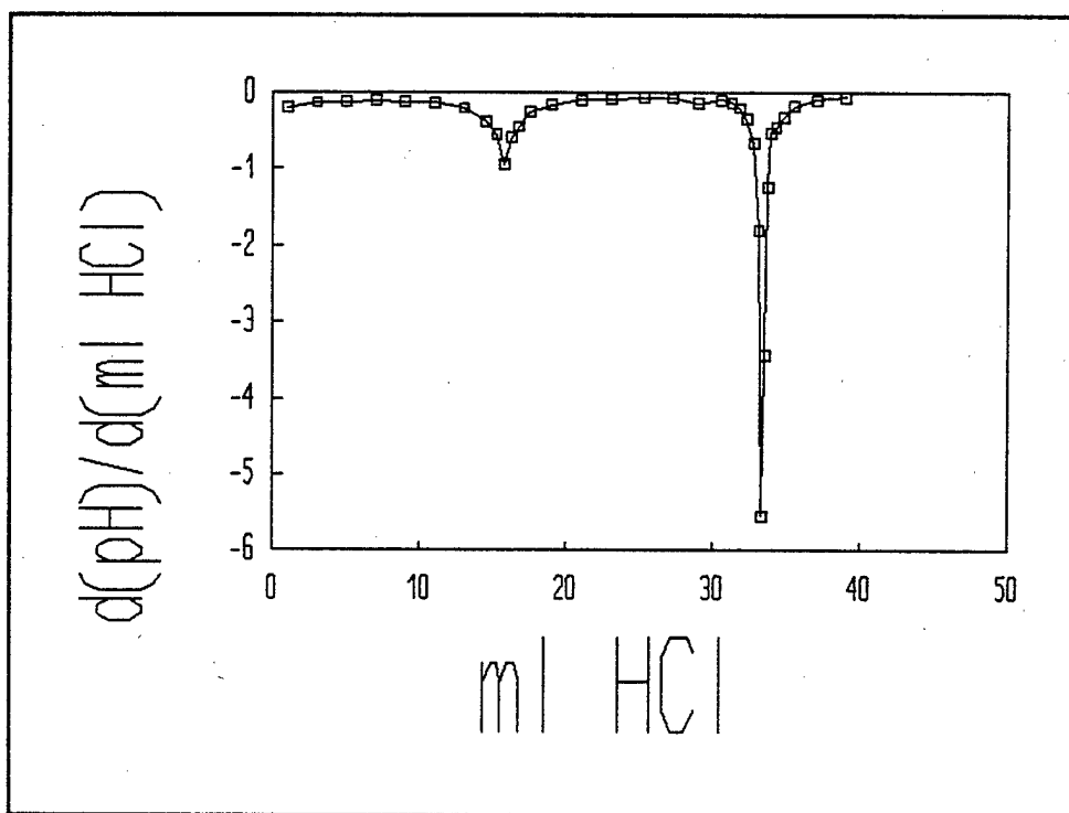
Figure C-95. First Derivative Of The Fourth Titration Curve For Titration Of Fresh 45 Micron Sodium Bicarbonate Media With 0.961 M HCl.
