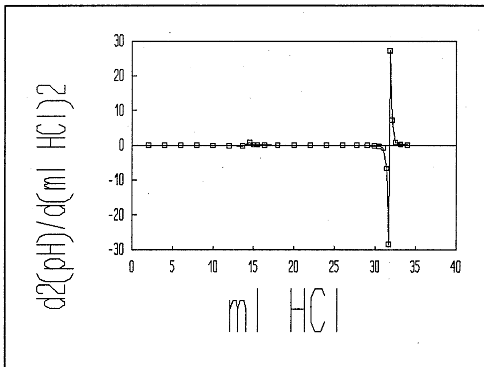
Figure C-207. Second Derivative Of The Third Titration Curve For Titration Of Spent 75 Micron Sodium Bicarbonate Media With 0.981 M HCl.
