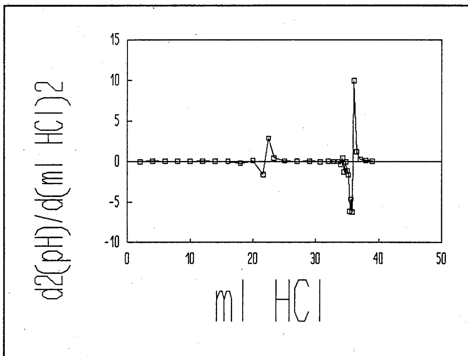
Figure C-225. Second Derivative Of The First Titration Curve For Titration Of Spent <45 Micron Sodium Bicarbonate Media With 0.981 M HCl.
