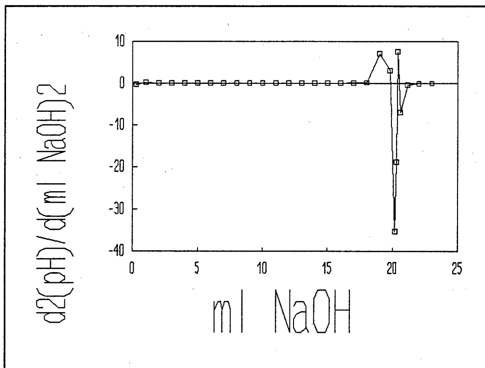
Figure C-12. Second Derivative Of The Titration Curve For The Standardization Of The Third Batch Of HCl With 0.969 M NaOH.
