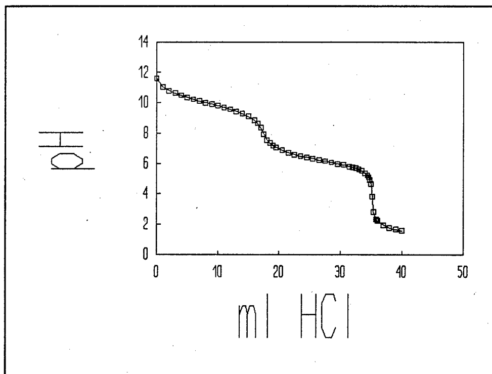
Figure C-145. Curve For The Third Titration Of Spent 600 Micron Sodium Bicarbonate Media With 0.984 M HCl.
