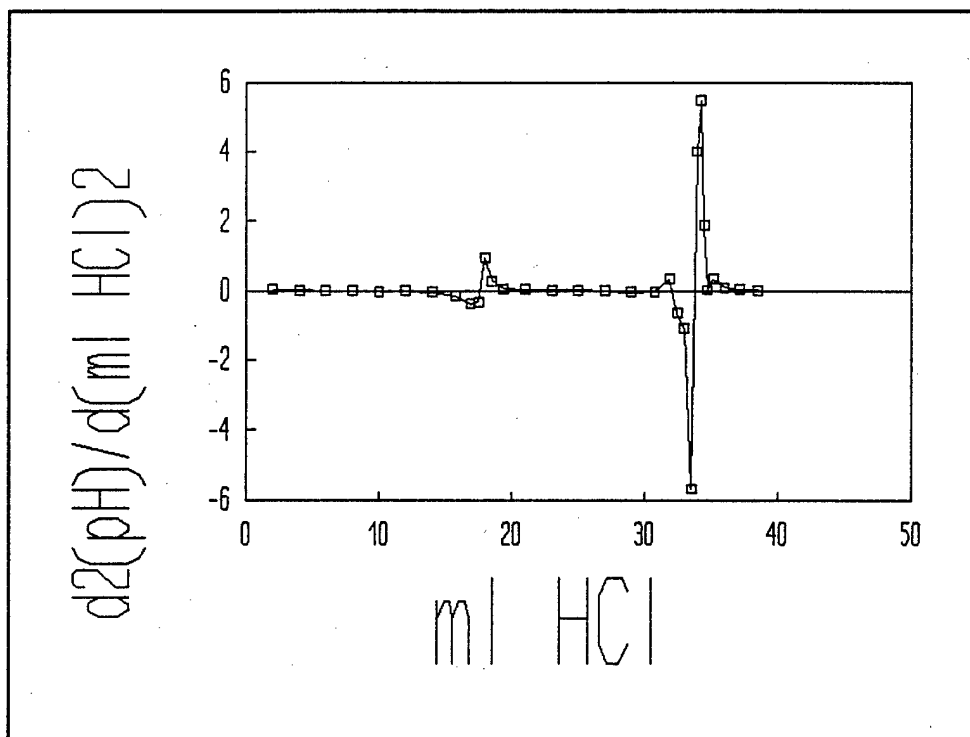
Figure C-213. Second Derivative Of The First Titration Curve For Titration Of Spent 45 Micron Sodium Bicarbonate Media With 0.981 M HCl.
