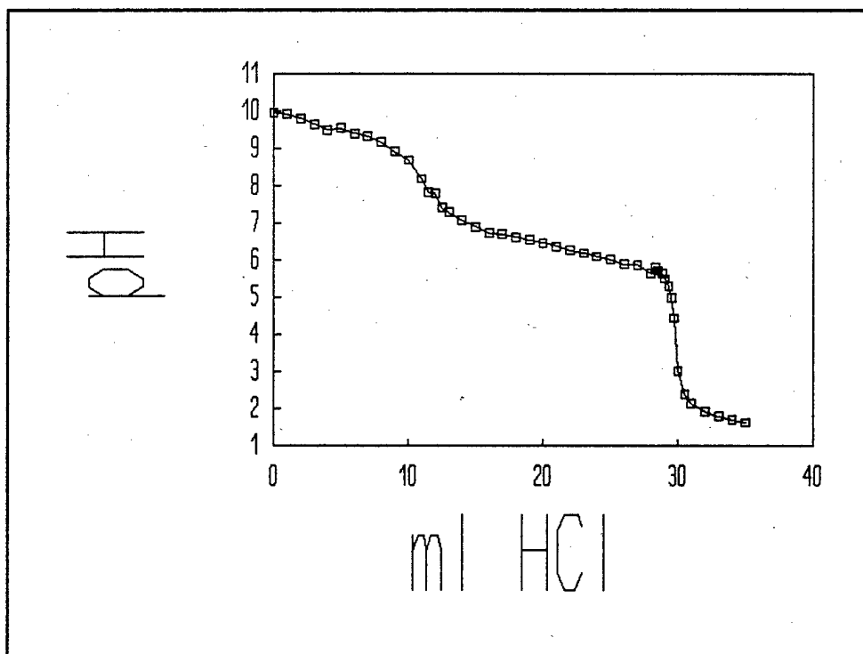
Figure C-172. Curve For The Fourth Titration Of Spent 250 Micron Sodium Bicarbonate Media With 0.984 M HCl.
