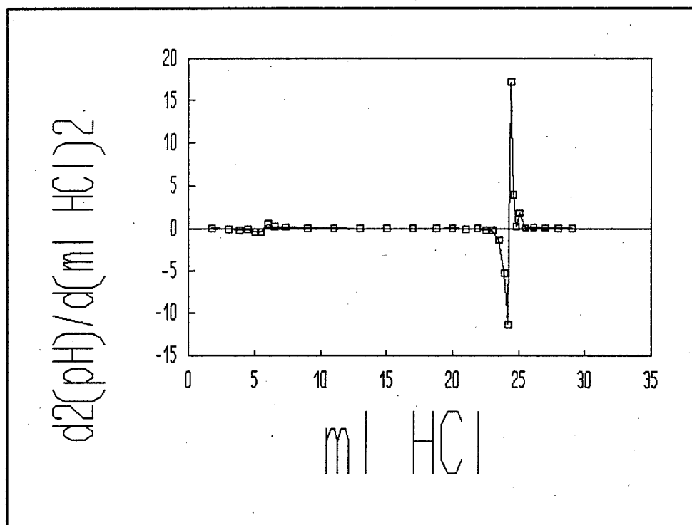
Figure C-39. Second Derivative Of The First Titration Curve For Titration Of Fresh 250 Micron Sodium Bicarbonate Media With 0.961 M HCl .
