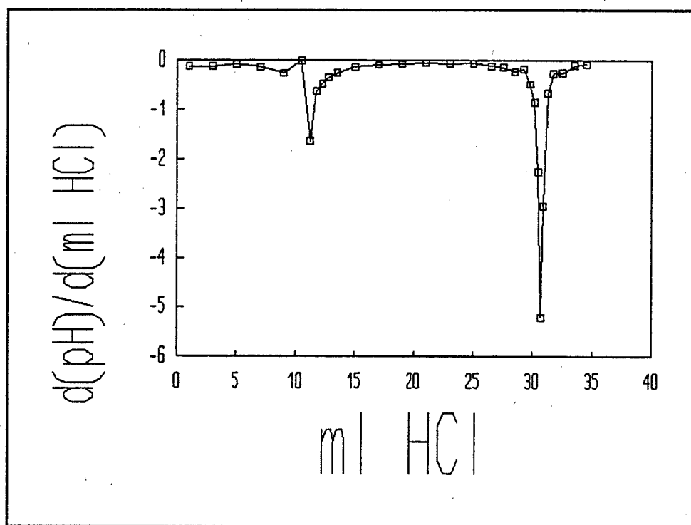
Figure C-83. First Derivative Of The Fourth Titration Curve For Titration Of Fresh 75 Micron Sodium Bicarbonate Media With 0.961 M HCl.
