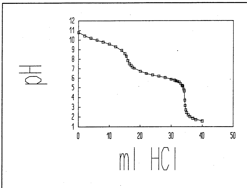
Figure C-91. Curve For The Third Titration Of Fresh 45 Micron Sodium Bicarbonate Media With 0.961 M HCl.
