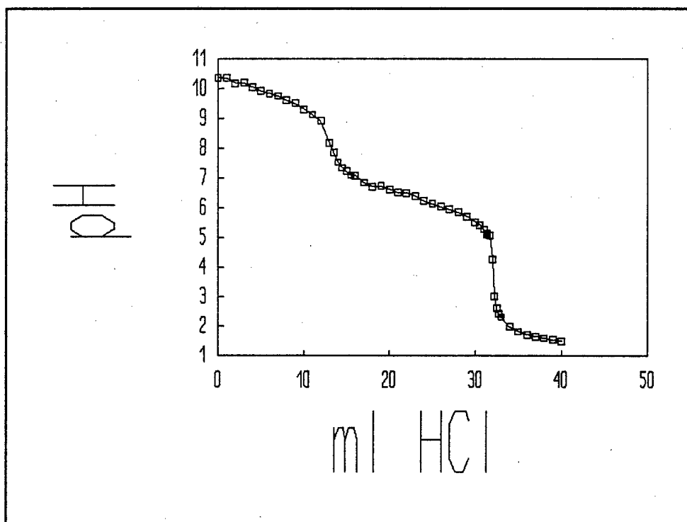
Figure C-154. Curve For The Second Titration Of Spent 450 Micron Sodium Bicarbonate Media With 0.984 M HCl.
