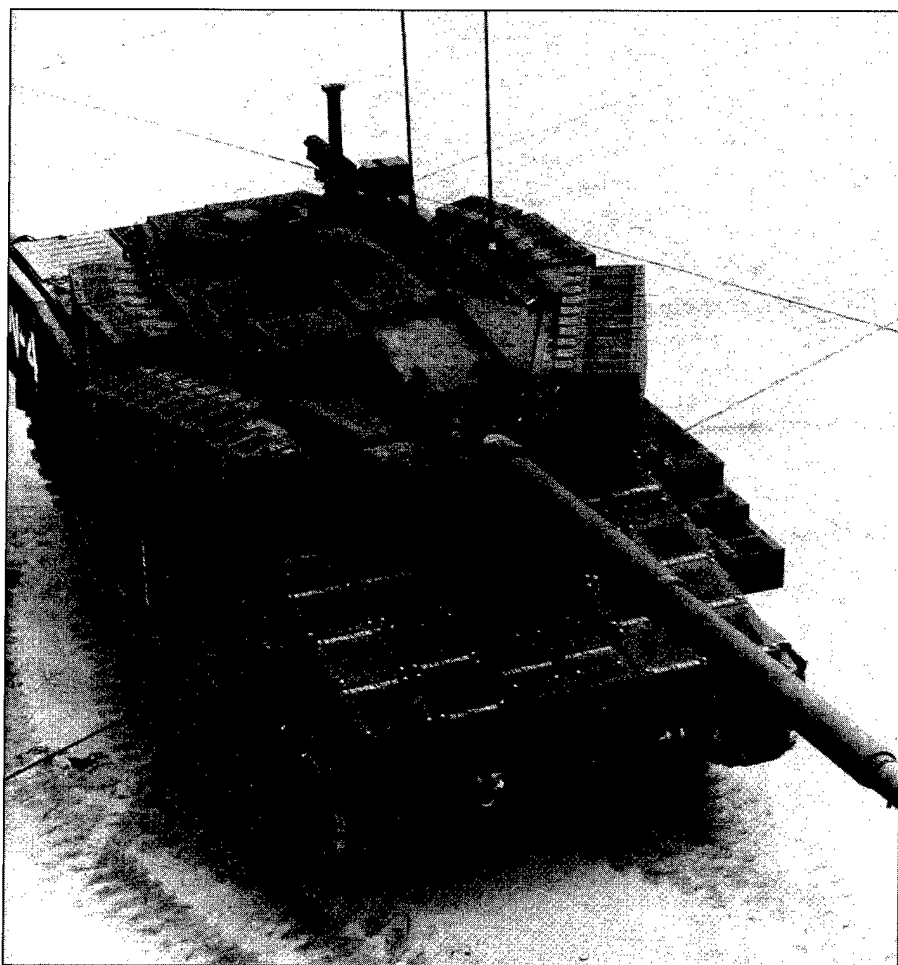
The AGS light tank system, shown here with the heaviest of its three levels of add-on armor, was intended as a replacement for the M551. It was designed to be delivered by air to provide 105mm firepower for light forces. But after several prototypes were built and testing had begun, the project was canceled to save money.
