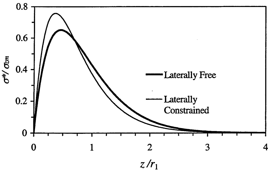
Figure 3.13: Comparison of the interfacial shear stress in both laterally free and laterally constrained systems for the case of a cracked matrix at z = 0 with \epsilon = 0.8\% .
