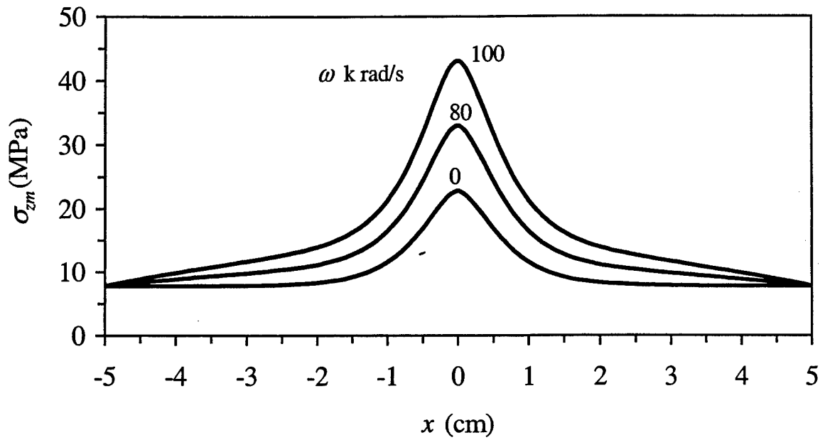
Figure 3.19: Variation of the amplitude of the matrix normal stress distribution with the loading frequency for the case of a broken fiber at z = 0 .
