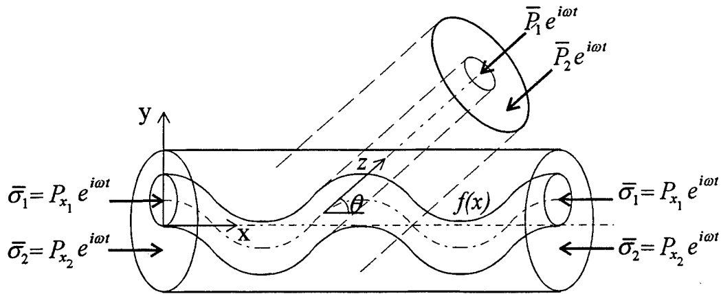
Figure 4.4: Solution Strategy for an undulated segment.
