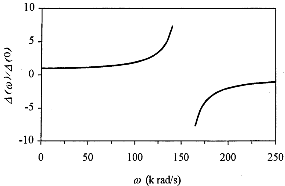
Figure 5.12: Variation of the amplitude of the fiber break opening displacement with the loading frequency for the case of undulated fiber.
