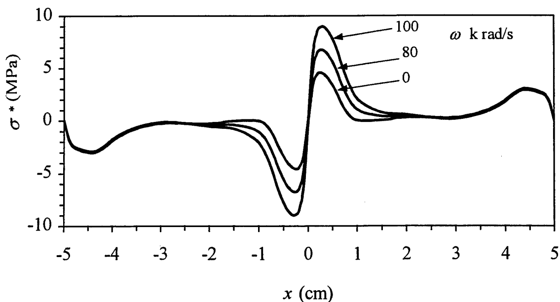
Figure 5.11: Variation of the amplitude of the interfacial shear stress distribution with the loading frequency for the case of undulated fiber with a break.
