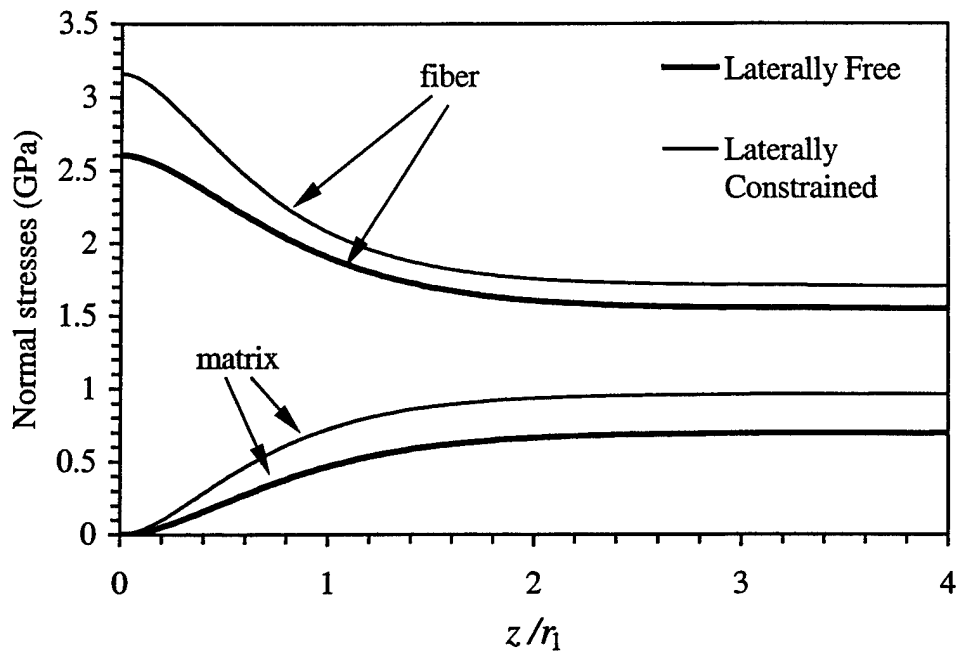
Figure 3.12: Comparison of the fiber and matrix normal stress in both laterally free and laterally constrained systems for the case of a cracked matrix at z = 0 with \epsilon = 0.8\% .
