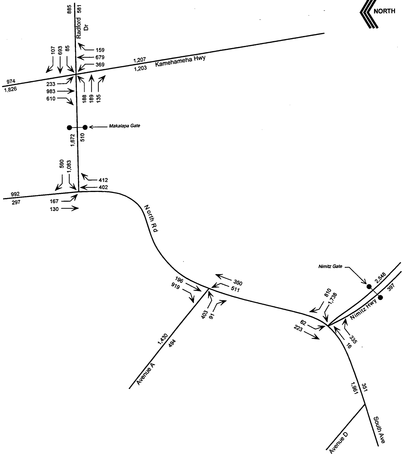
Figure 4-1 YEAR 2005 WITH CARRIER MORNING ARRIVAL PEAK HOUR TRAFFIC
