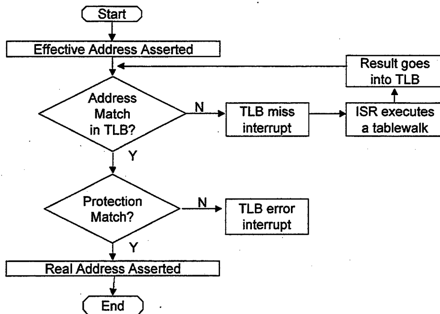
Figure 31. MMU Flow Diagram [Ref. 20]
