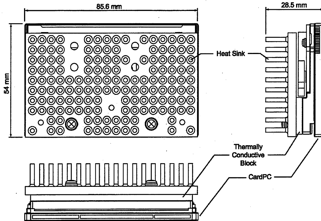
Figure 24. CardPC Heat Sink [Ref. 25]
