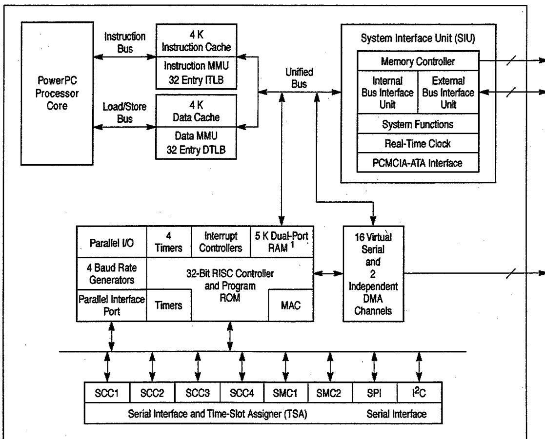
Figure 27. MPC860 Block Diagram [Ref. 68]
