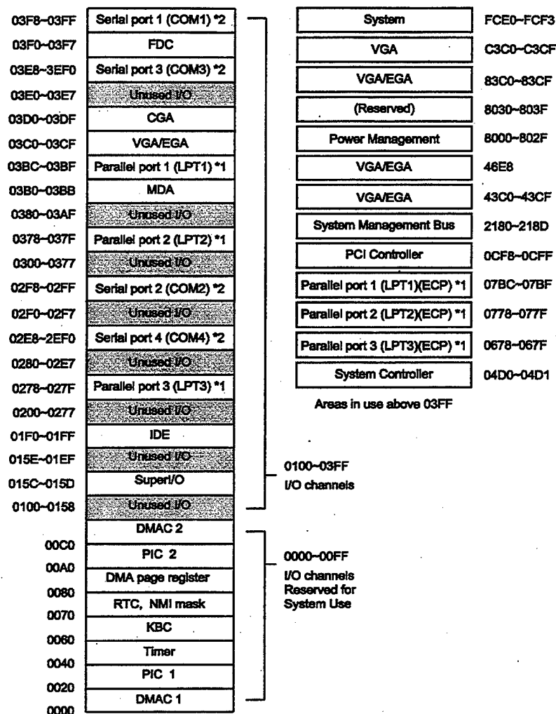
Figure 22. CardPC I/O Map [Ref. 25]
