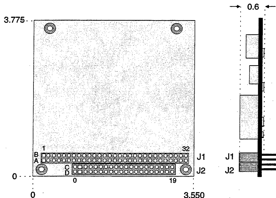
Figure 6. Basic Mechanical Dimensions, 16-bit PC/104 Module [Ref. 16].
