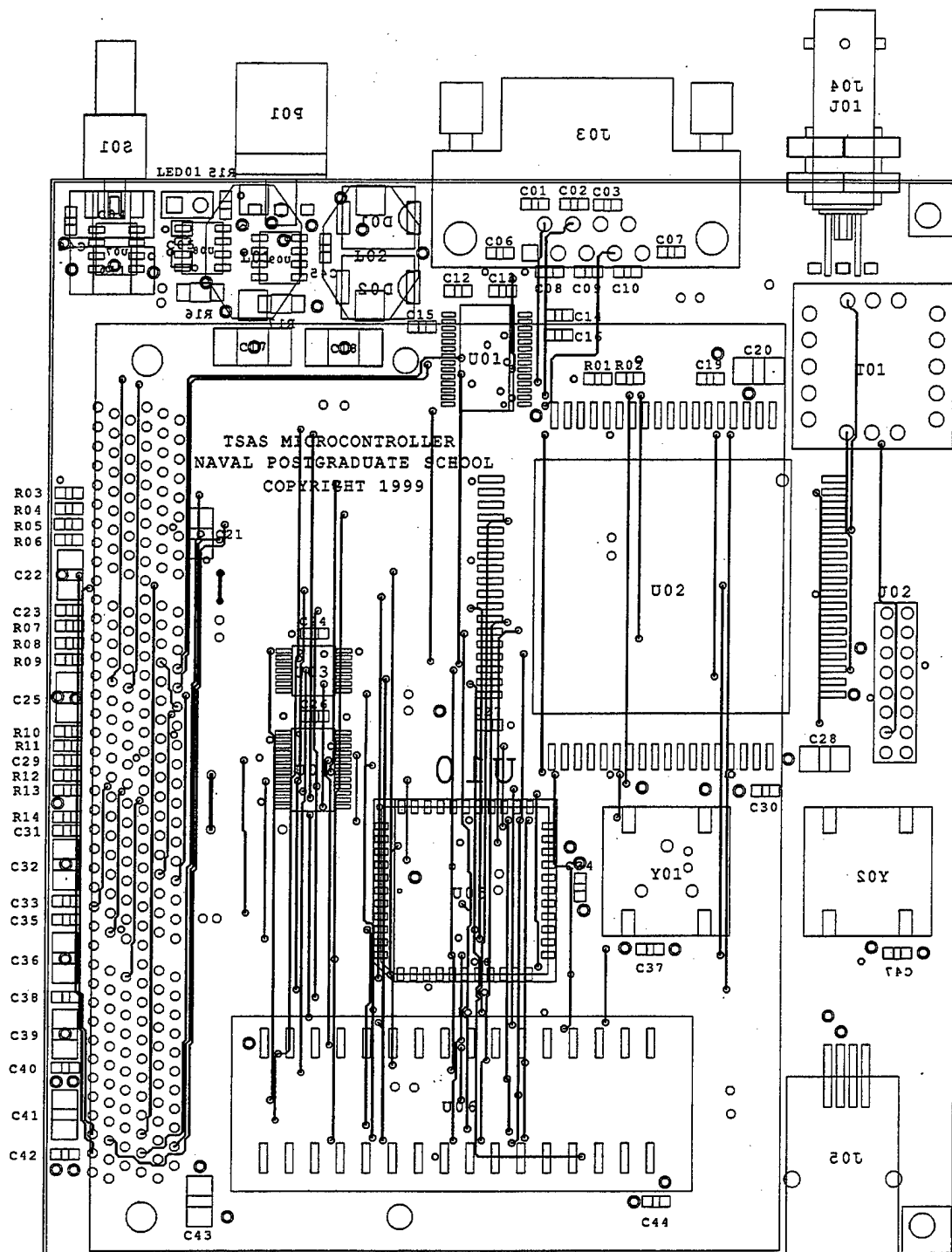
Figure 51. TSAS Microcontroller, Showing S2 Signal Layer Etch
