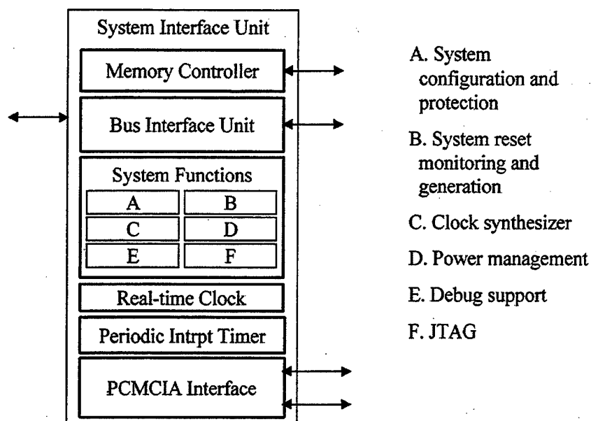
Figure 34. System Interface Unit Block Diagram [Ref. 68]
