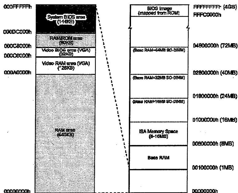
Figure 21. CardPC Memory Map [Ref. 25]
