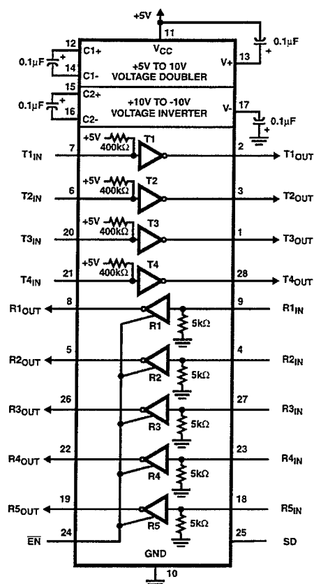
Figure 18. Harris HIN211 Internal Circuit Overview [Ref. 43]
