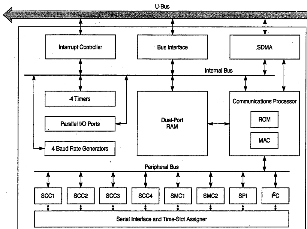
Figure 35. Communications Processor Module Block Diagram [Ref. 20]
