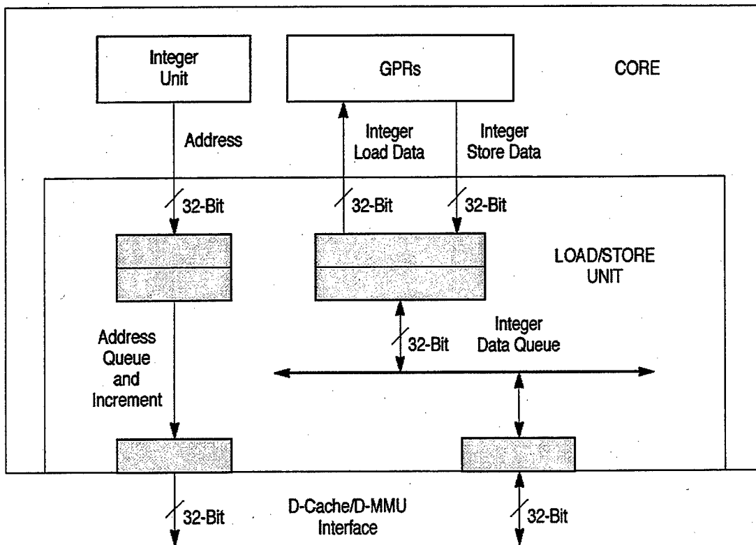
Figure 29. LSU Functional Block Diagram [Ref. 20]
