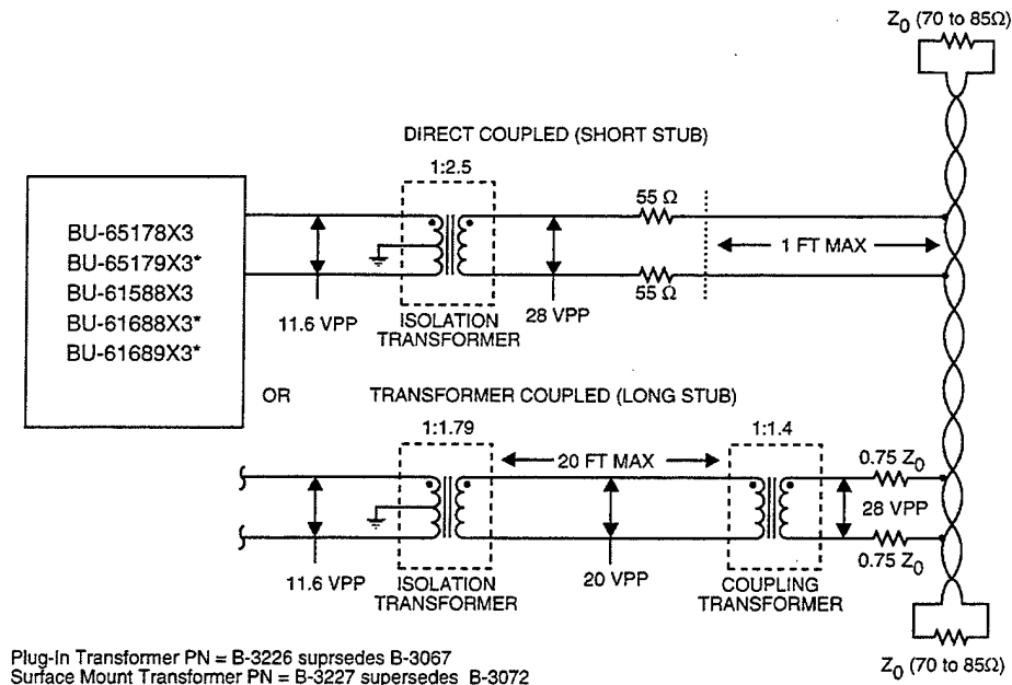
Figure 16. BU-61588/65178 Interface to 1553 Bus [Ref. 31]
