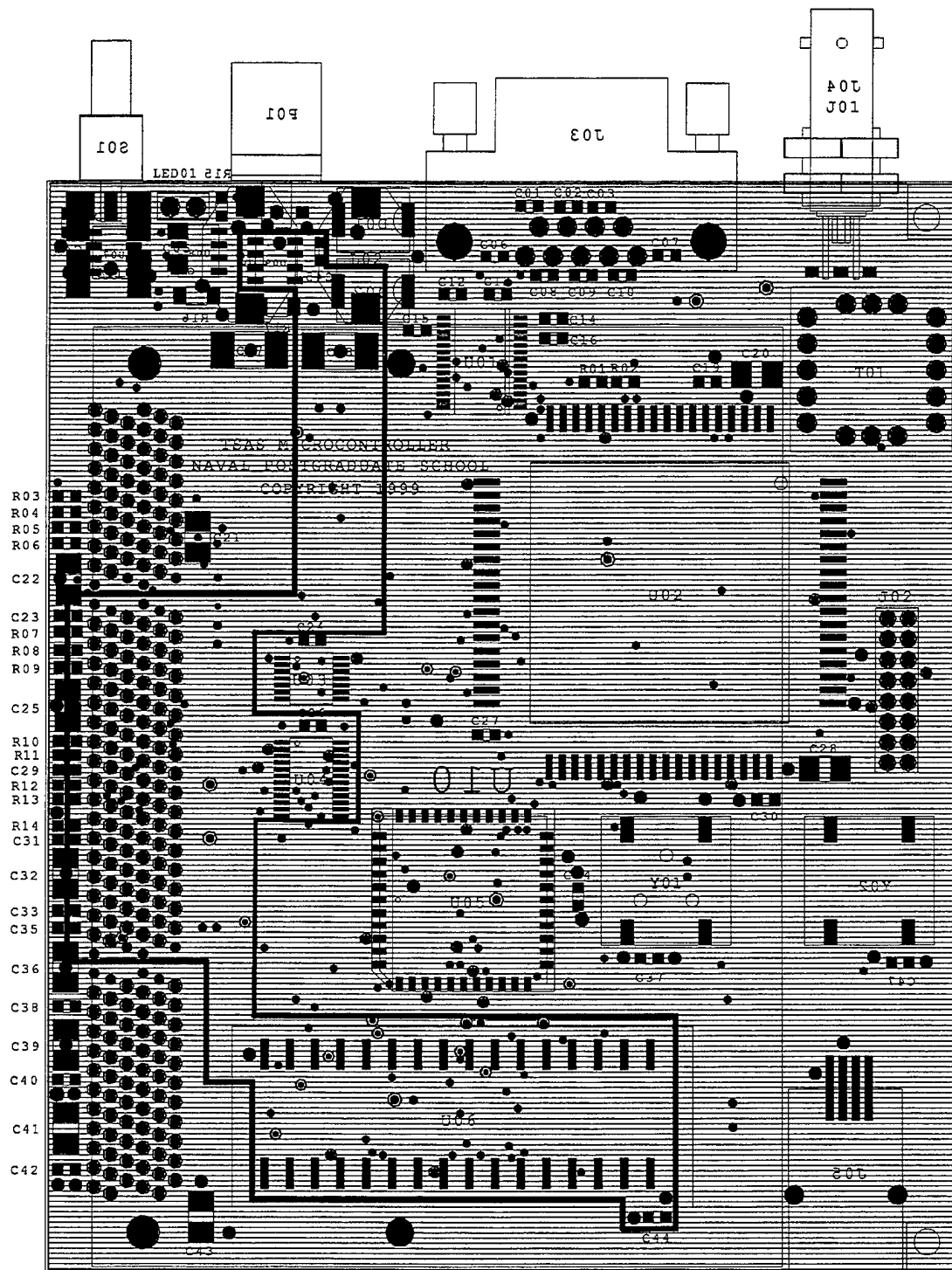
Figure 62. TSAS Microcontroller VCC3 and VCC5 Planes Layout
