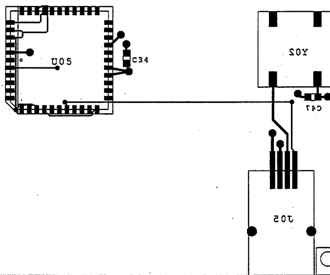
Figure 56. TIC Interface Component Layout
