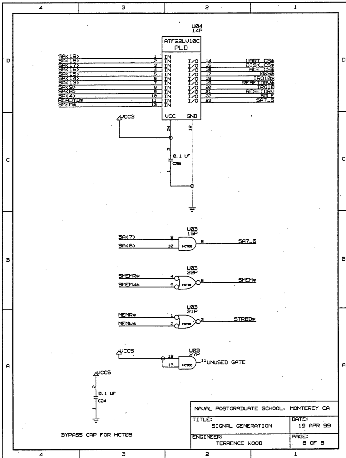
Figure 44. Signal Generation Circuit Schematic
