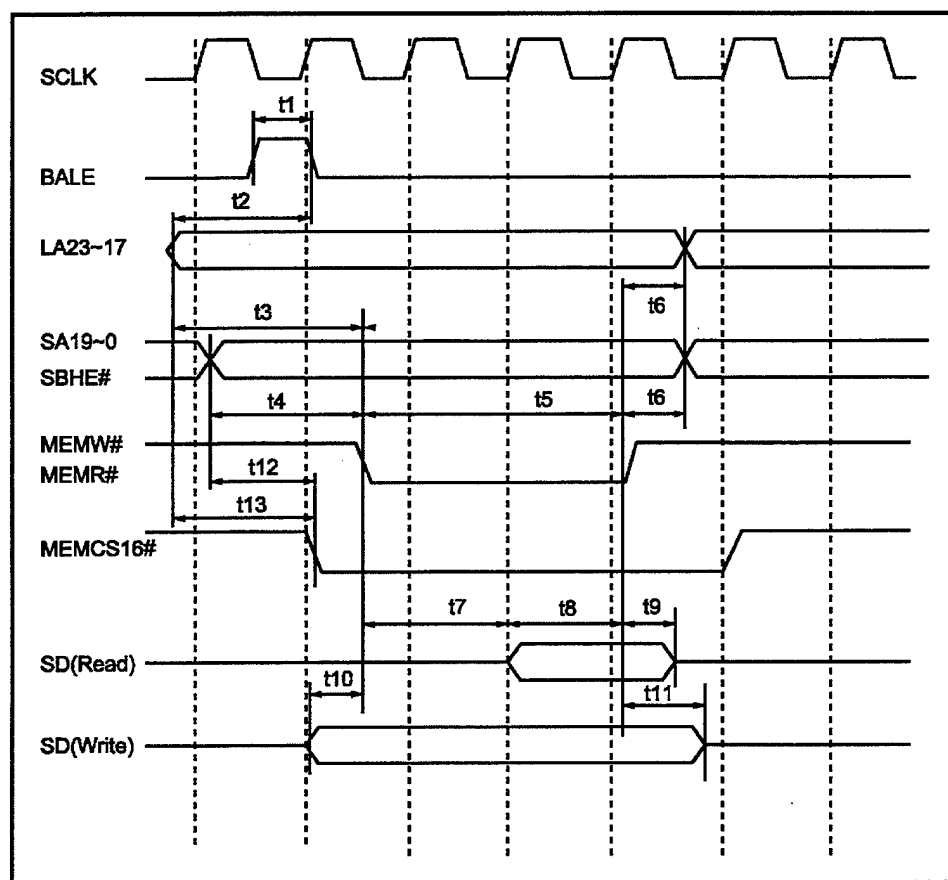
Figure 17. CardPC ISA Bus 16-bit Memory Read/Write Cycle [Ref. 25]
