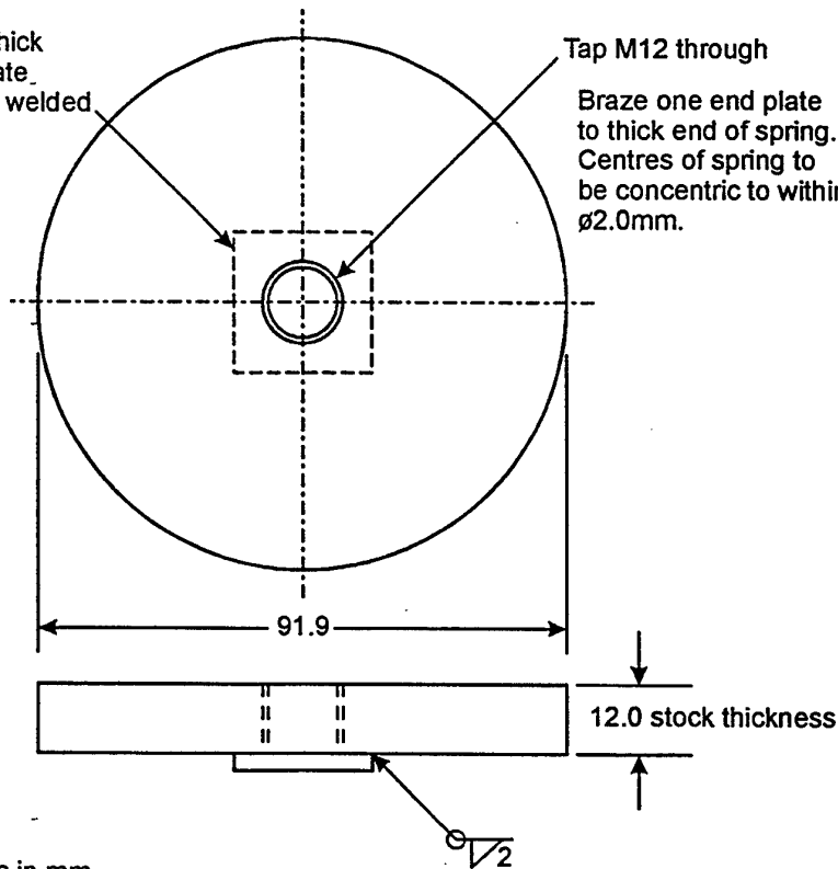
Figure A2 Steel Components of waveguide vibration isolator.
