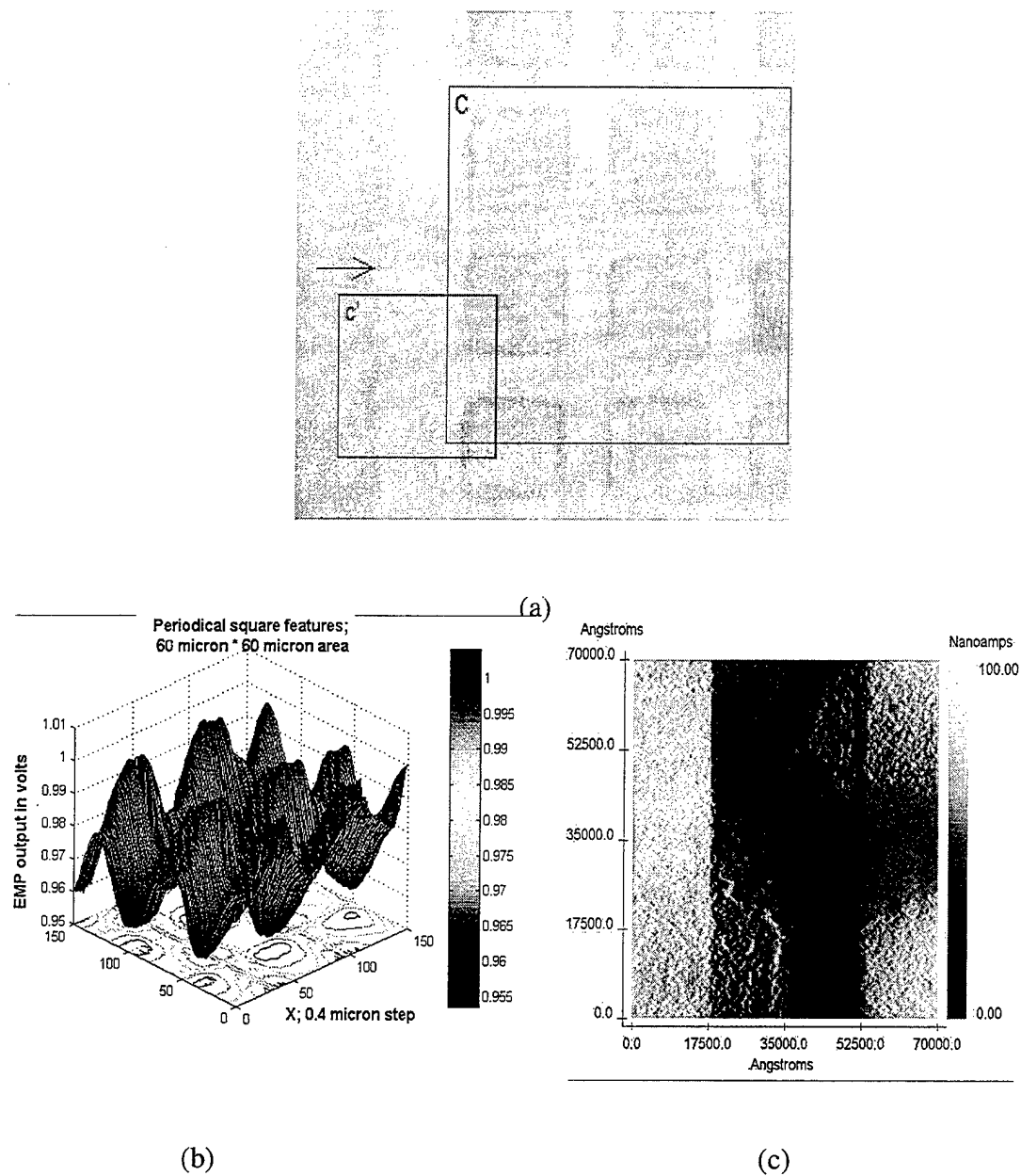
Figure 19 The optical image (a) and the EMP image (b) of a 10 \mu m square features (Area C in Figure 16). The STM image (c) shows the roundness at corners of those squares (Area c' in Figure 16).
