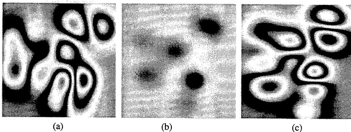
Figure 1.3. Synthetic shearograms obtained from a complex of simulated debonds. (a) X-axis shearogram; (b) curvature image calculated from the input displacement; (c) Y-axis shearogram
