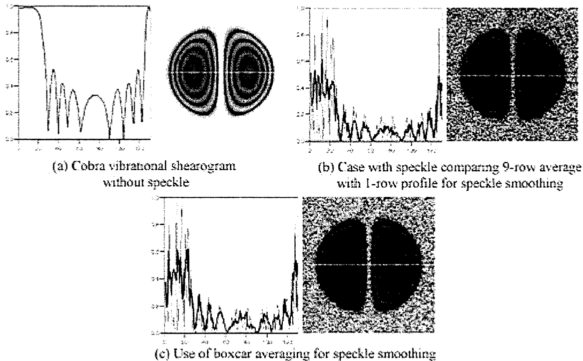
Figure 2.14. Illustration of fringe modulation when vibrational excitation is used. (a) without speckle (b) 9-row average to smooth speckle; (c) boxcar averaging to smooth speckle
