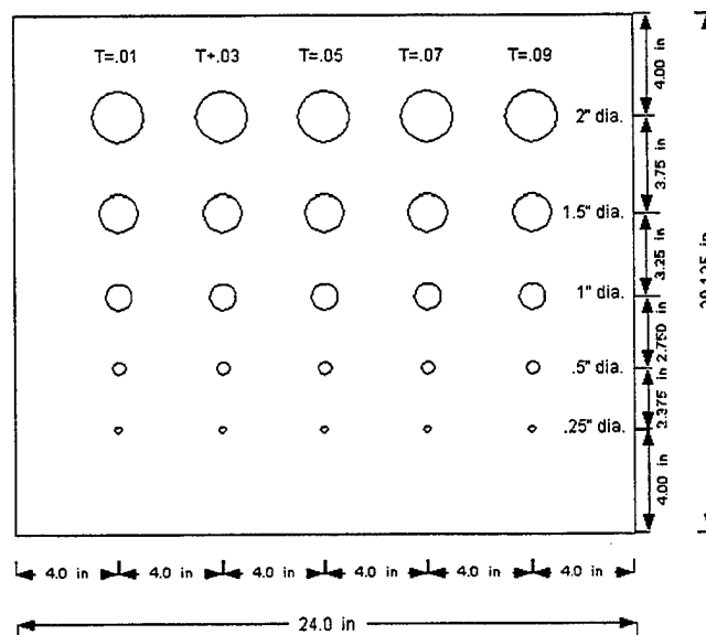
Figure 2.2. Schematic of Fast debond phantom
