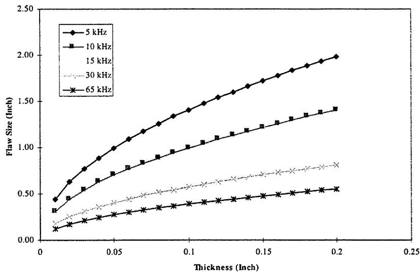
Figure A4. Required forcing frequency for target flaw size and thickness for graphite/epoxy composite
