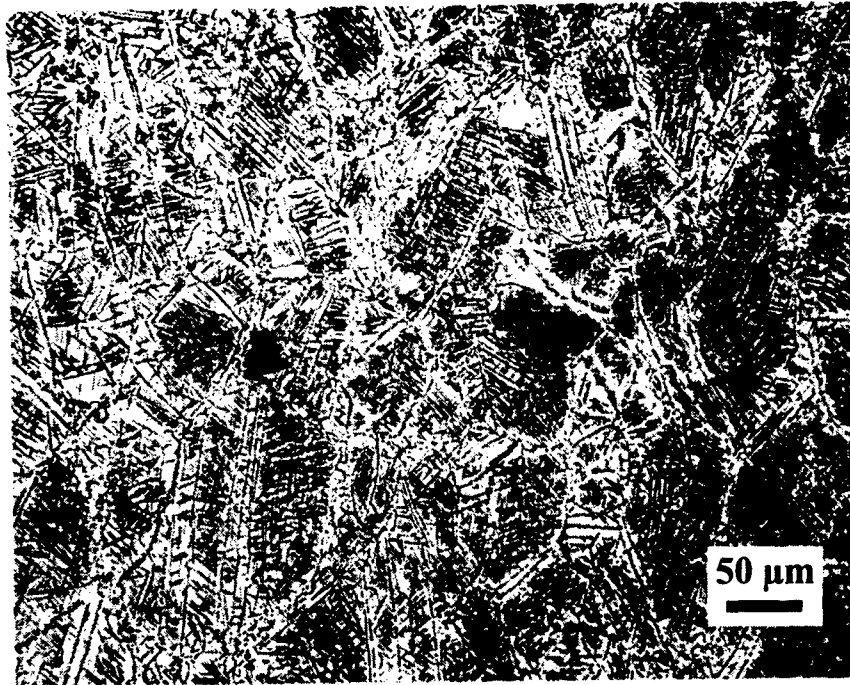
FIGURE 73a. MICROSTRUCTURE OF WROUGHT MATERIAL WITH LOW NIOBIUM AND BORON CONTENT AFTER 40 HEAT TREATMENT CYCLES
