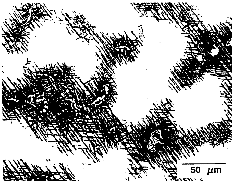
FIGURE 63a. CAST IN718 MICROSTRUCTURE FROM RETIRED CF6-6
