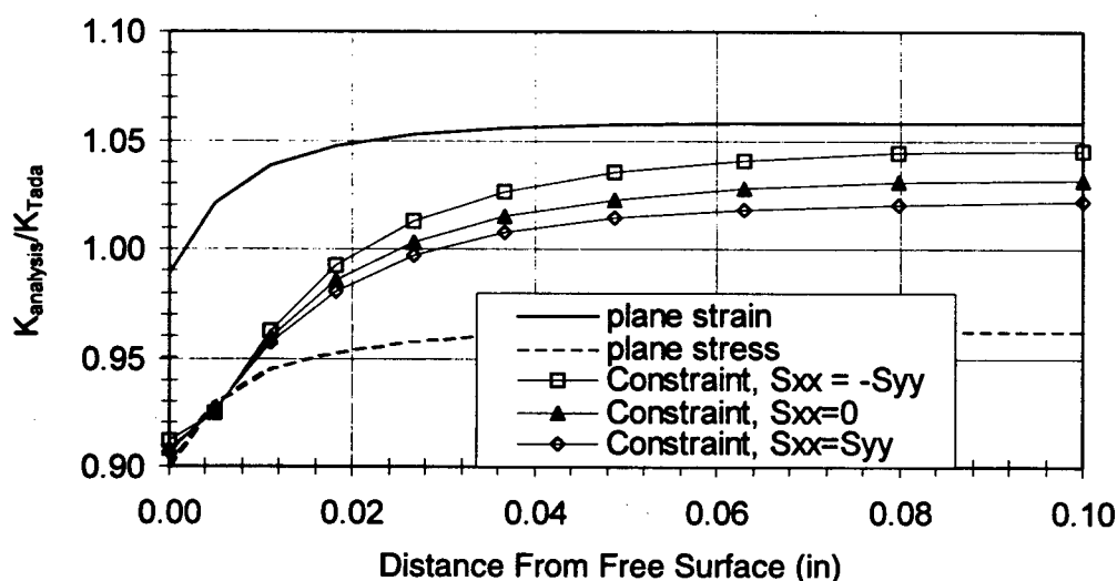
FIGURE 16. CENTER-CRACKED PANEL, 2a/W = 0.2 , B/W = 0.1
