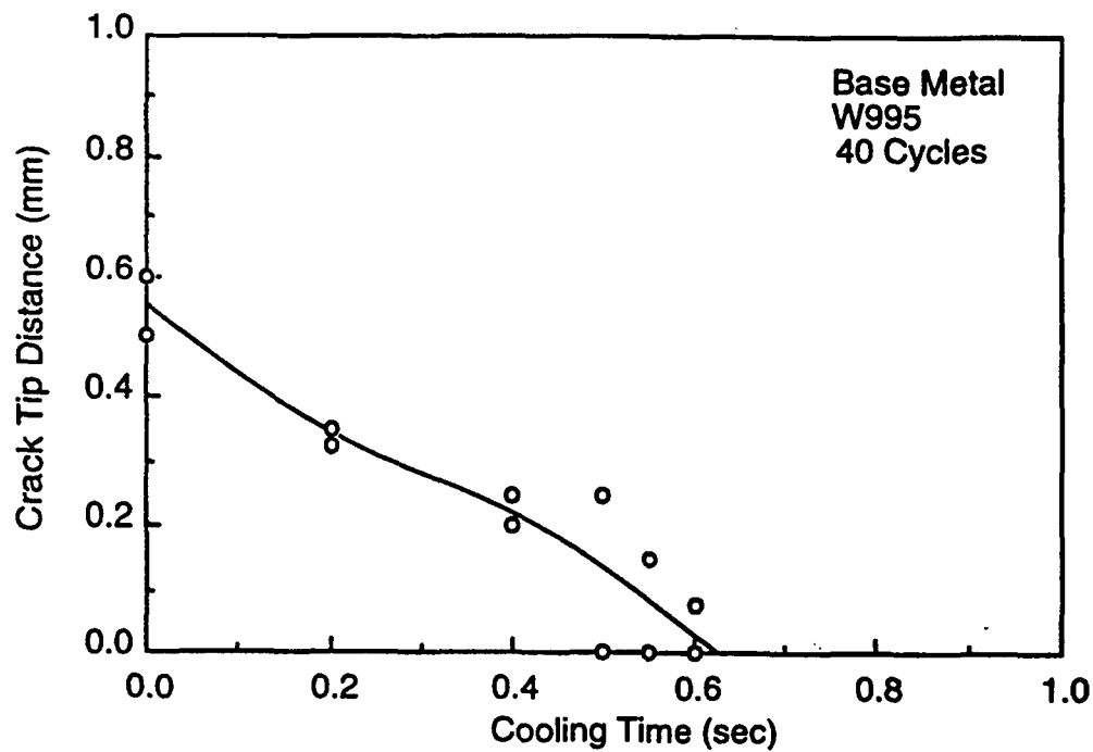
FIGURE 70a. SPOT VARESTRAINT DATA FOR MEDIUM COMPOSITION WROUGHT PROGRAM MATERIAL AFTER 40 HEAT TREATMENT CYCLES
