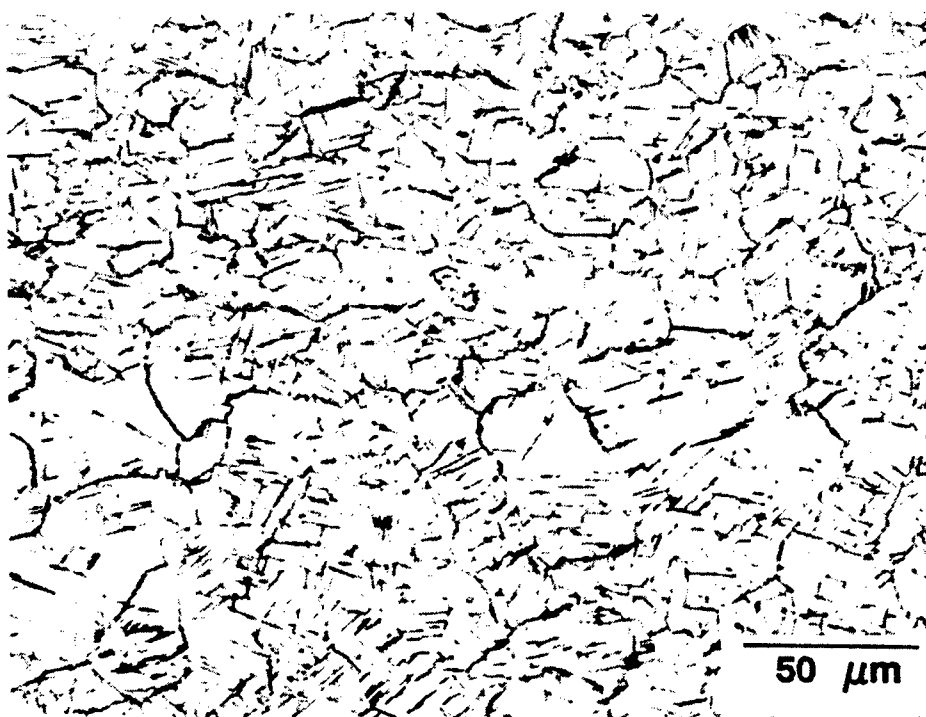
FIGURE 63b. WROUGHT IN718 MICROSTRUCTURE FROM RETIRED CF6-6
