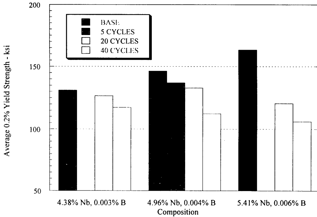
FIGURE 48. EFFECT OF MULTIPLE POSTREPAIR THERMAL CYCLES ON CAST+HIP IN718 0.2% YIELD STRENGTH
