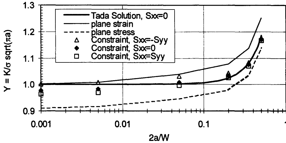
FIGURE 18. WEIGHTED AVERAGE K MULTIAXIAL APPLIED LOAD, B/W = 0.2
