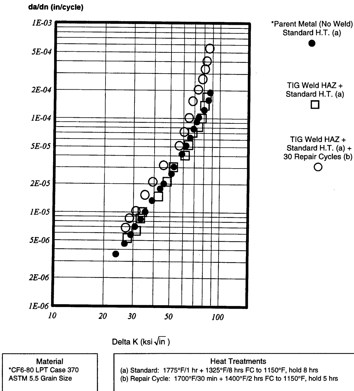
FIGURE 29. EFFECT OF MULTIPLE REPAIR (1700°F) CYCLES ON WROUGHT IN718 WELD HEAT AFFECTED ZONE REGIONS II AND III CRACK GROWTH 800°F, R = 0.05, FREQUENCY = 0.33 Hz
