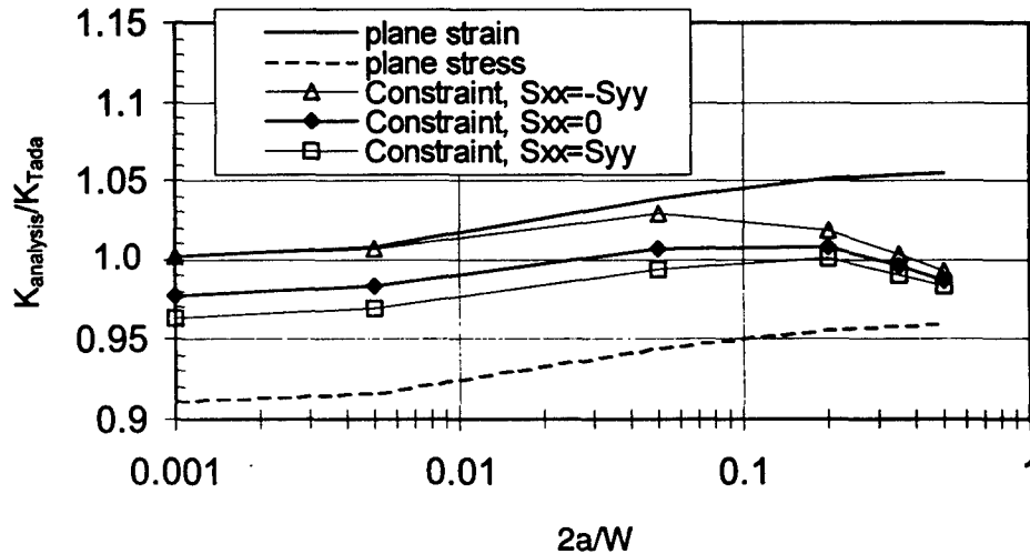
FIGURE 19. WEIGHTED AVERAGE K MULTIAXIAL APPLIED LOAD, B/W = 0.2
