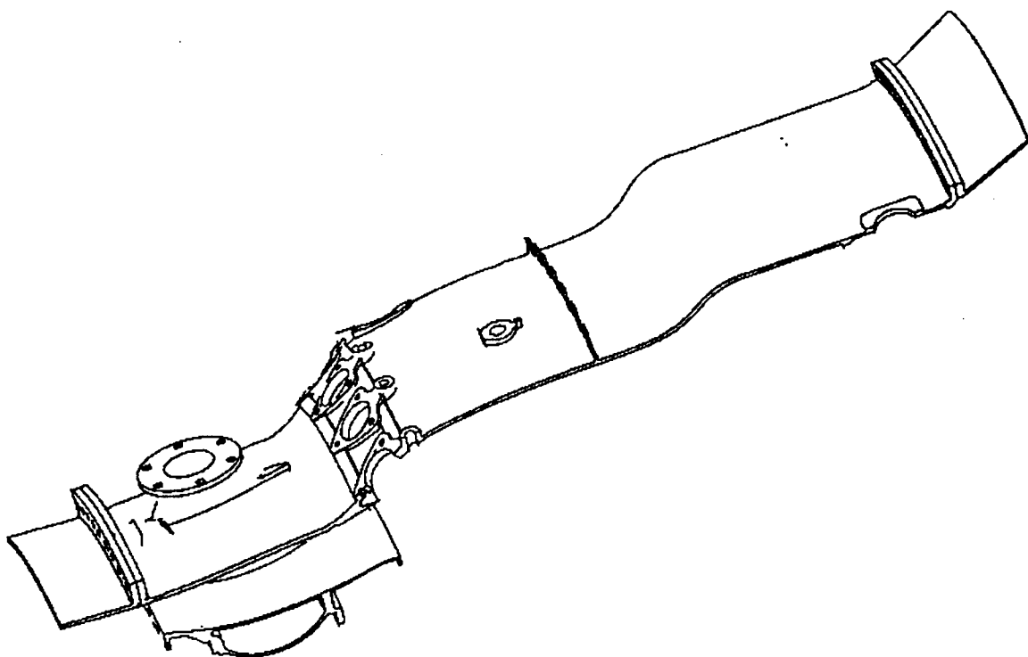
FIGURE 6. CF6-50 UNIGRAPHIC MODEL
