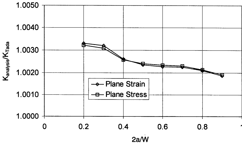
FIGURE 11. TWO-DIMENSIONAL CENTER-CRACKED PANEL
