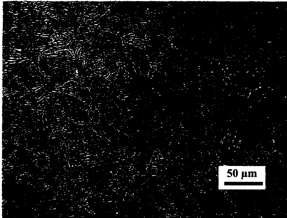
FIGURE 66a. MICROSTRUCTURE OF MEDIUM COMPOSITION WROUGHT PROGRAM MATERIAL IN THE AS-RECEIVED CONDITION
