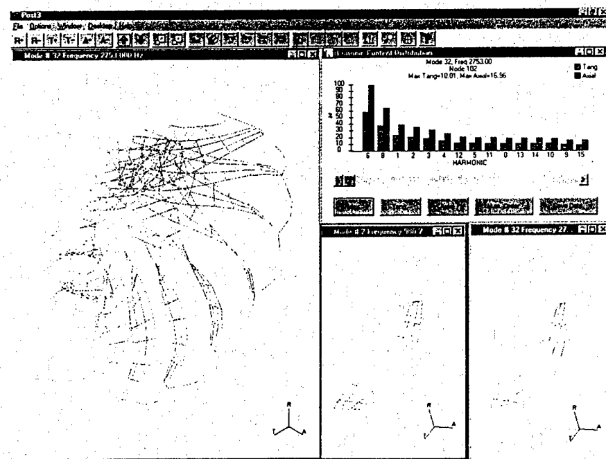
A Modal post-processing allows the user to view multiple animated mode shapes, and determine the harmonic content of any mode.
