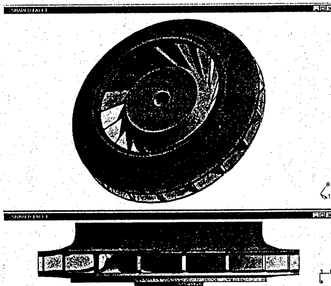
A Example of shrouded impeller. (Courtesy of Demag Delaval)
