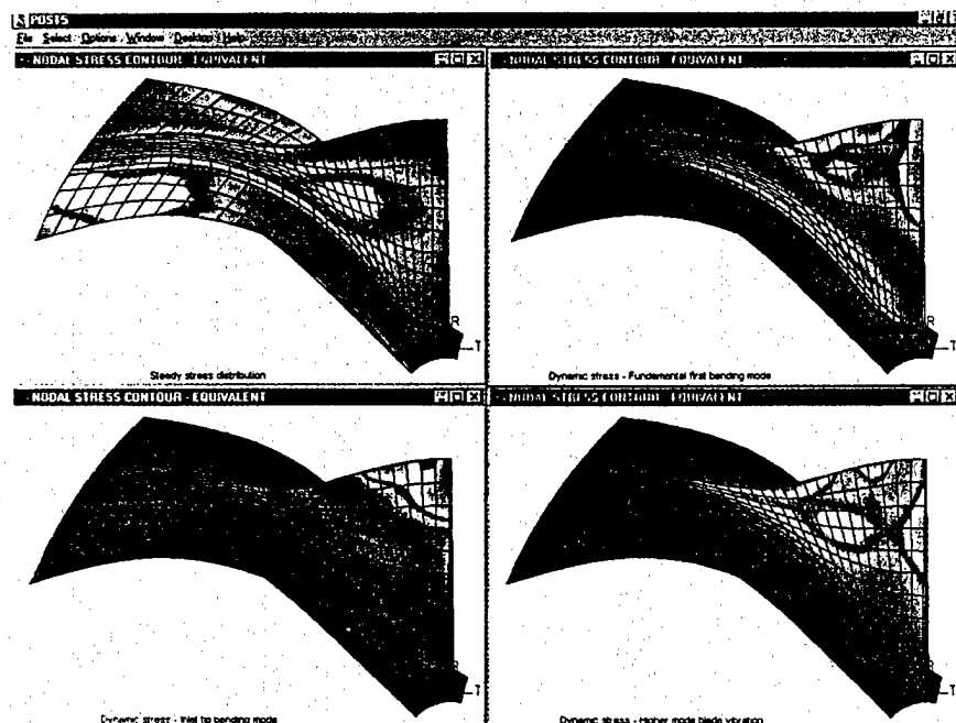
A IMPRO can calculate both steady and vibratory stresses.
