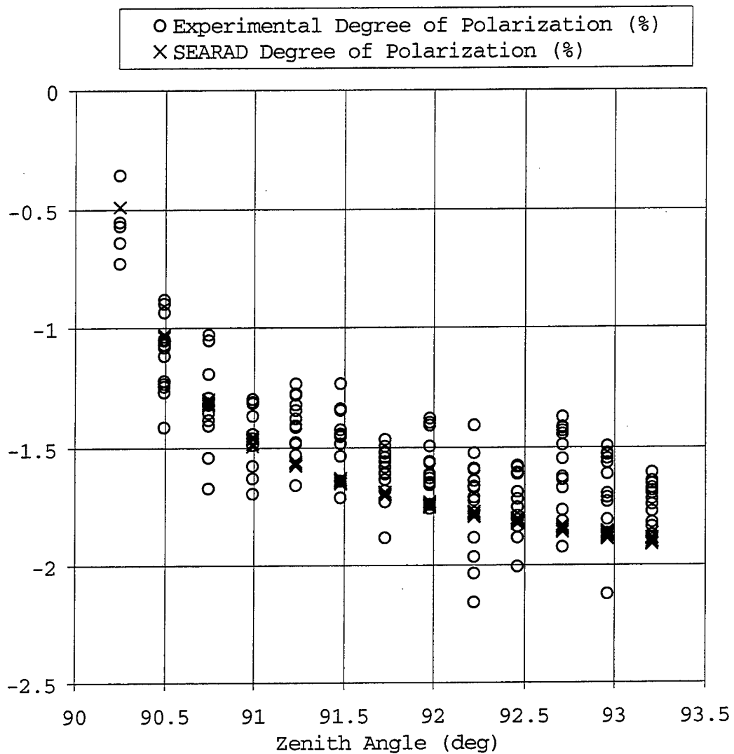
Figure 5.4 Comparison of the SEARAD and Experimental Degrees of Polarization Different Values of Polarization for the Same Zenith Angle Correspond to Different Azimuth Angles.
