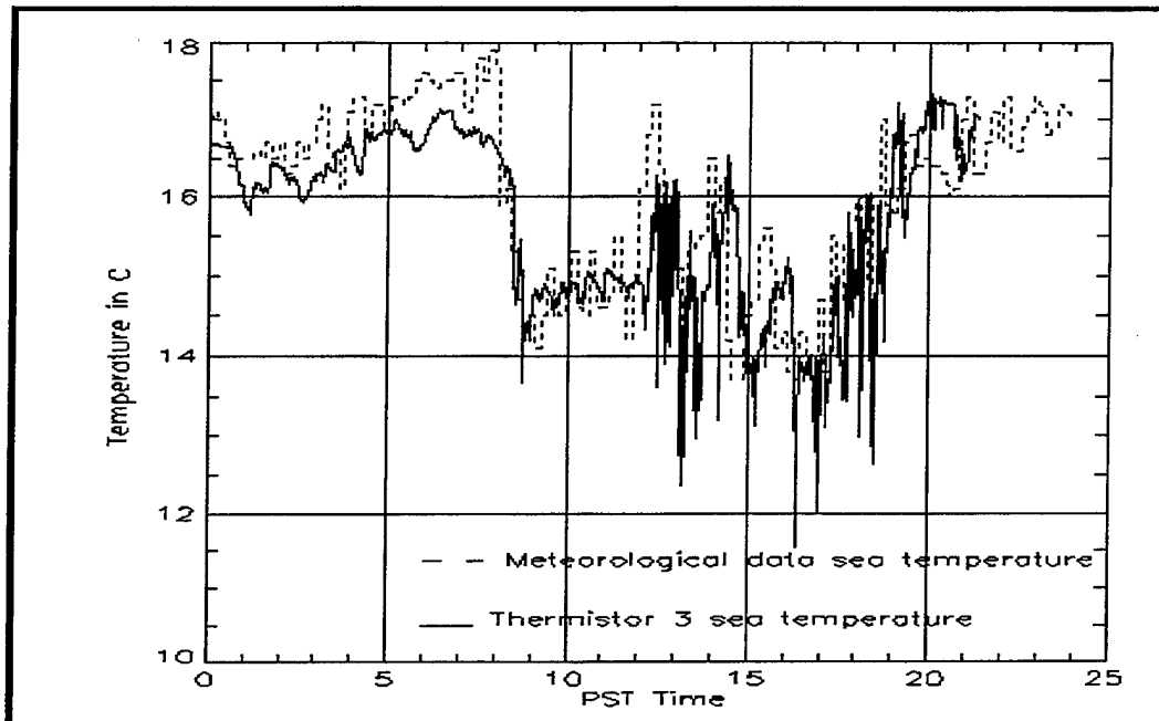
Figure 4.6 Comparison of the Meteorological Data Sea Temperature and Thermistor 3 Sea Temperature, to Clarify in which Time Zone were the “Skin “ Data Recorded
