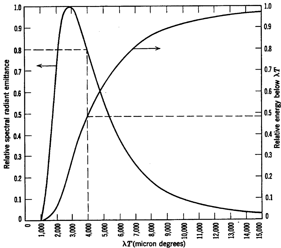
Figure 2.3 Universal Blackbody Curve [Ref. 9]
