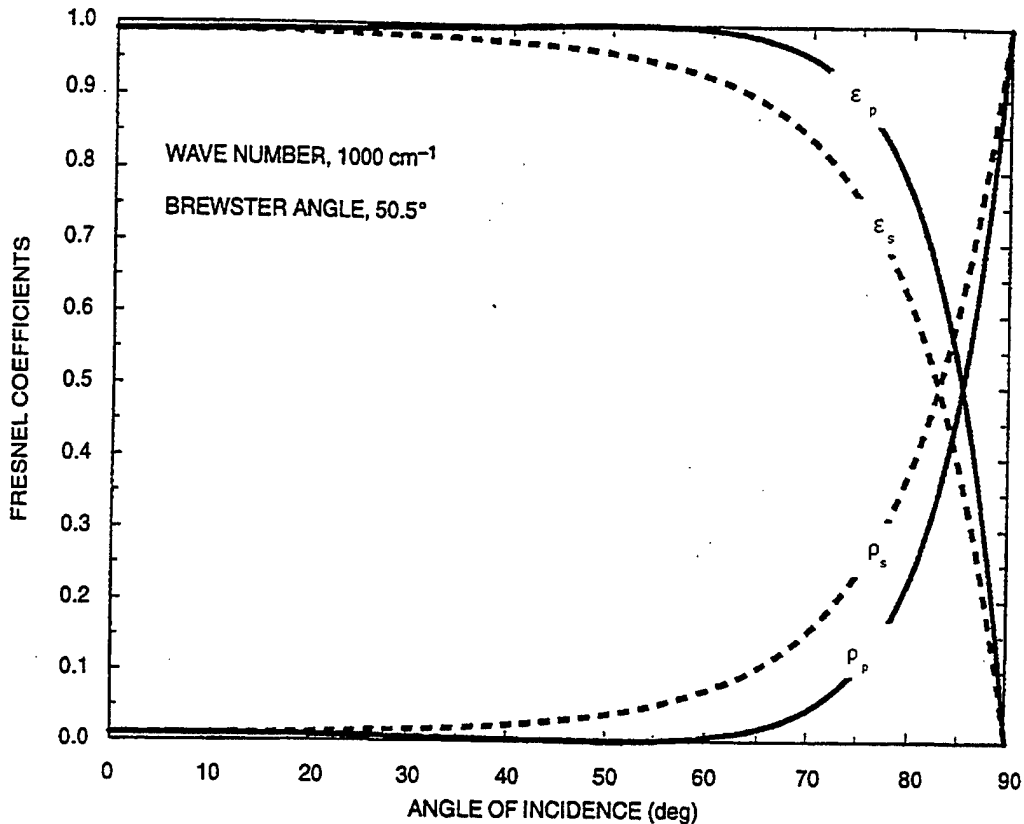
Figure 3.3 Sea Water Emissivities and Reflectances for a Wavelength of 10 \mu\text{m} ; s Refers to the Component Perpendicular to the Plane of Incidence, and p to the Component Parallel to the Plane of Incidence [Ref. 8].
