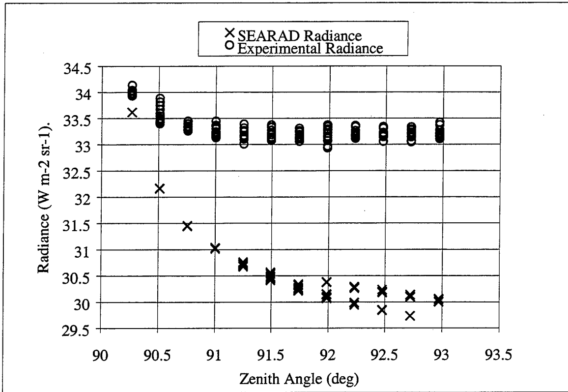
Figure G1.5 Experimental and SEARAD Sea Radiance as a Function of the Zenith Angle. Different Values of Radiance for the Same Zenith Angle Correspond to Different Azimuth Angles. The Ship Camera Slant Range is 2704 m. The Average Absolute Error is 2.56 \text{ Wm}^{-2}\text{sr}^{-1} and the Standard Deviation is 0.73 \text{ Wm}^{-2}\text{sr}^{-1}
