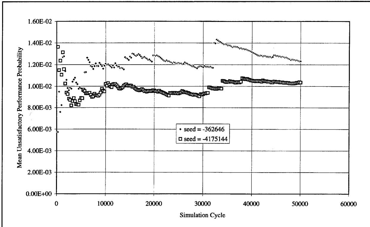
Figure 5. IS with SF_t = 1.50
