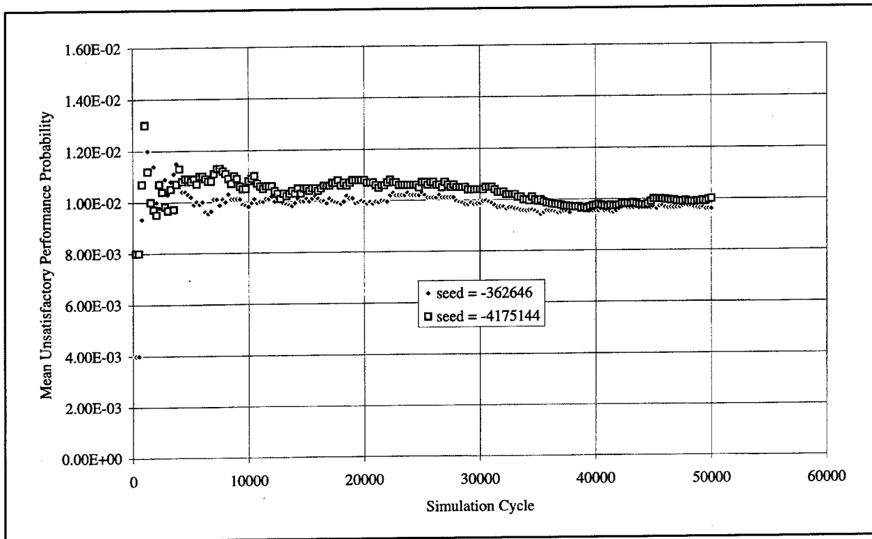
Figure 6. Direct MCS with SF_t = 1.82545
