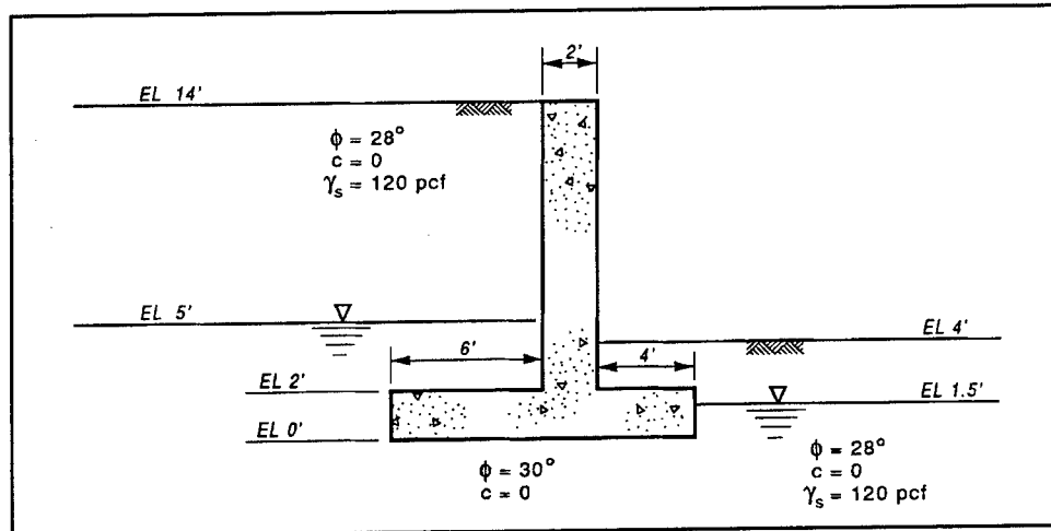
Figure 3. Retaining wall
