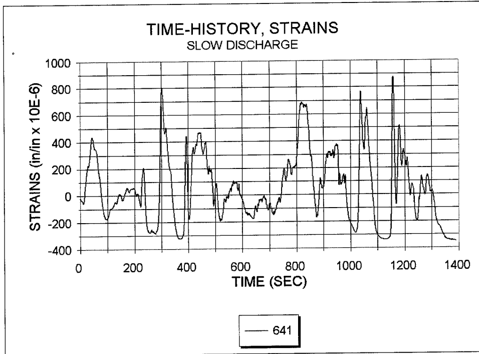
Figure 9. Strain time-history, Experiment 1 (Transducer 641)
