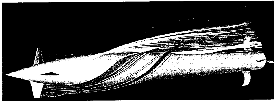
c. Particle traces for Mach 1.6, 10^\circ angle of attack.
