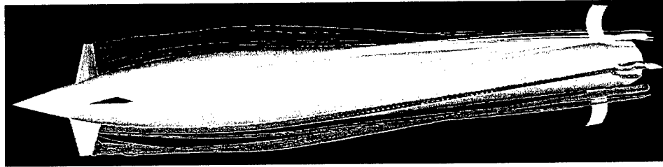
a. Particle traces for Mach 1.6, 0^\circ angle of attack.
