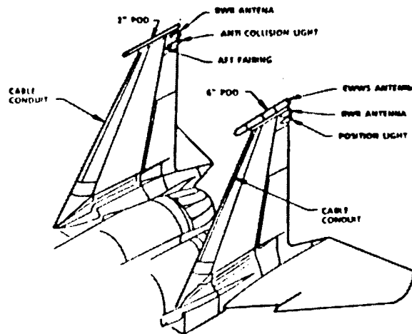
Figure 1.2. F-15 Vertical Tail Configuration
