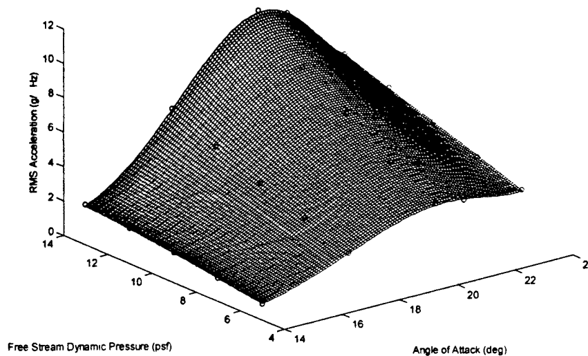
Figure 11.8. Envelope of Root Mean Square of the Trailing Edge Tip Acceleration versus Angle of Attack and Free Stream Dynamic Pressure (o: Experimental Data Points).
