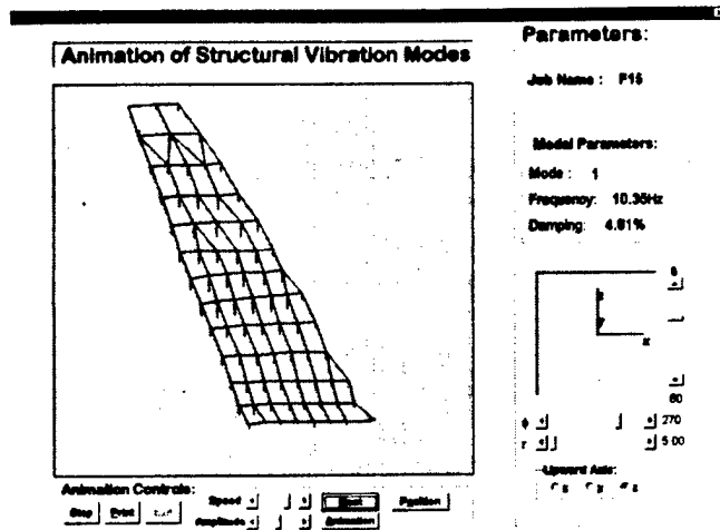
Figure 5.13 Mode 1, vector display, x-direction
