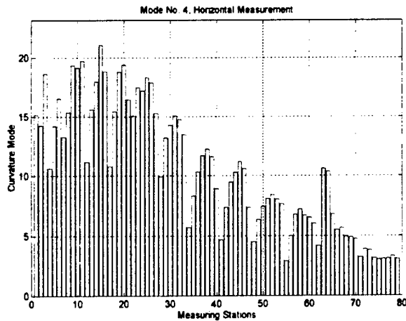
Figure 5.20 Mode 4, bar plot, x-direction
