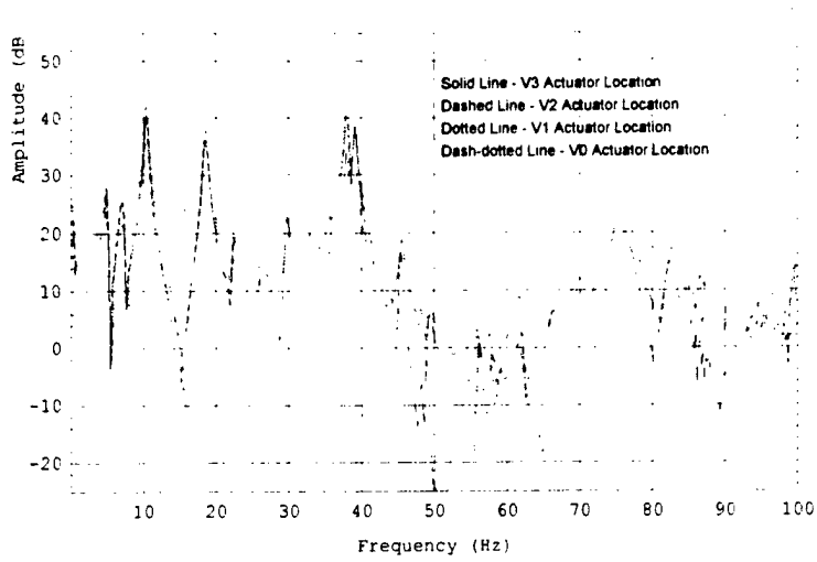
Figure 5.20 Refined modal survey, z-direction
