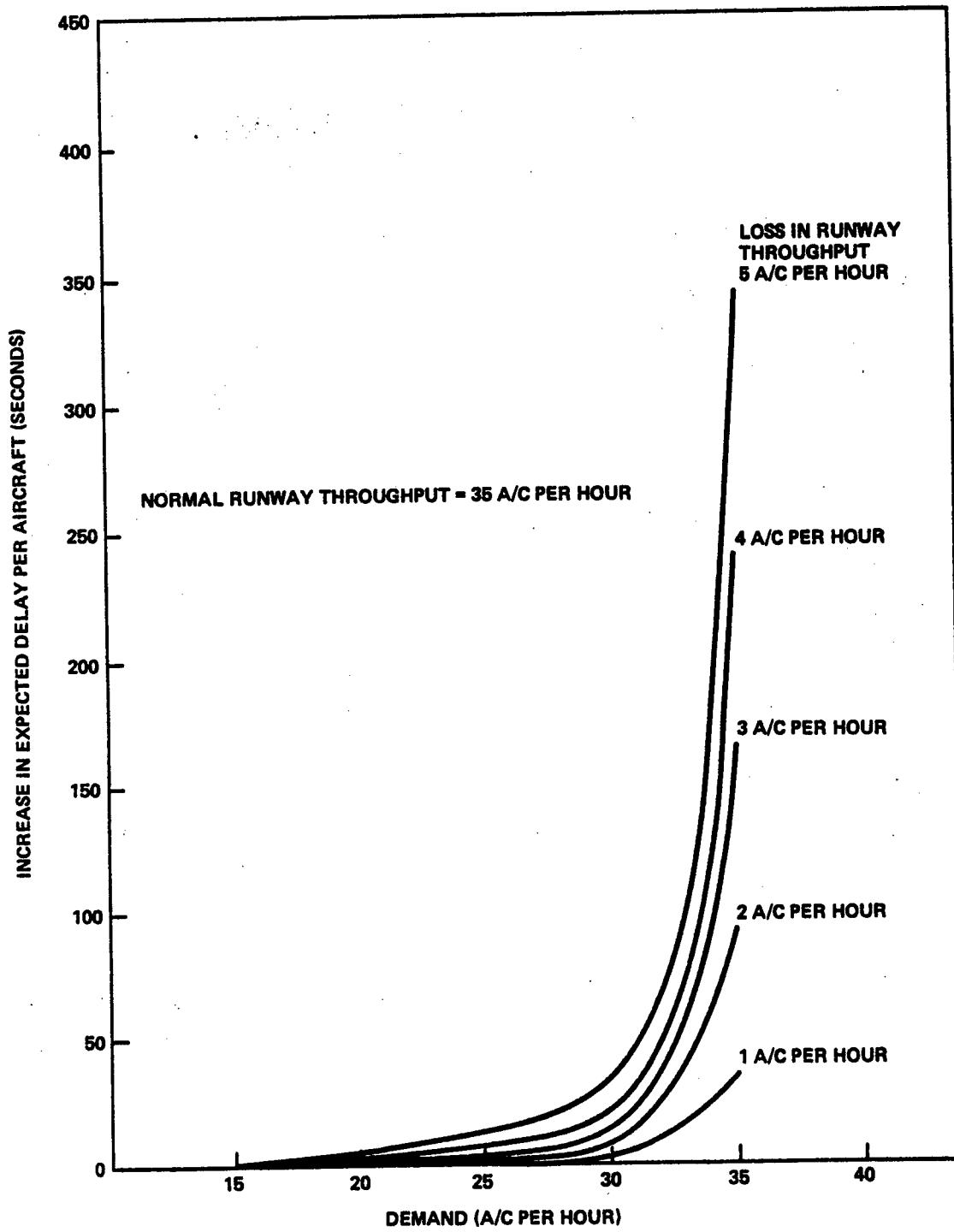
INCREASE IN TIME DELAY (ABOVE AVERAGE DELAYS) DUE TO A LOSS IN RUNWAY THROUGHPUT AS A FUNCTION OF DEMAND (FOR ARRIVALS ONLY)
