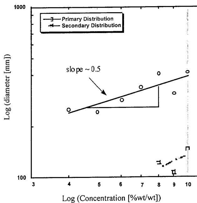
Figure 9. Average Fiber Diameter as a Function of PEO Concentration.
