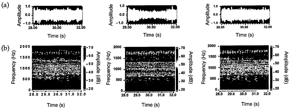
Figure 17. (a) Time-series data and (b) spectrograms for vehicle passing open offices with noise and speech.
