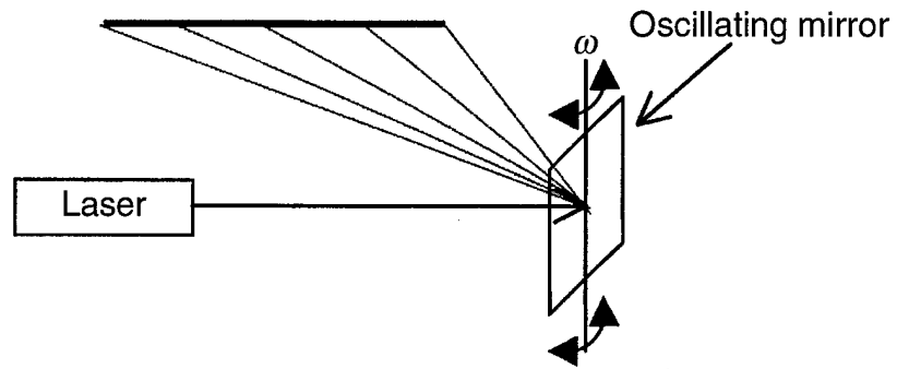
Figure 5. Line illumination raster scan pattern.
