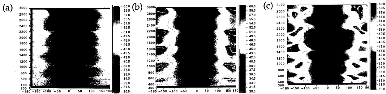
Figure 13. Polar and Cartesian directivity curves from density plots (a) microphone only, (b) single microphone with plastic tubes, and (c) array with plastic tubes.
