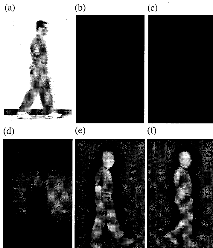
Figure 22. CCD and FLIR images of humans at 19 ft (CCD) and 14 ft (FLIR): (a) CCD with lights, (b) CCD without lights, (c) CCD with IR illuminator, IR filter removed; (d) CCD with IR illuminator, without filter, 95 percent increase in contrast via software; (e) FLIR with lights; and (f) FLIR without lights.
