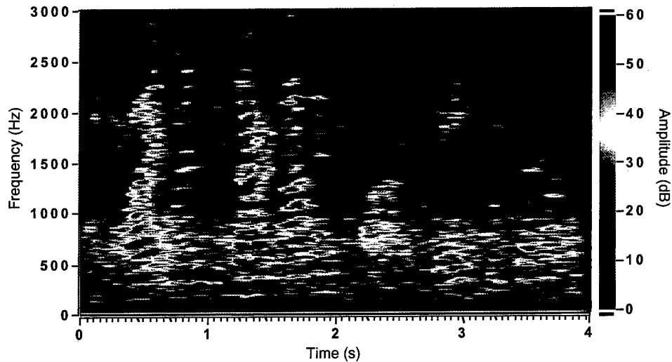
Figure 18. High-SNR speech: time (s) vs frequency (Hz) and amplitude (dB).
