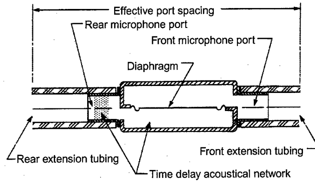
Figure 9. A bidirectional microphone schematic and photograph of Knowles and B&K microphones.
