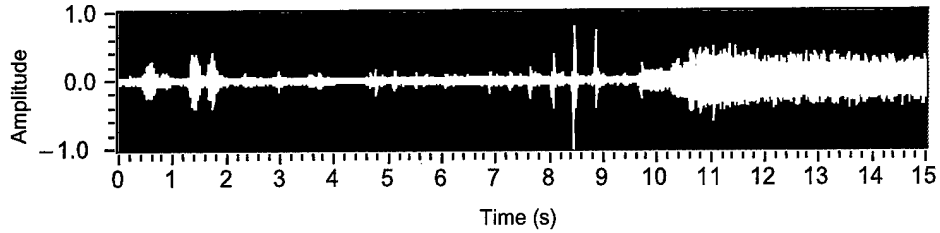
Figure 15. Time series: talking, footfalls, and engine.
