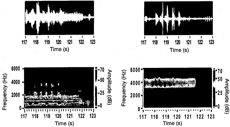
Figure 16. Spectrogram: time vs frequency and amplitude.
