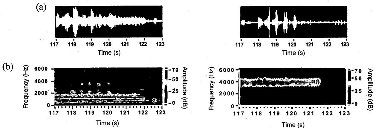
Figure 20. (a) Time-series data and (b) spectrograms for vehicle noise and data, unfiltered and band-rejected.
