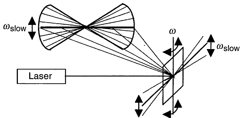
Figure 6. Bow-tie illumination raster scan pattern.
