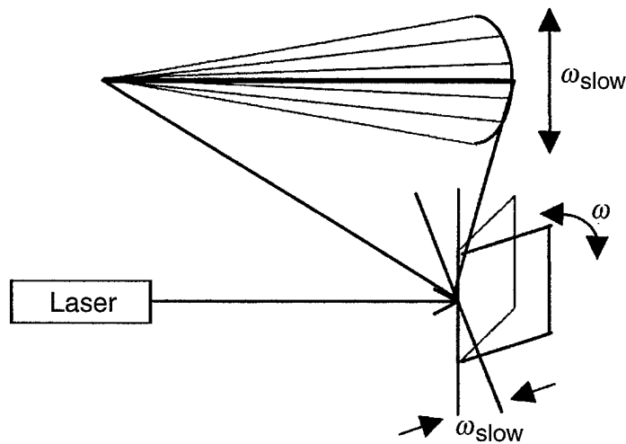
Figure 7. Wiper illumination raster scan pattern.
