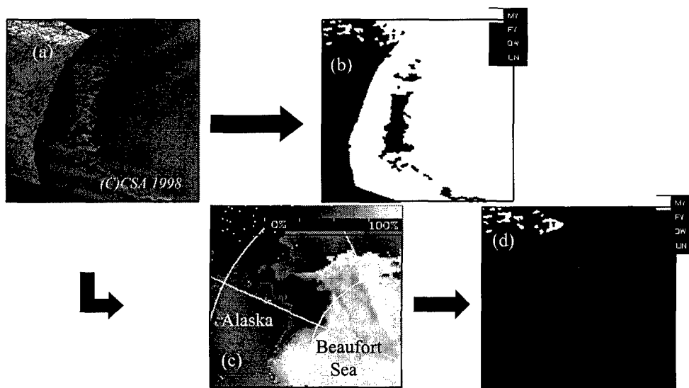
Figure 2. Improvements gained through addition of SSM/I ice concentration data. (a) Radarsat image near Point Hope, Alaska. (b) ARKTOS classification map (without SSM/I), incorrectly classifying water as MY ice (c) SSM/I (d) After incorporation of SSM/I, ARKTOS classification with water correctly classified.
