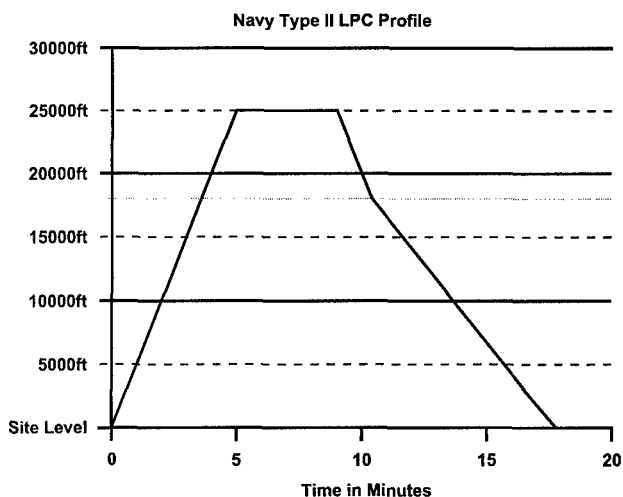
Type II 25K' Initial, 30 min pressure breathing at site level
