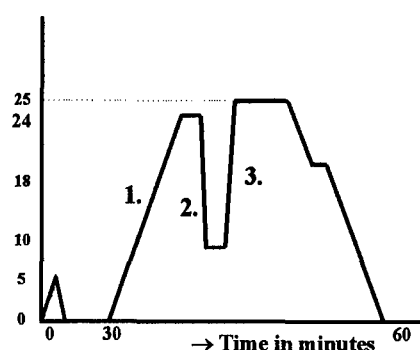
Fig. 8: HAHO/HALO chamber flight-profile
