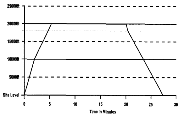
Type III 20K' Non-pressure breathing Navy Type III LPC Profile
