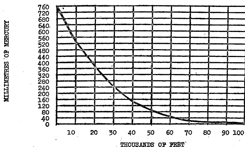
FIGURE 1.—Altitude-pressure curve.
