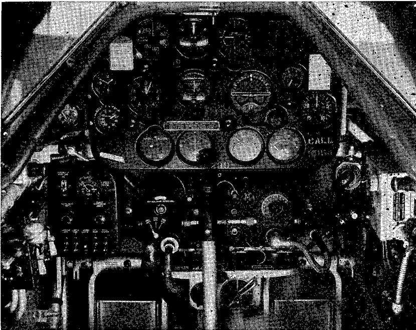
FIGURE 2.—Instrument board equipped for blind flying.
