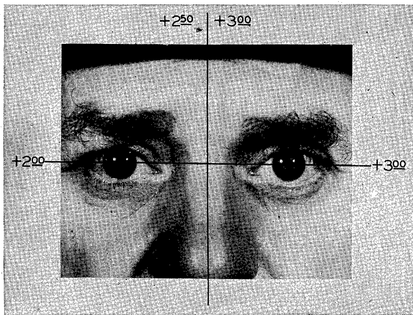
FIGURE 47.—Retinoscopic findings.
