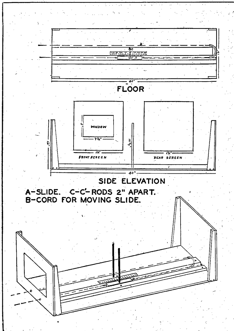
FIGURE 9.—Depth perception apparatus.
