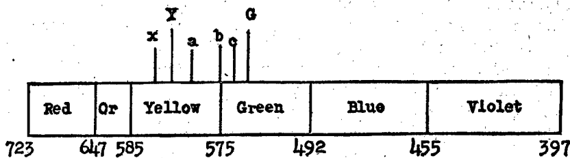
FIGURE 28.—Spectrum.
