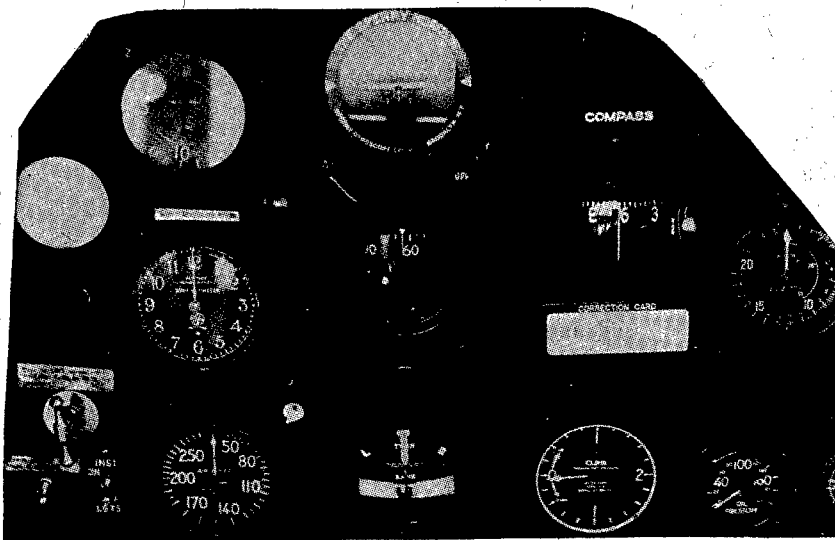
FIGURE 5.—Instrument board of blind flying ship.
