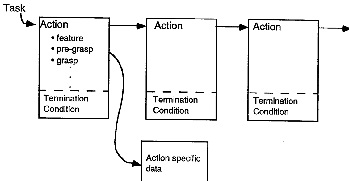
Figure 10. Task Data Structure
